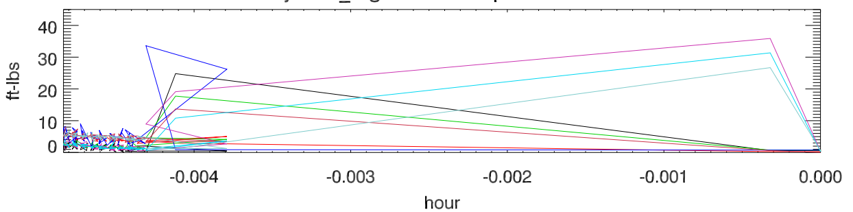
18jun13_2 gr motor torques at failure
