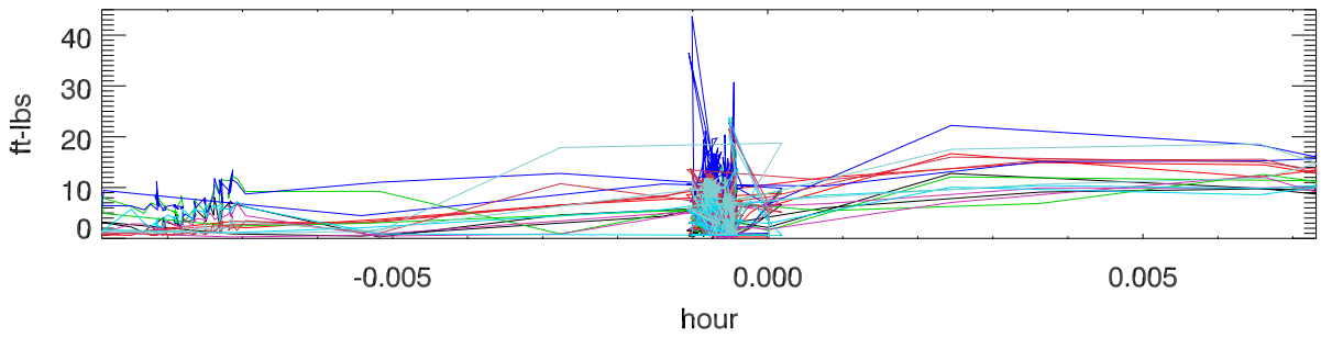
16jun13 gr motor torques at failure
