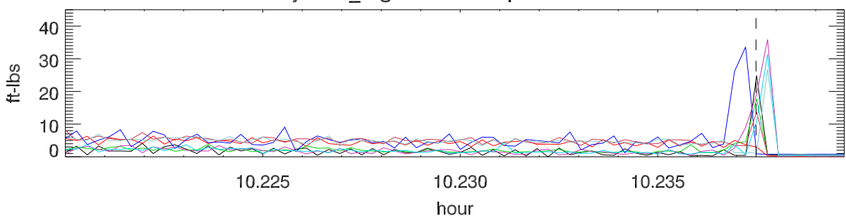
18jun13_2 gr motor torques at failure
