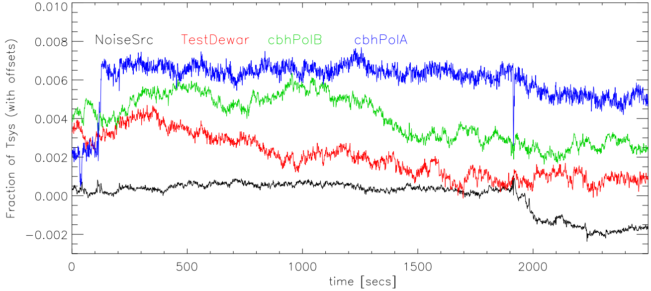
01aug06 mmic amplifier noise test Allen Deviation
