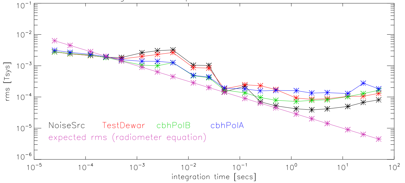
01aug06 acf of (tp[i]-tp[i+1]) . 25 usecs resolution
