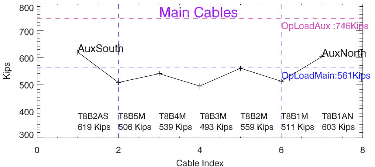
Tower 8 Backstay Average cable tensions
