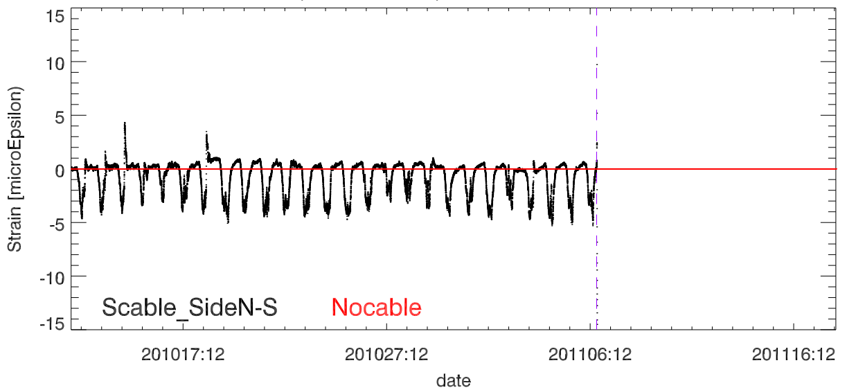
StrainDif (Side1 - Side2) vs date. Platform Tower 4
