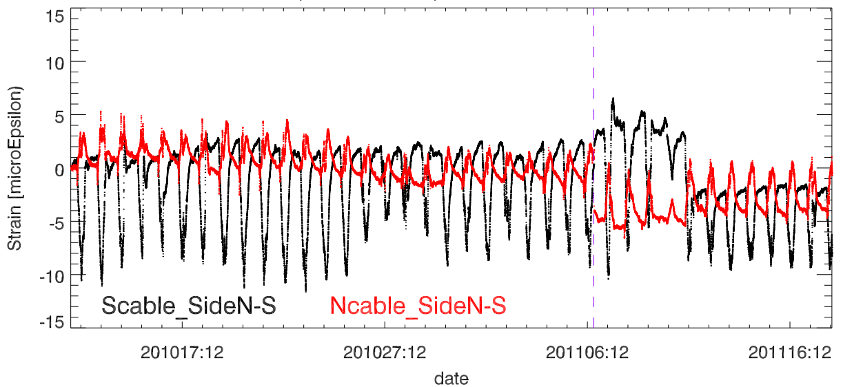
StrainDif (Side1 - Side2) vs date. Platform Tower 8
