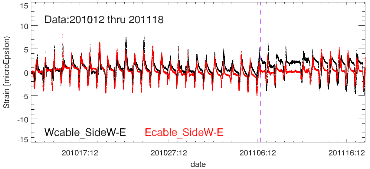
StrainDif (Side1 - Side2) vs date. Platform Tower 12
