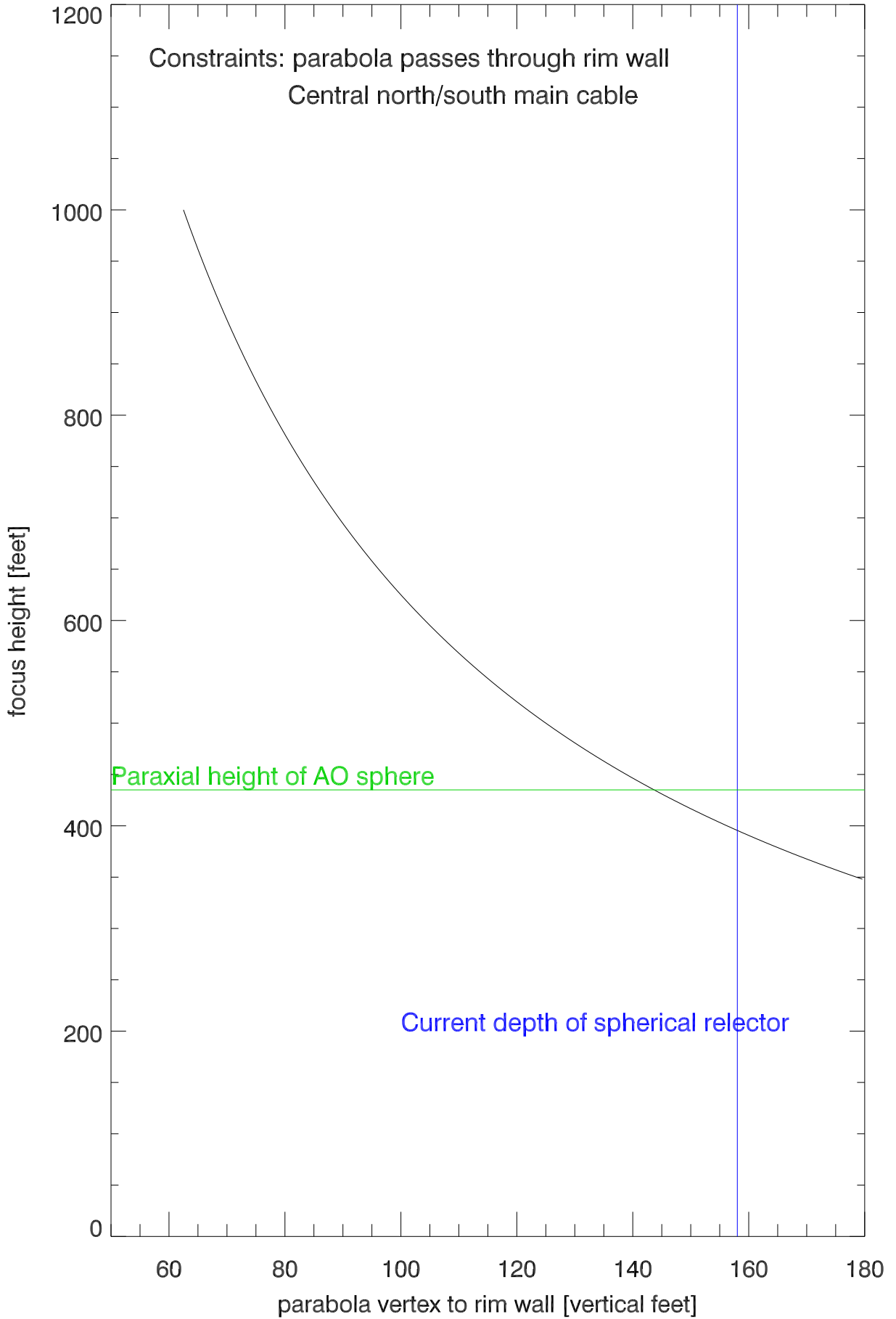
Focal height vs depth of dish below rim wall for a parabola
