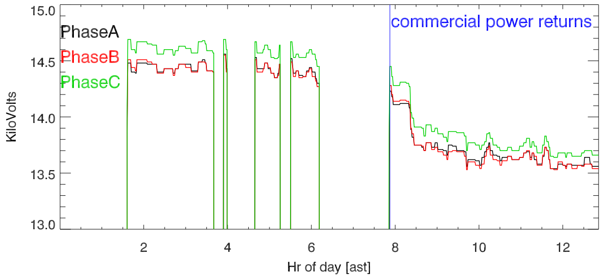
19apr18 site power. PhaseToPhase voltages at breaker input
