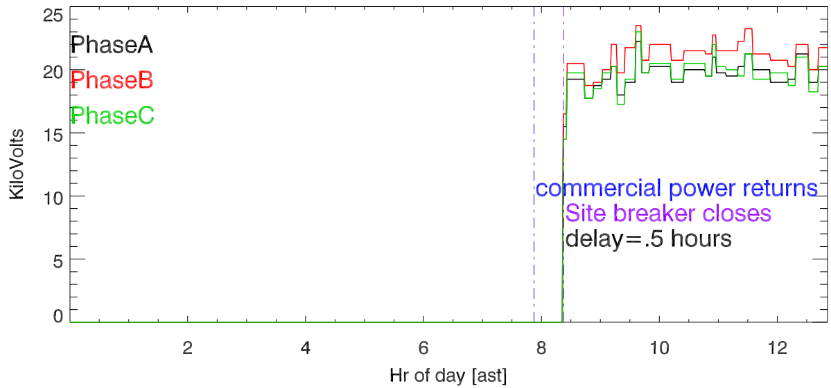
Current through breaker
