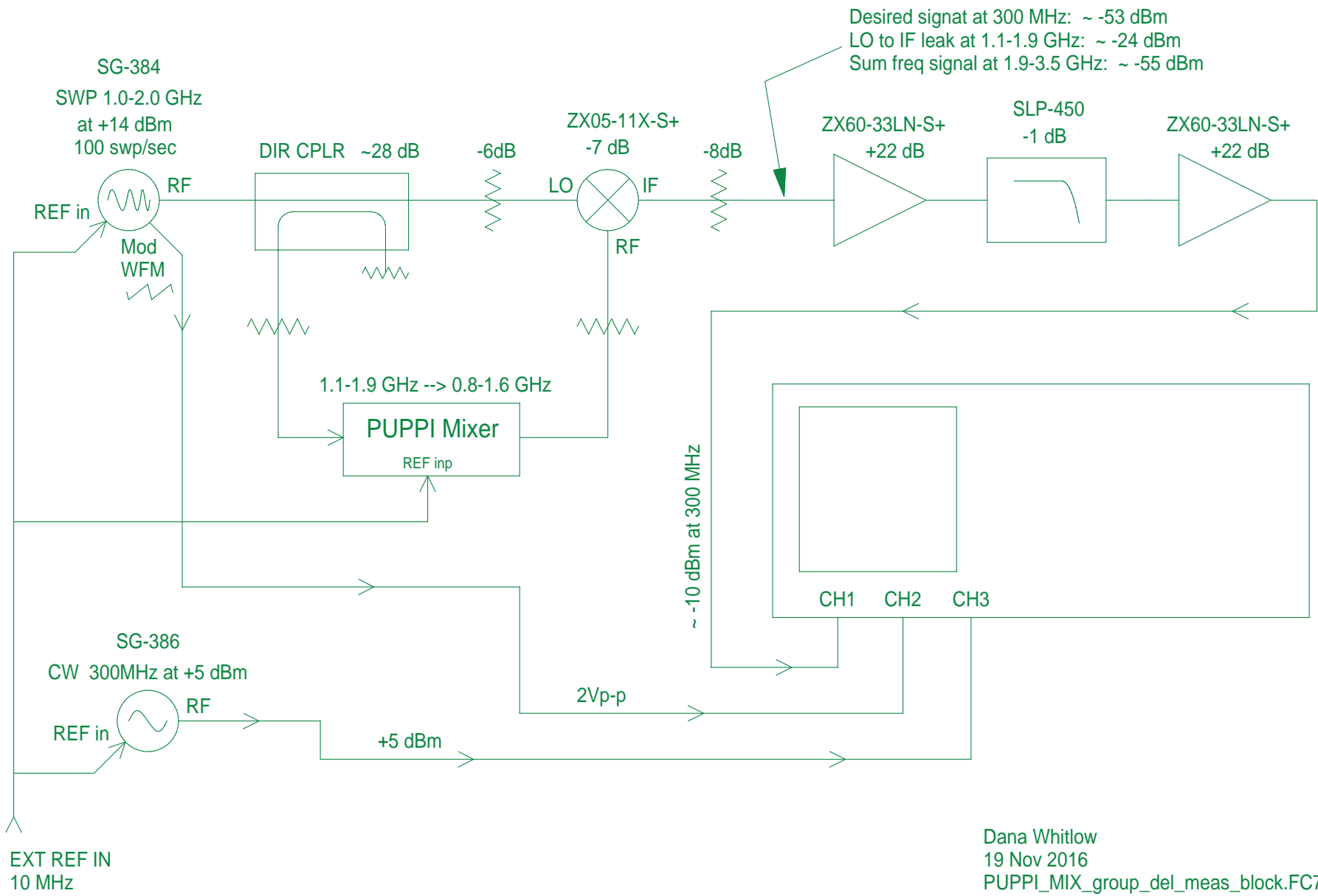
PUPPI_MIXER Group Delay Measurement Setup Also see PUPPI_MIX_group_del_meas_TOO.txt
