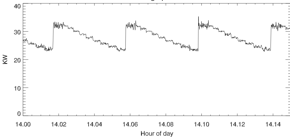
Average power
