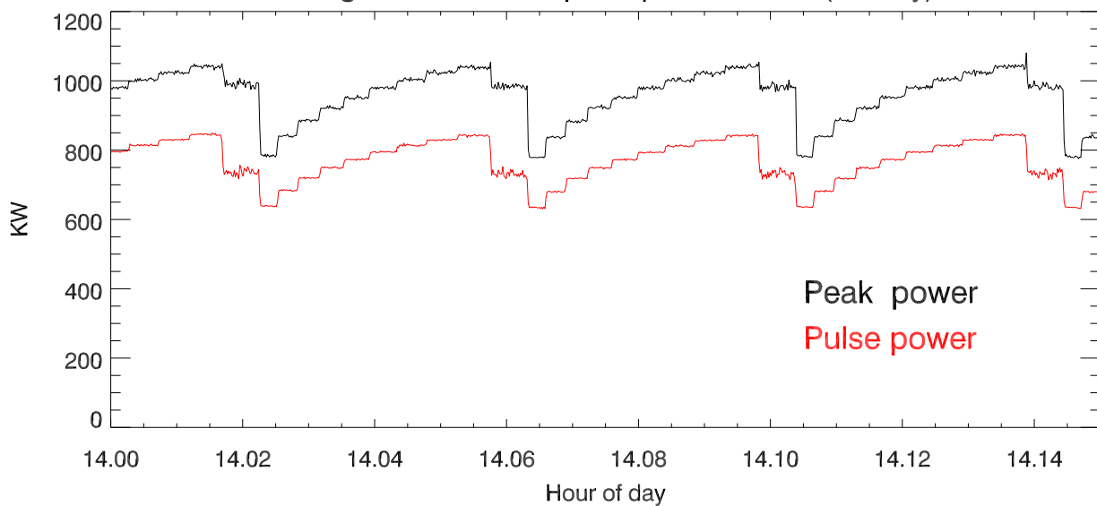
19aug11 T2635 Peak, pulse power 430 Tx (ch only)
