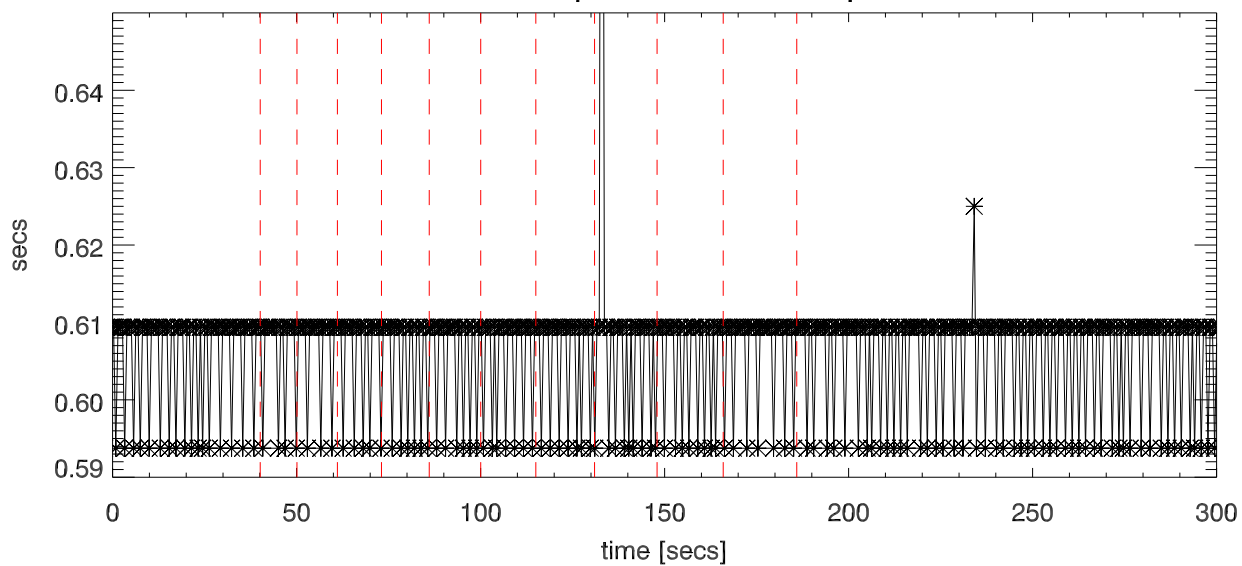
Time between samples returned from power meter
