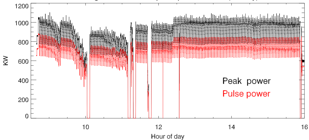
19aug11 T2635 Peak, pulse power 430 Tx (ch only)
