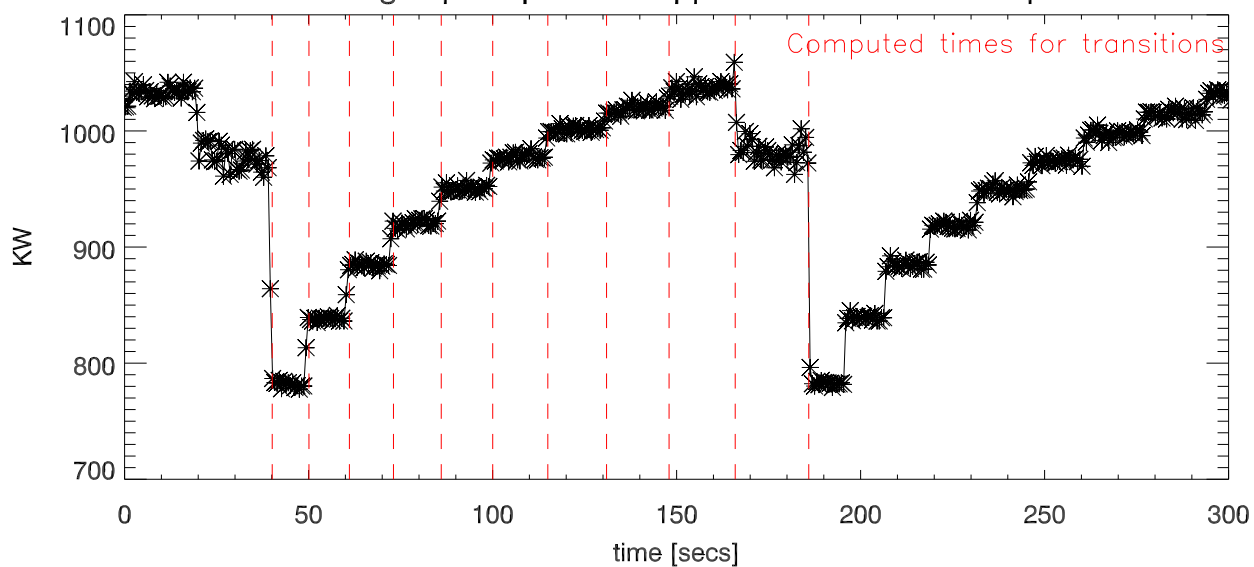
19aug11 peak power for ipps 1040 to 1872 then clp
