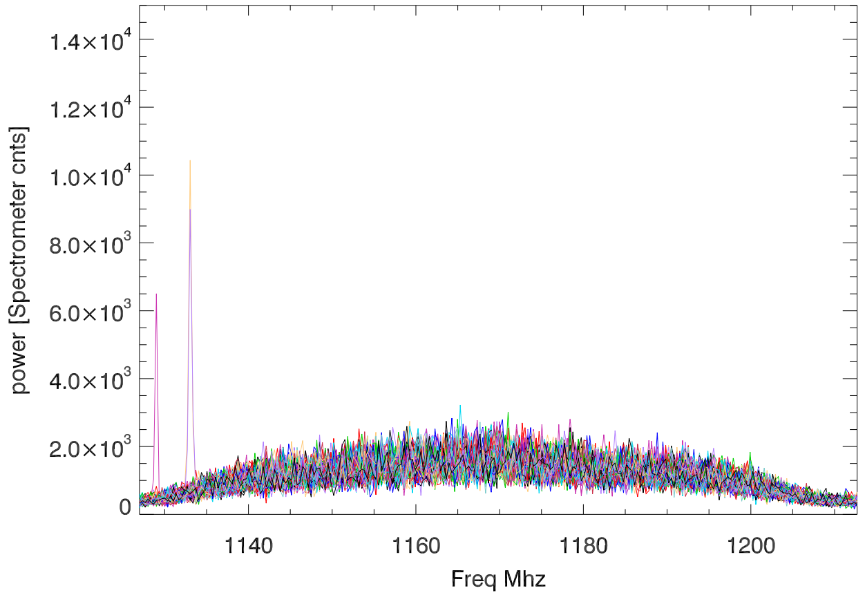
29sep12 p2679 lbw, B1919+21,file:200. 100Spectra. PoIA
