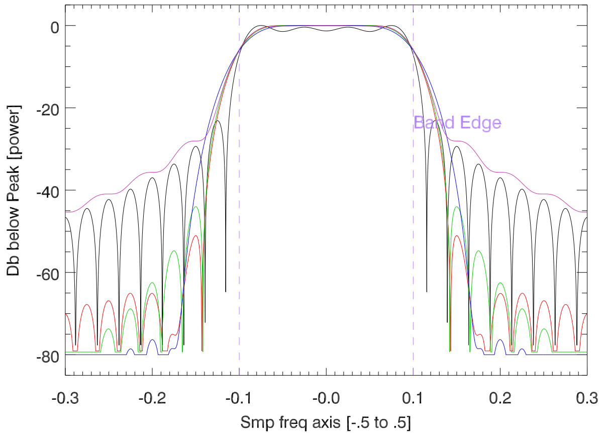
Blowup freq response for mock Digital filters
