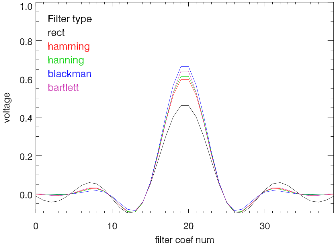
Time domain response Mock digFilt. dec= 5
