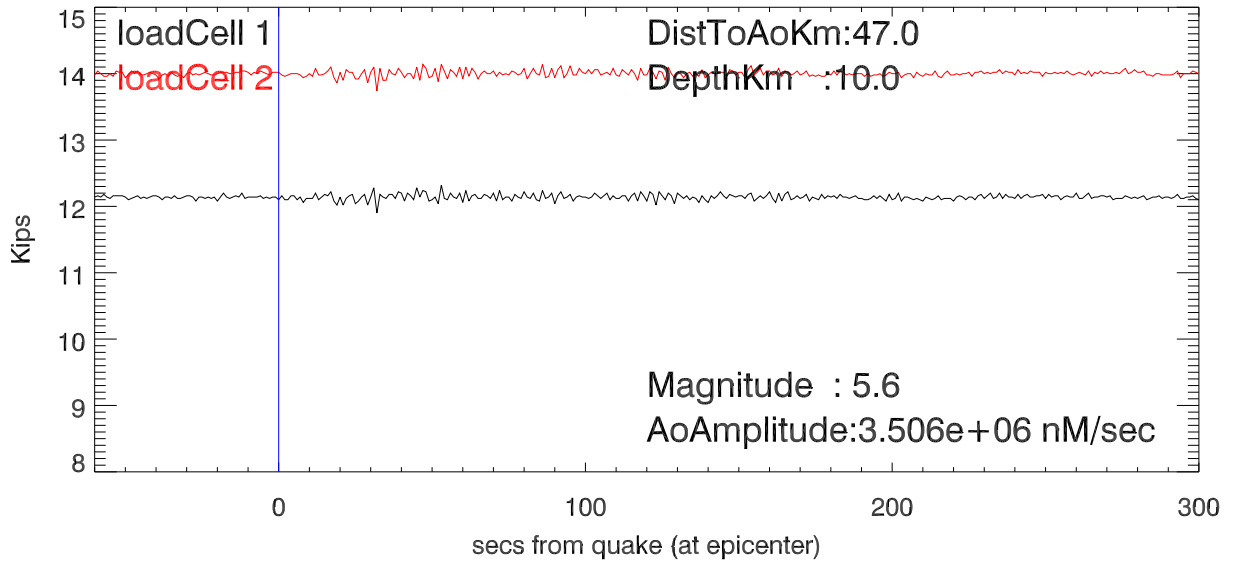
20200107 08:34:02(UTC) quake. tension in Td12
