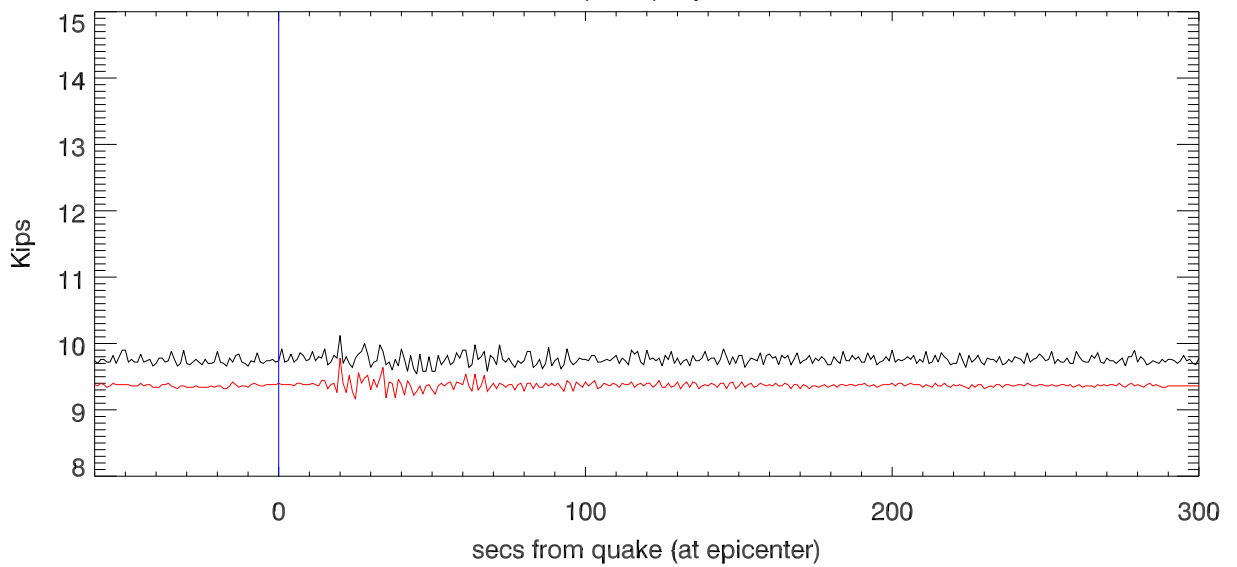
20200107 08:34:02(UTC) quake. tension in Td8
