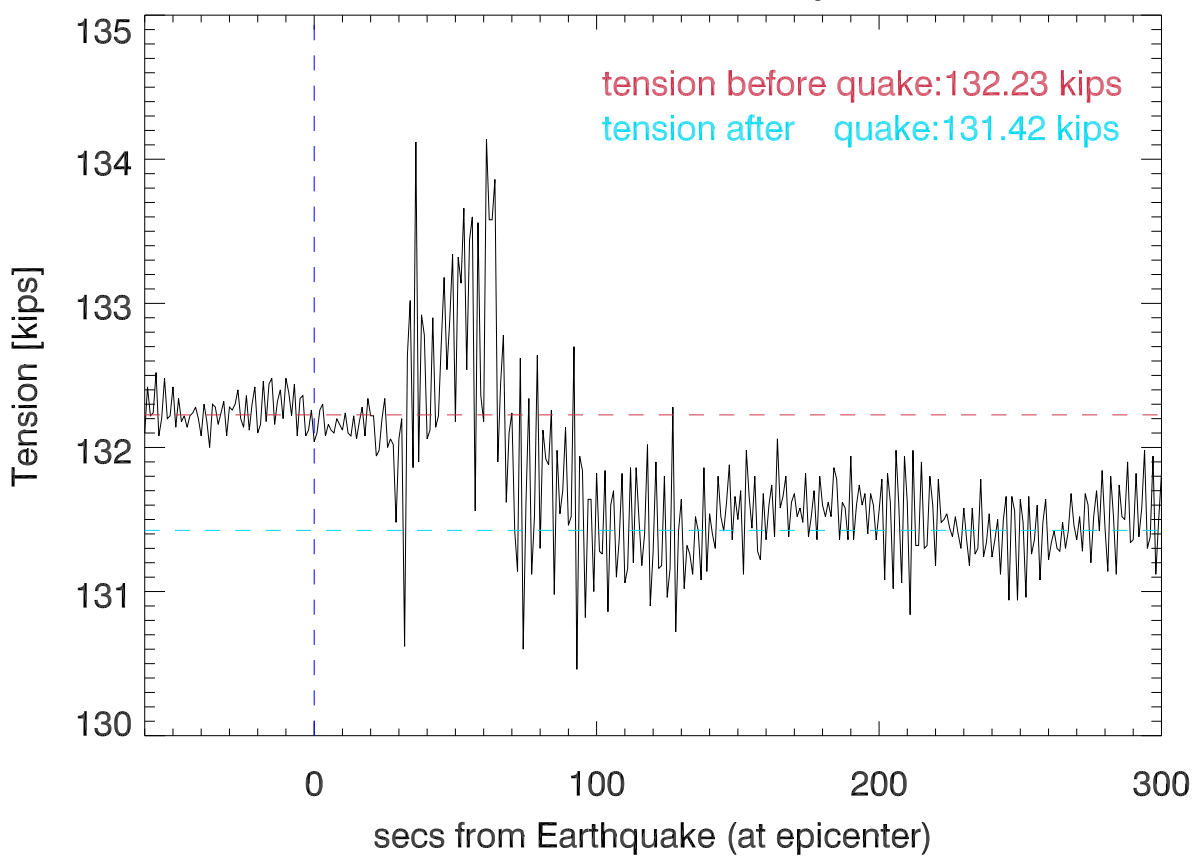
Combined tension all jacks
