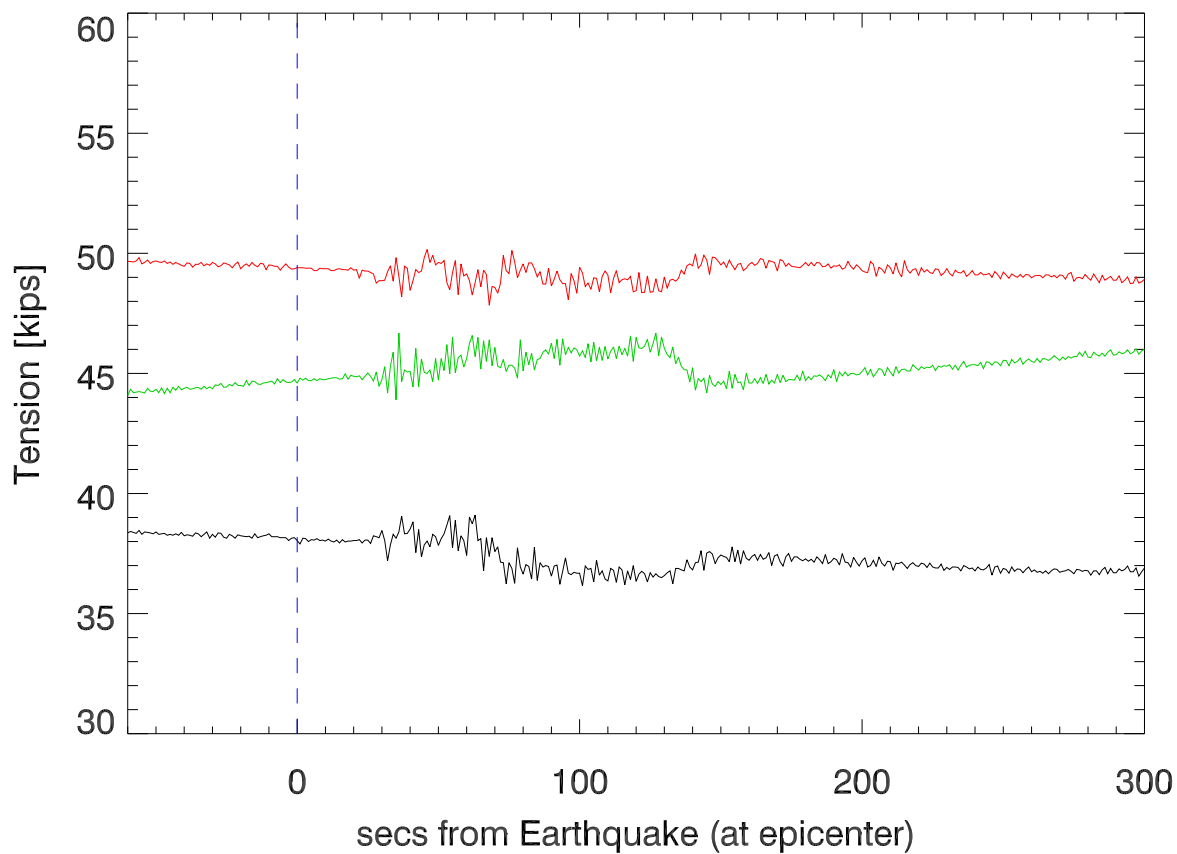
Tension in each td jack
