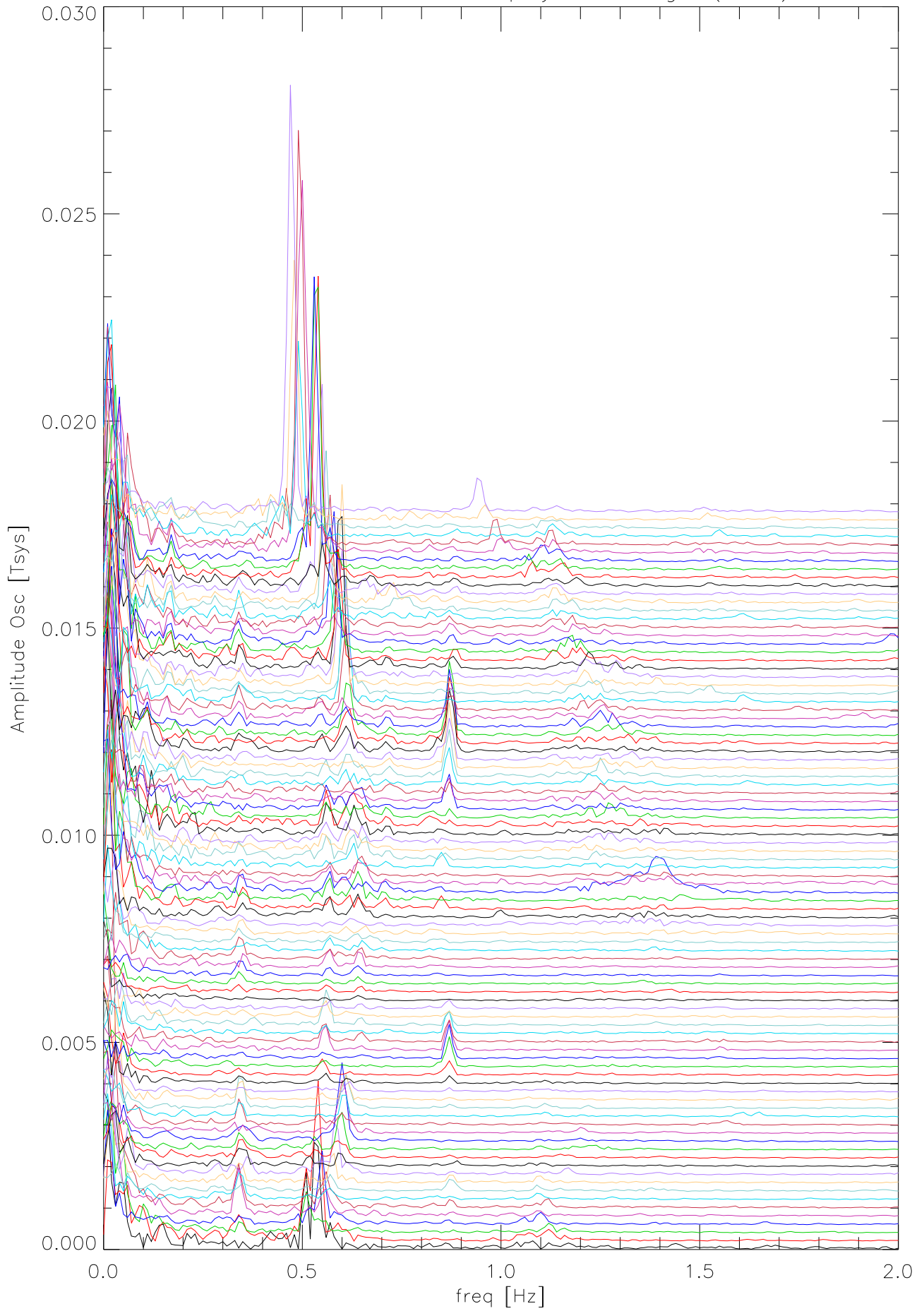
11mar06 oscillation freq by hour angle (2 Hz)
