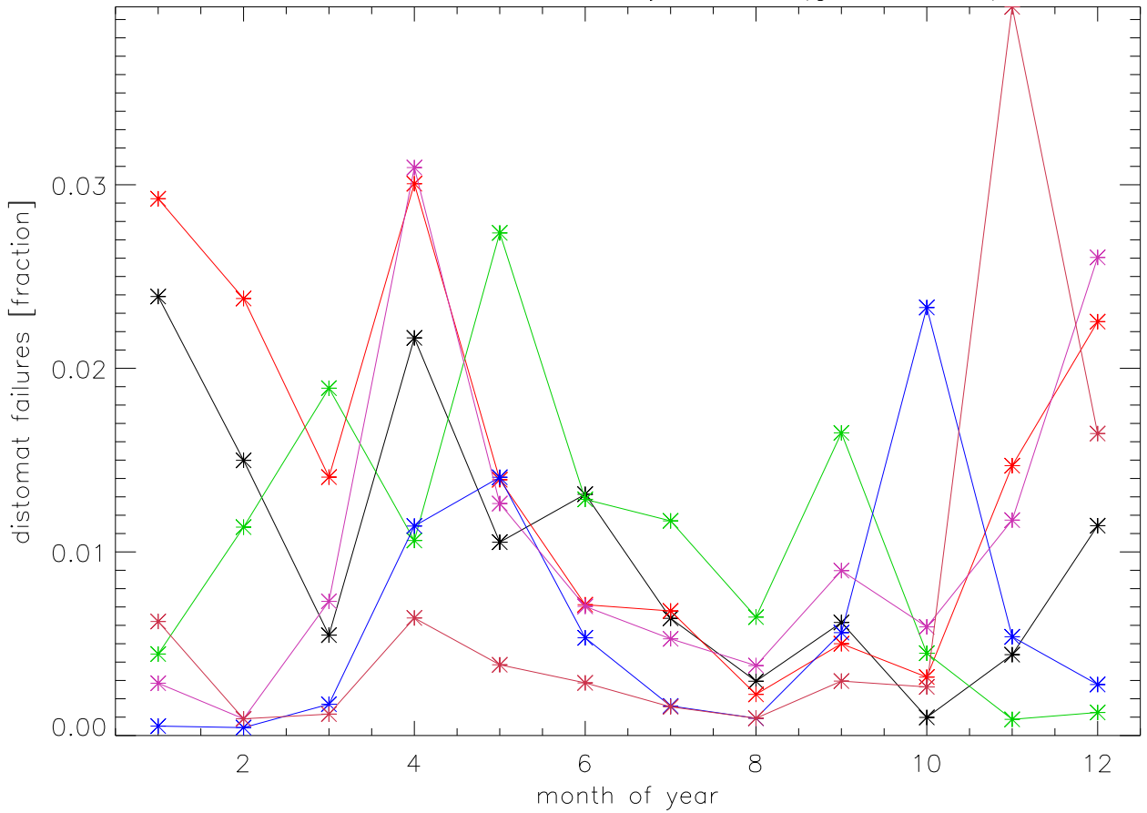
2008 distomat failures by month (gooddist=3)
