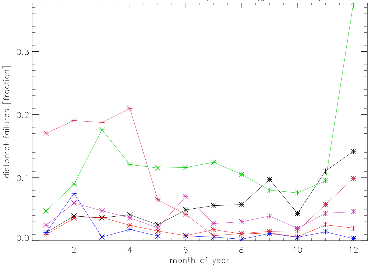
2016 distomat failures by month (gooddist=0)
