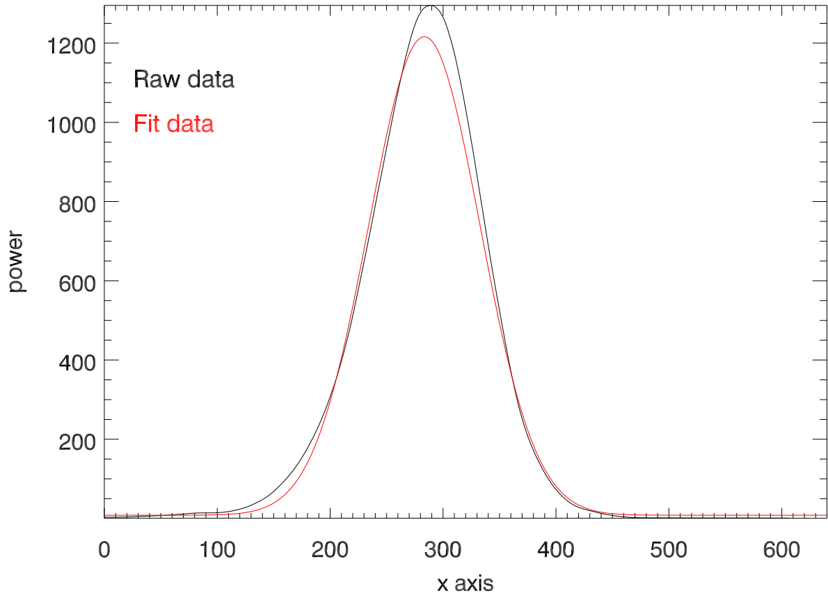
x cut through center of beam
