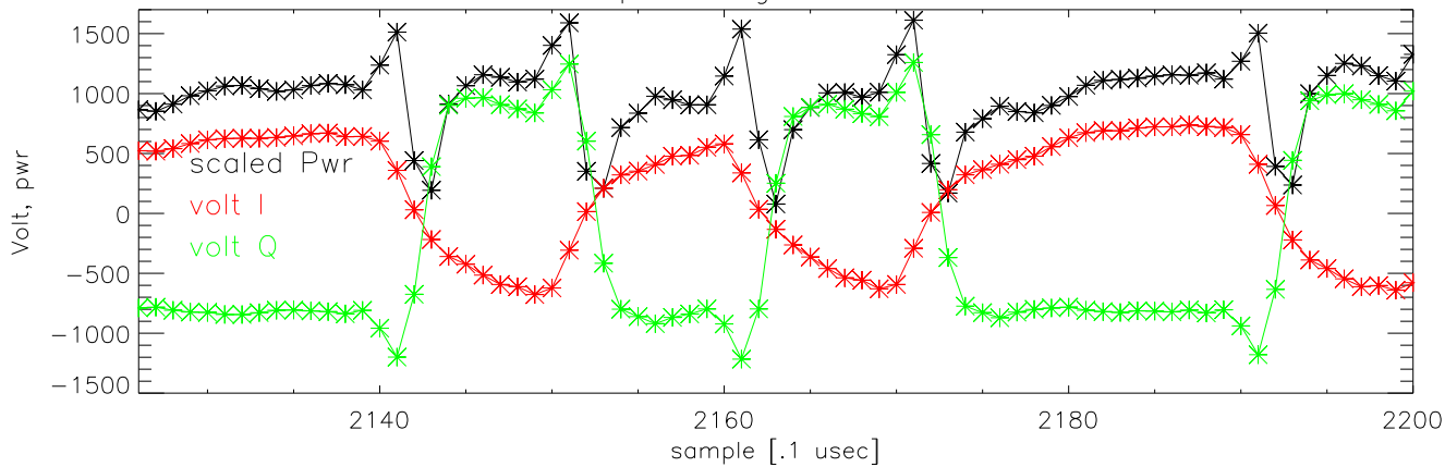
blowup showing baud transition
