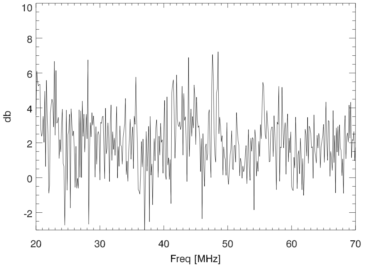
DoorOpen/DoorClosed spectra
