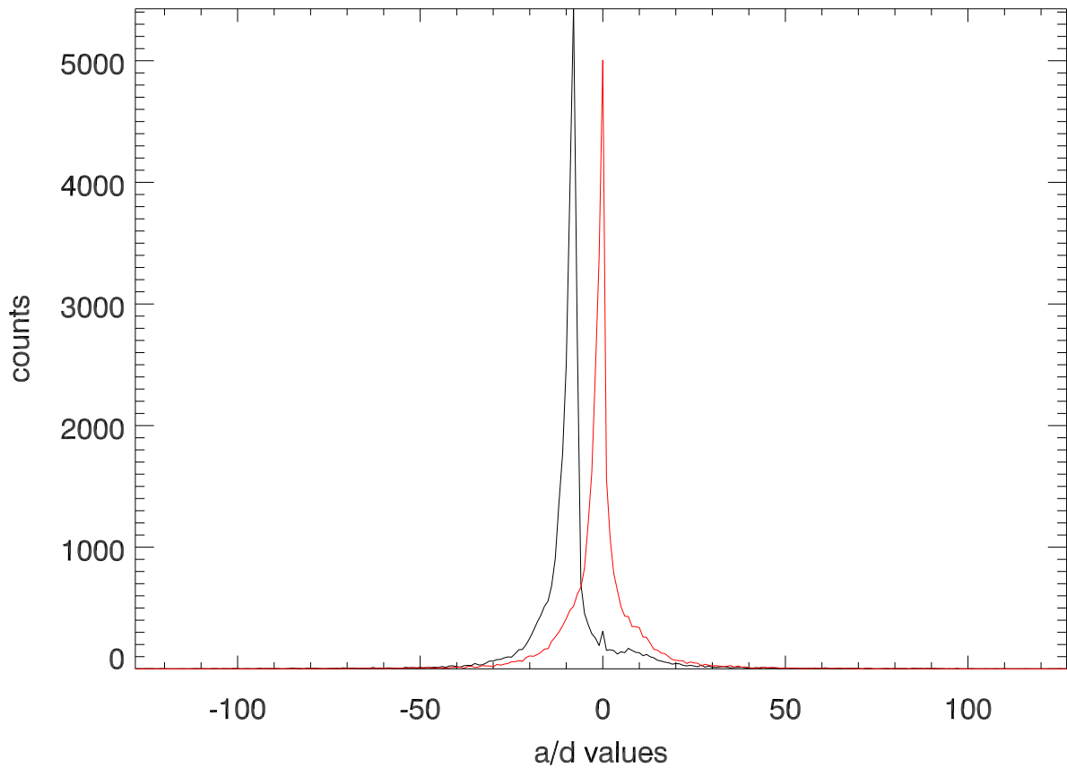
Histograms of i,q voltages samples
