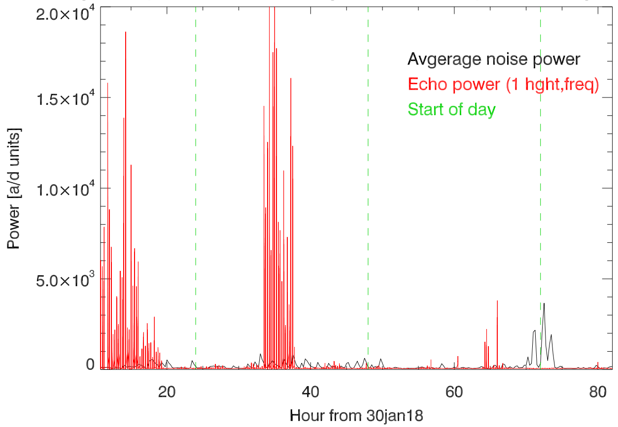
AvgNoise power for each ionogram, and echo power (1height,freq)
