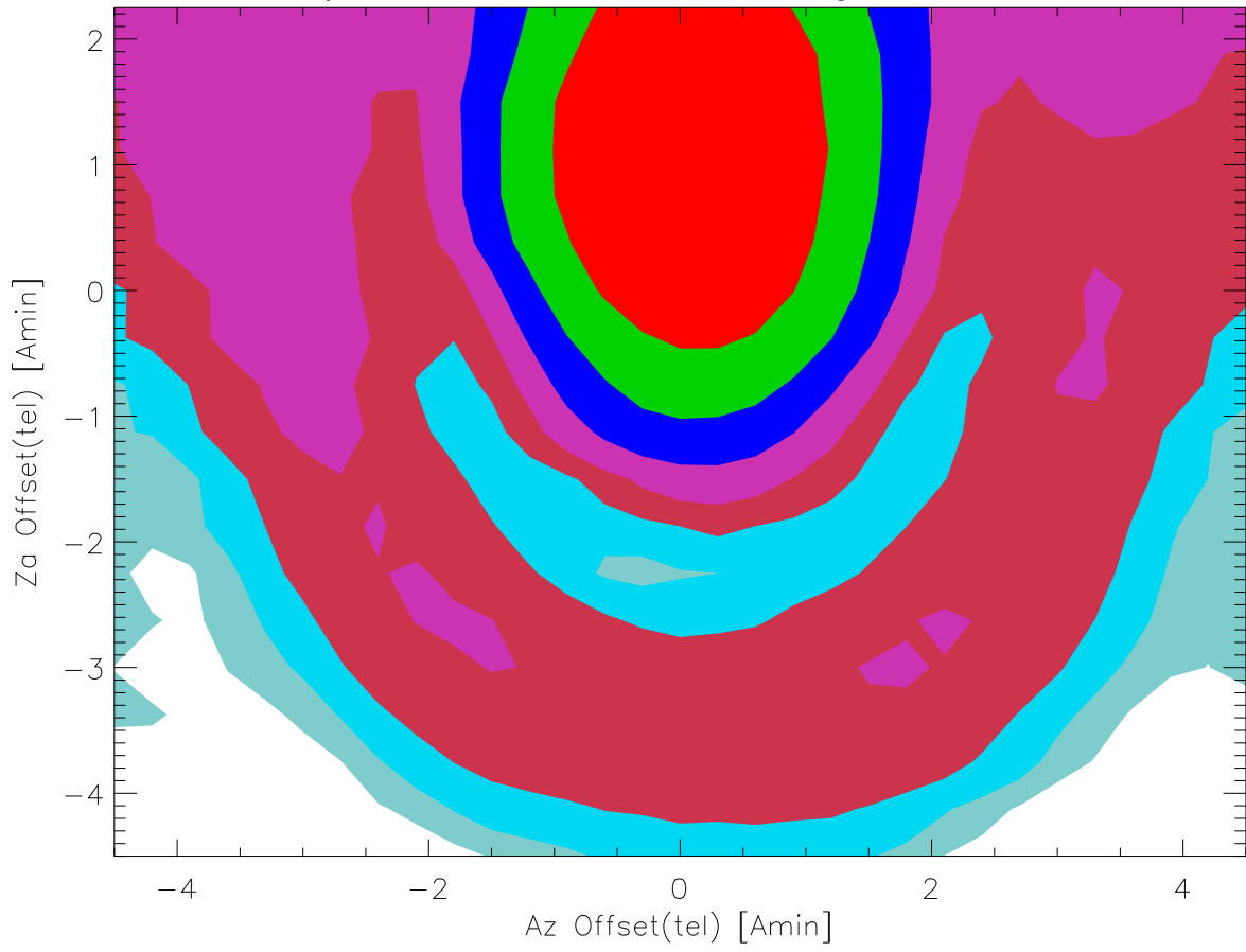
21-21 jun10 A0 partial superfine grid. 3db contours
