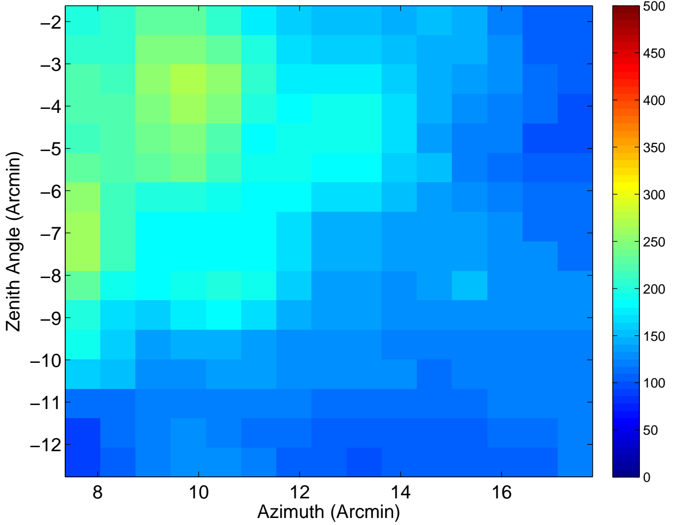
C5 Ae/Tsys Map ( z = 7.463 cm)
