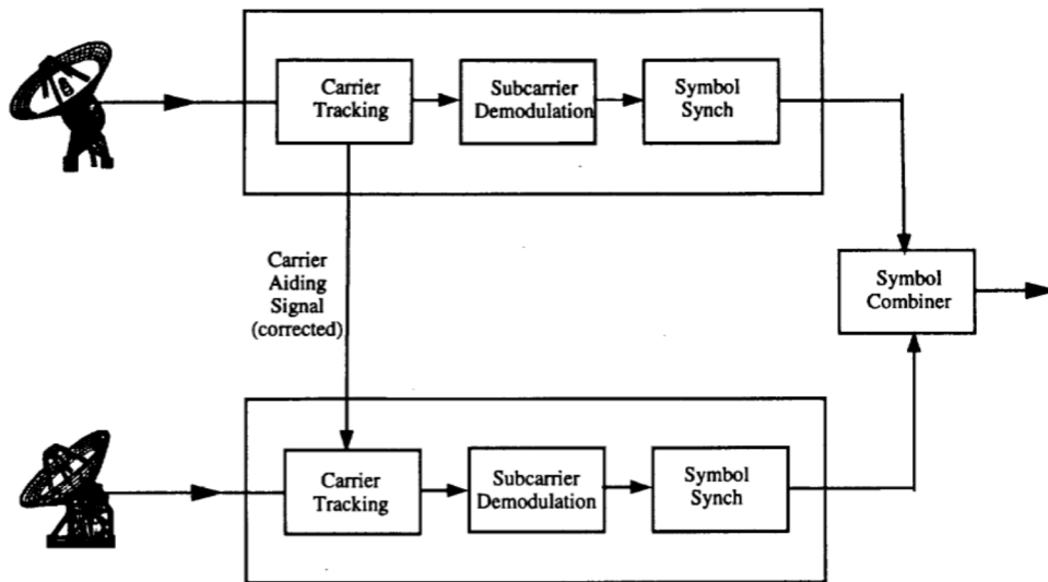
Figure 3-3. Block Diagram for Carrier Arraying.
