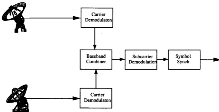
Figure 3-2. Block Diagram for Baseband Combining.
