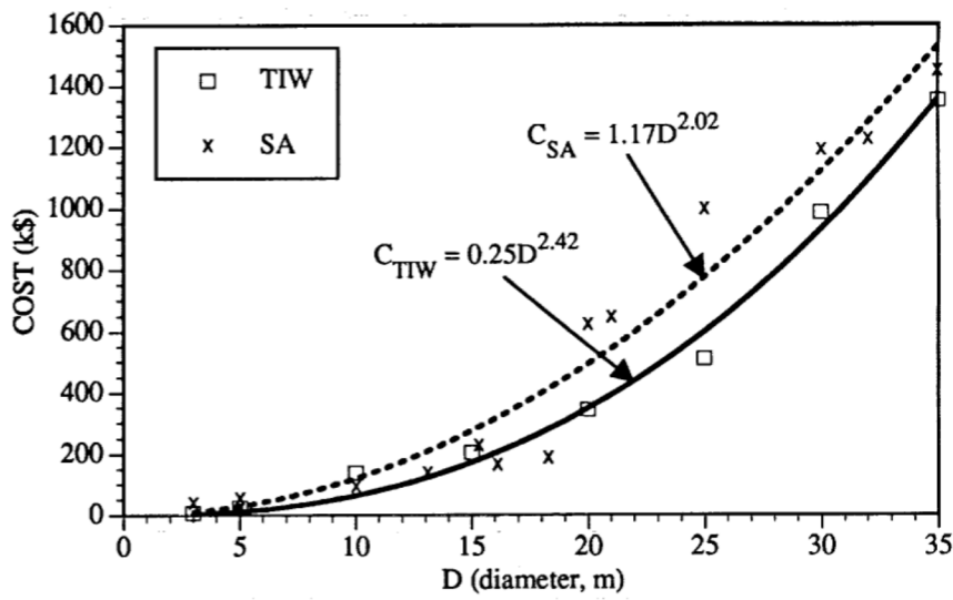
Figure 4.2-9. Cost and power law fit for the antenna shipping, installation, and testing data.
