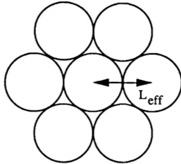
Fig. 4.4-3. The unit cell for the hexagonal close-pack array layout, often referred to as a first-order Gosper snowflake. The distance between centers L_{eff} is determined by the shadowing constraint.
