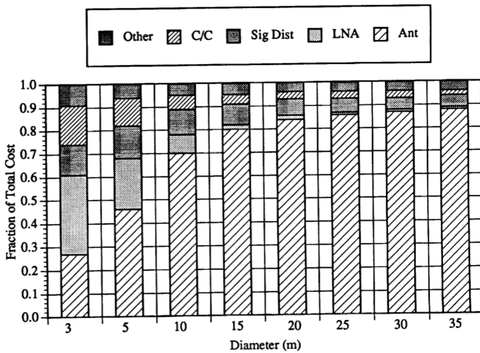
Figure 6-1. The fractional subsystem cost versus antenna diameter.
