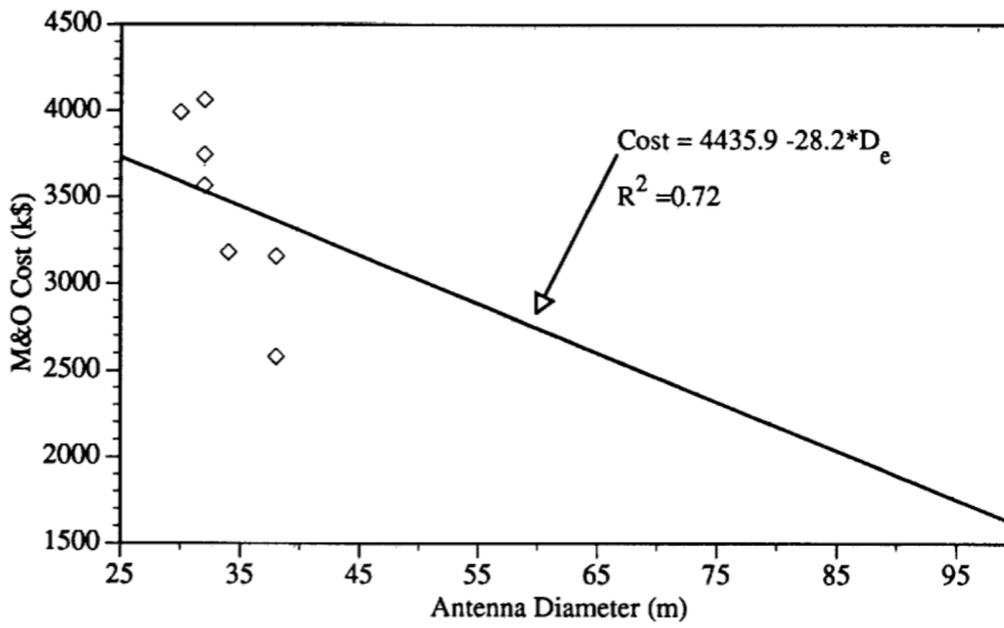
Figure 4.9-2. M&O costs as a function of array element diameter (from the LAAS study).
