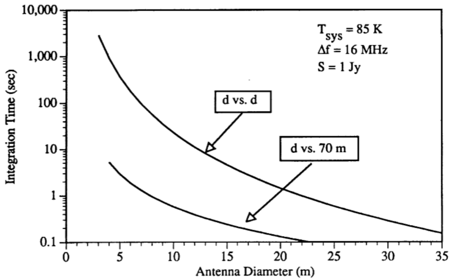
Figure 3-8. The integration time needed to achieve snr = 5 for two array elements vs. element diameter. In the first case both elements are assumed to have equal diameter (d vs. d) and in the second case one of the elements is assumed to be a 70-m antenna.
