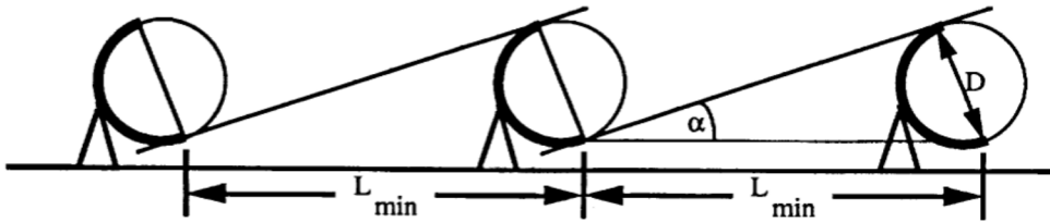
Figure 4.4-2. Geometry of the antenna shadowing constraint.
