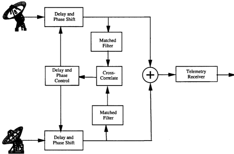
Figure 3-4. Block Diagram for Full Spectrum Combining.
