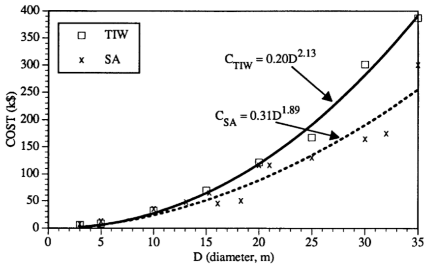
Figure 4.2-7. Cost and power law fit to the antenna foundation data.
