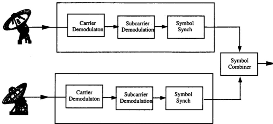
Figure 3-1. Block Diagram for Symbol Stream Combining.
