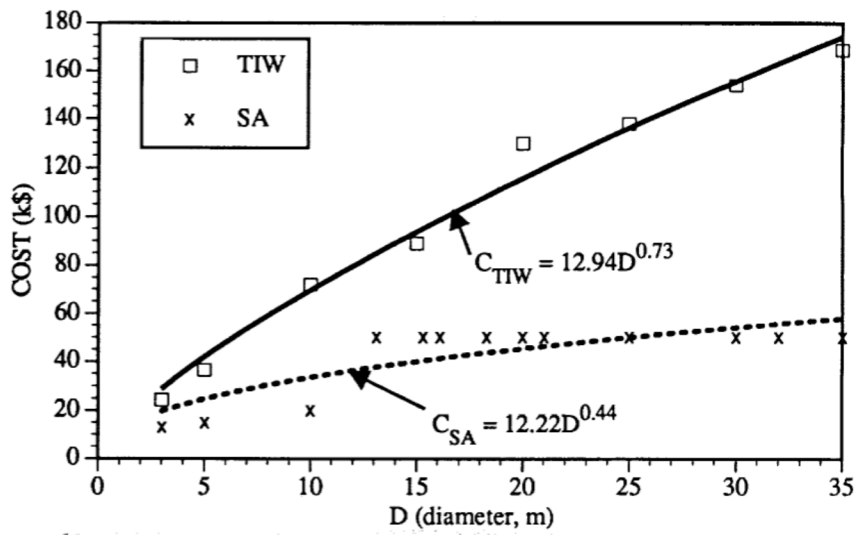
Figure 4.2-5. Cost and power law fit to the antenna position control data.
