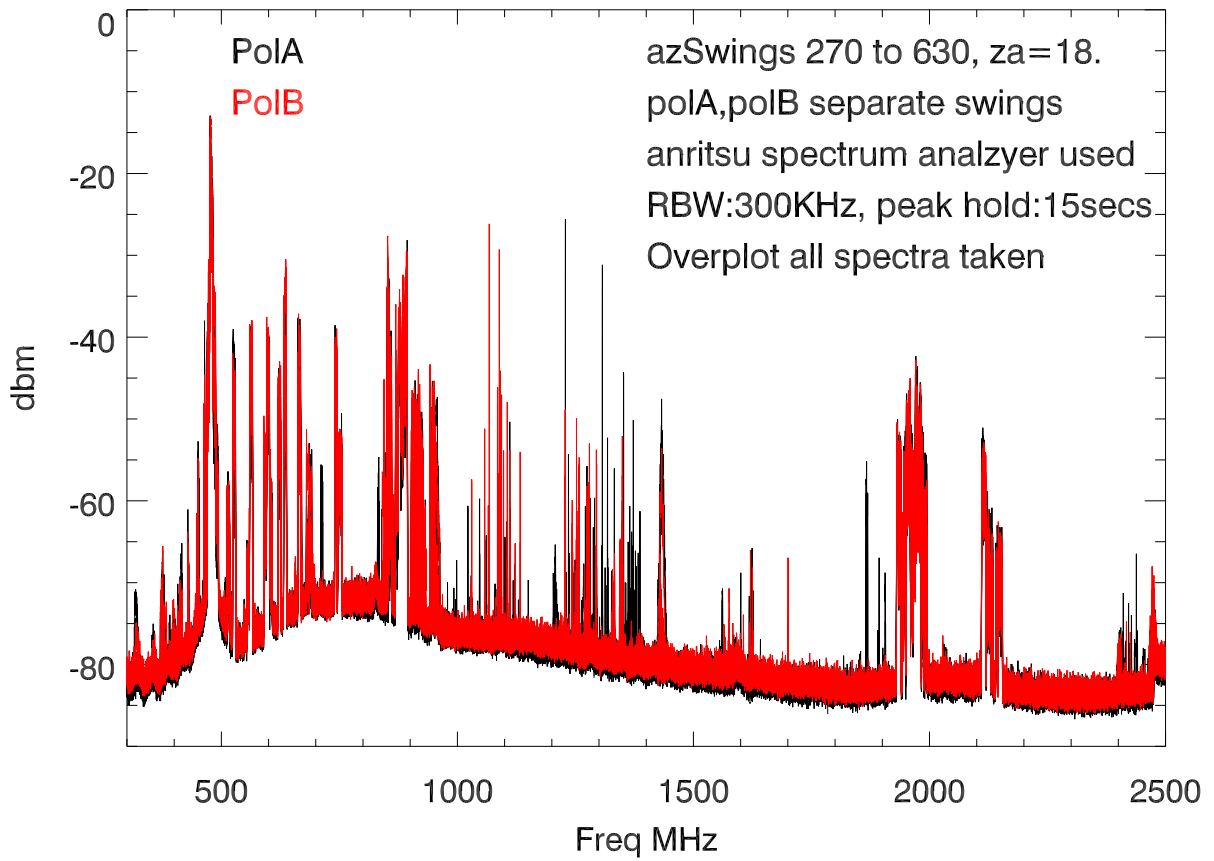
AO40 21may15:(fat dipole + amps) output vs Freq
