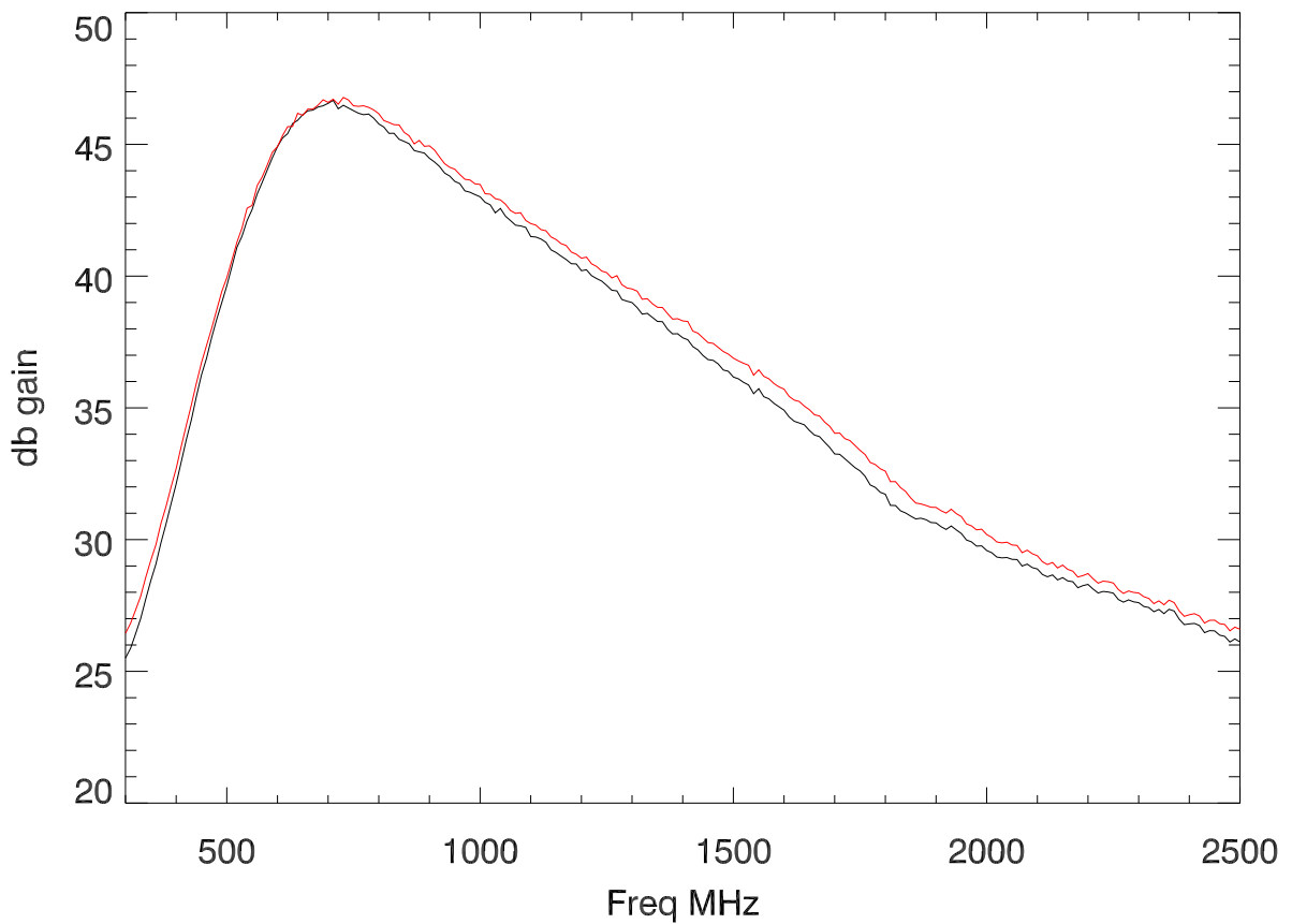
AO40 02may15: measured S21 (gain) vs freq for amps (no filters)
