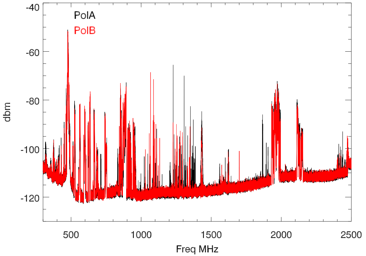
Remove amp gain. power at output of dipole
