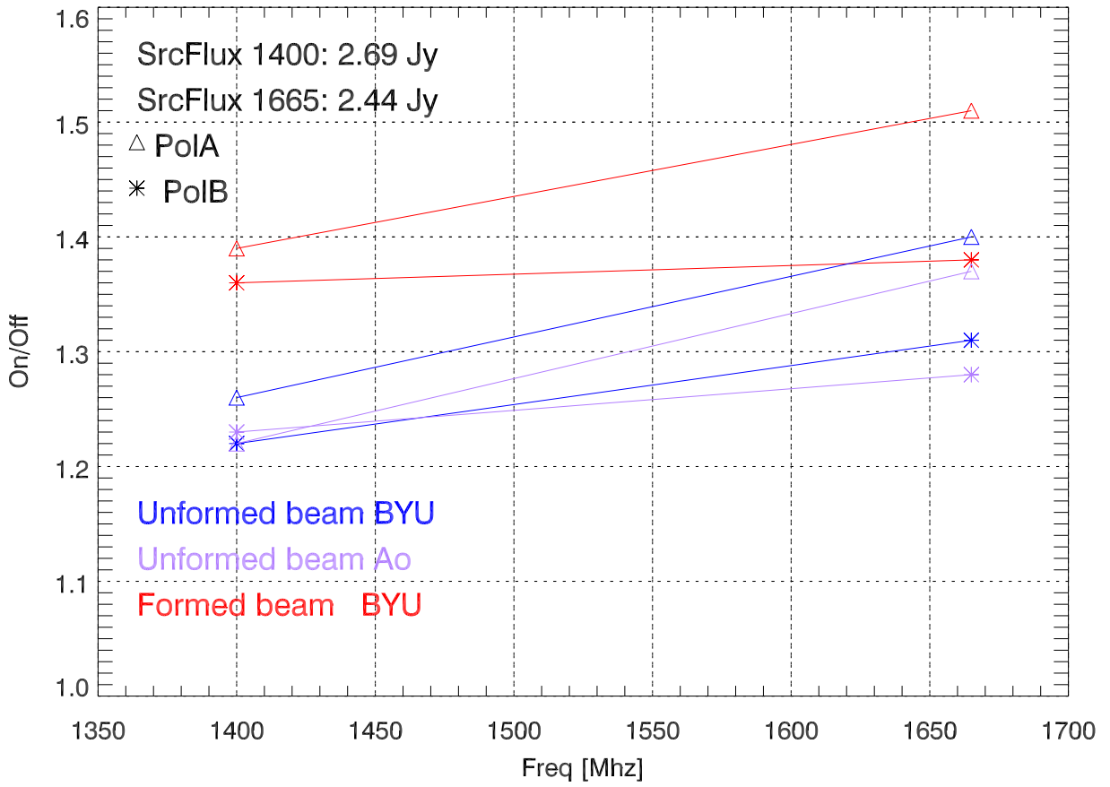
03aug13 ao19 dipole 1 Yfactor on J0603+219 (B0600+219)
