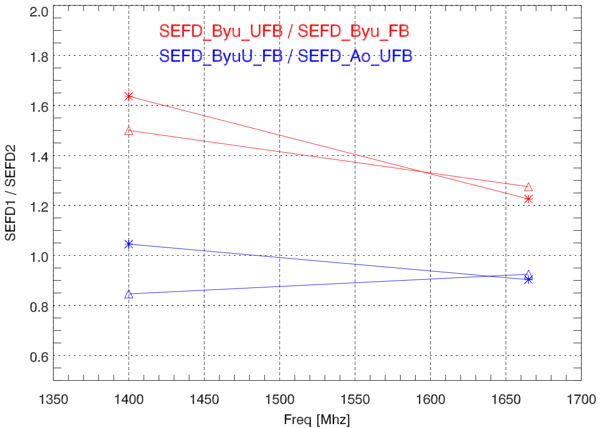
03aug13 ao19 dipole 1 SEFD Ratios on J0603+219
