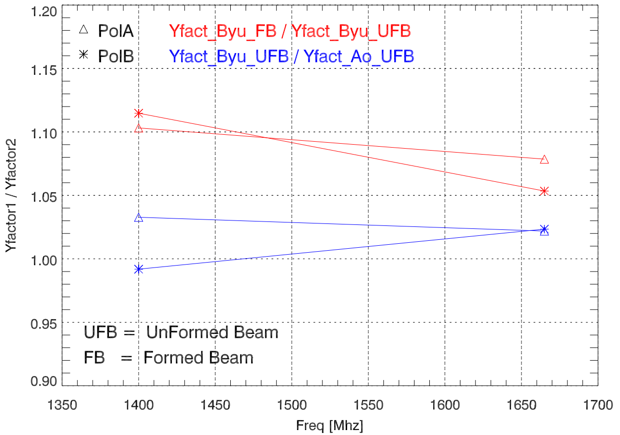
03aug13 ao19 dipole 1 Yfactor Ratios on J0603+219
