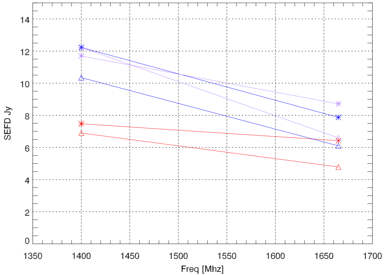
03aug13 ao19 dipole 1 SEFD
