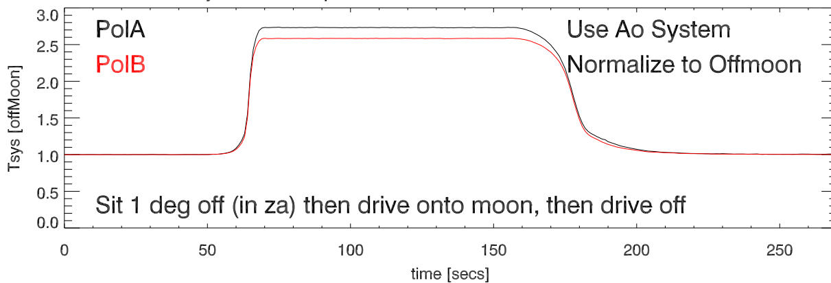
30jul13 ao19 Dipole 1. Scan 1 drive onto moon and then off
