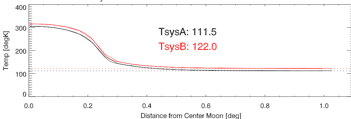
Scan 1 Tsys vs distance from center of moon. Use Tmoon = 193.1 K
