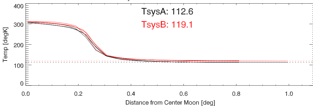
Scan 2 Tsys vs distance from center of moon.
