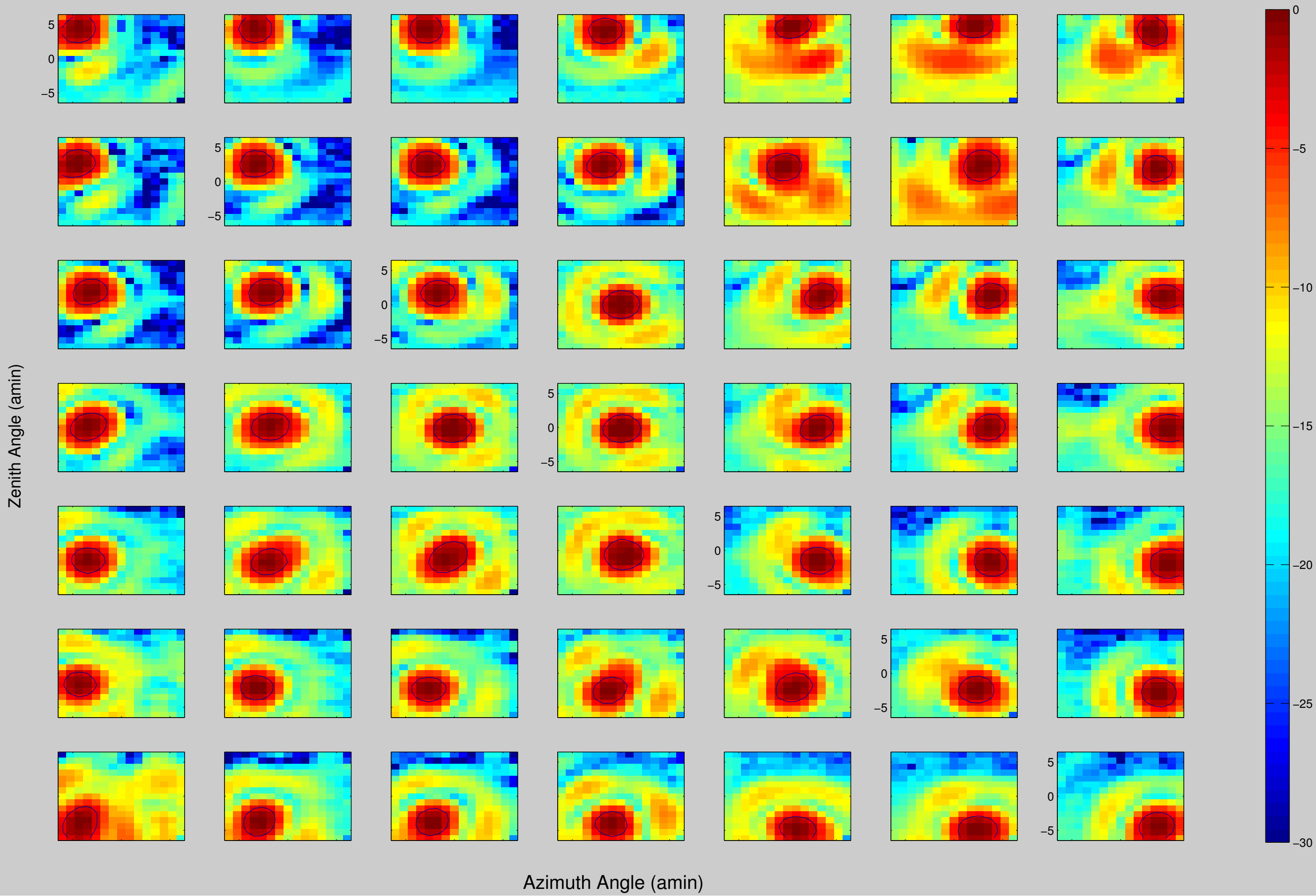
Formed Beams for Grid /media/Disk0/07_28_2013_15x15/default.mat, Frequency 1399.6094 MHz, Polarization A
