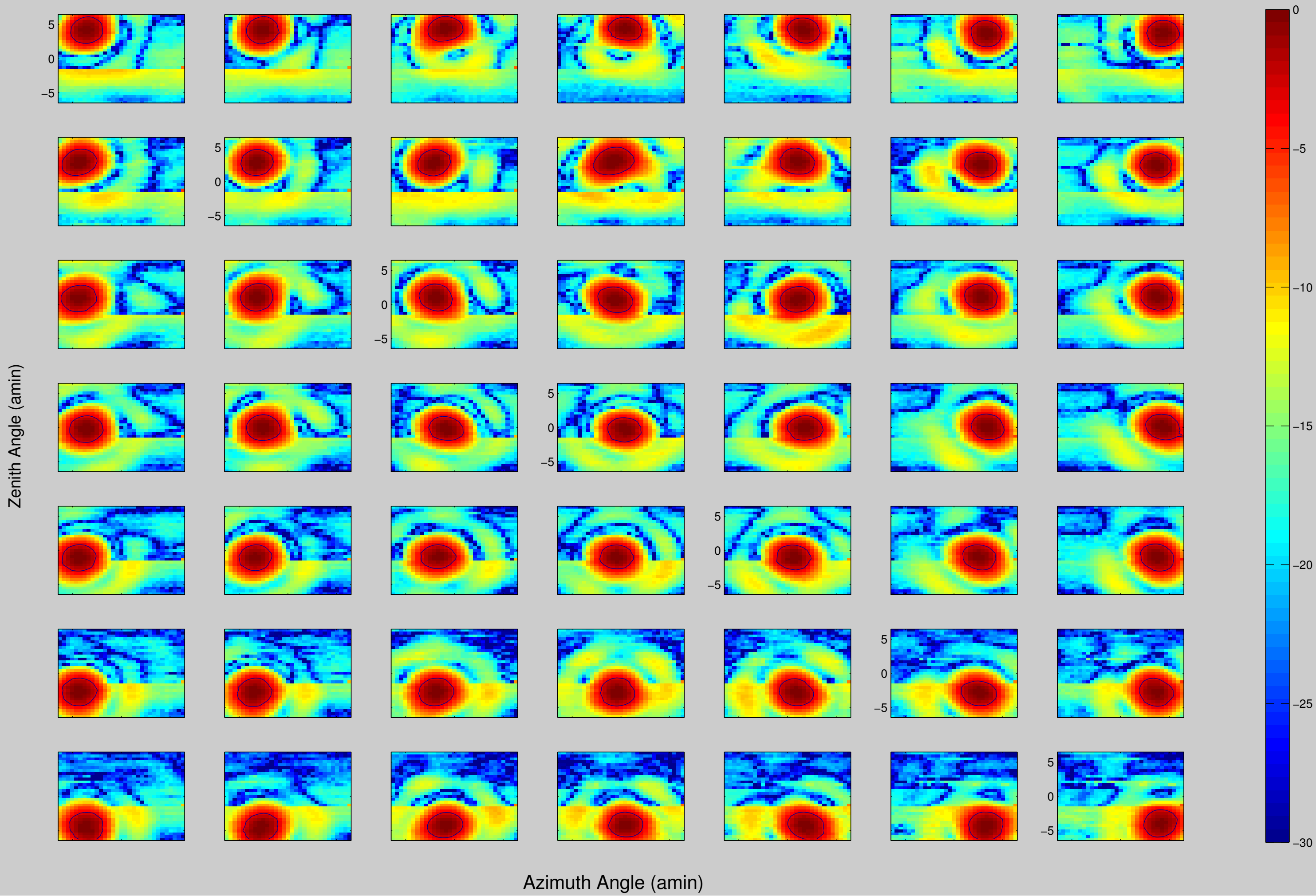
Formed Beams for Grid /media/Disk0/08_02_2013_evening_31x31_2/default.mat, Frequency 1399.707 MHz, Both Polarizations
