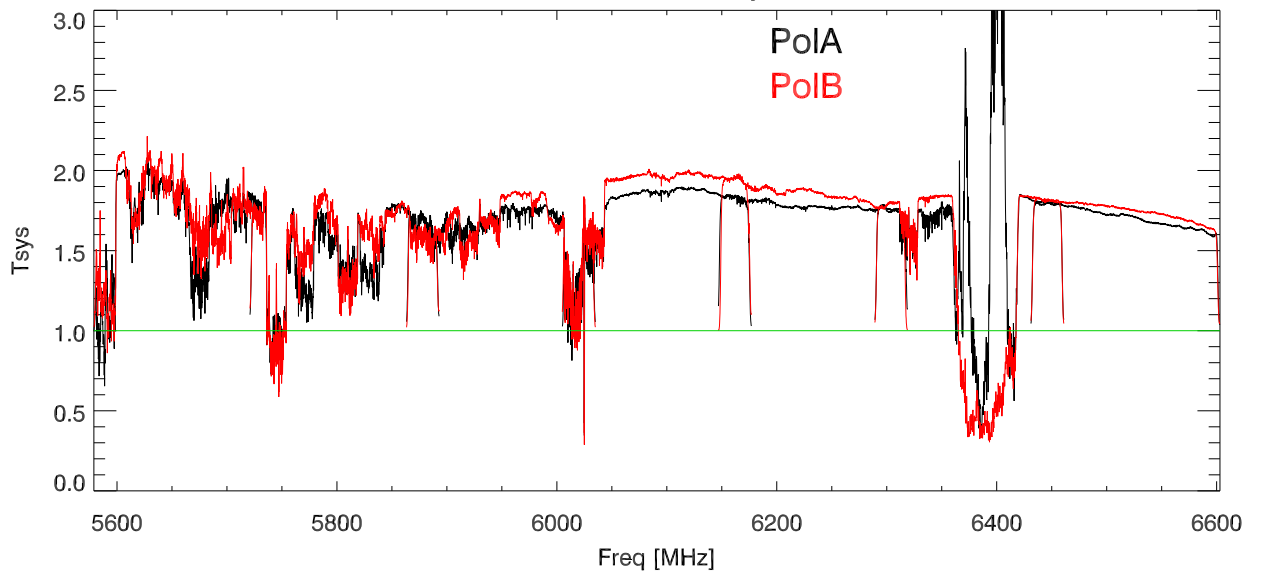
CalDeflection/Tsys
