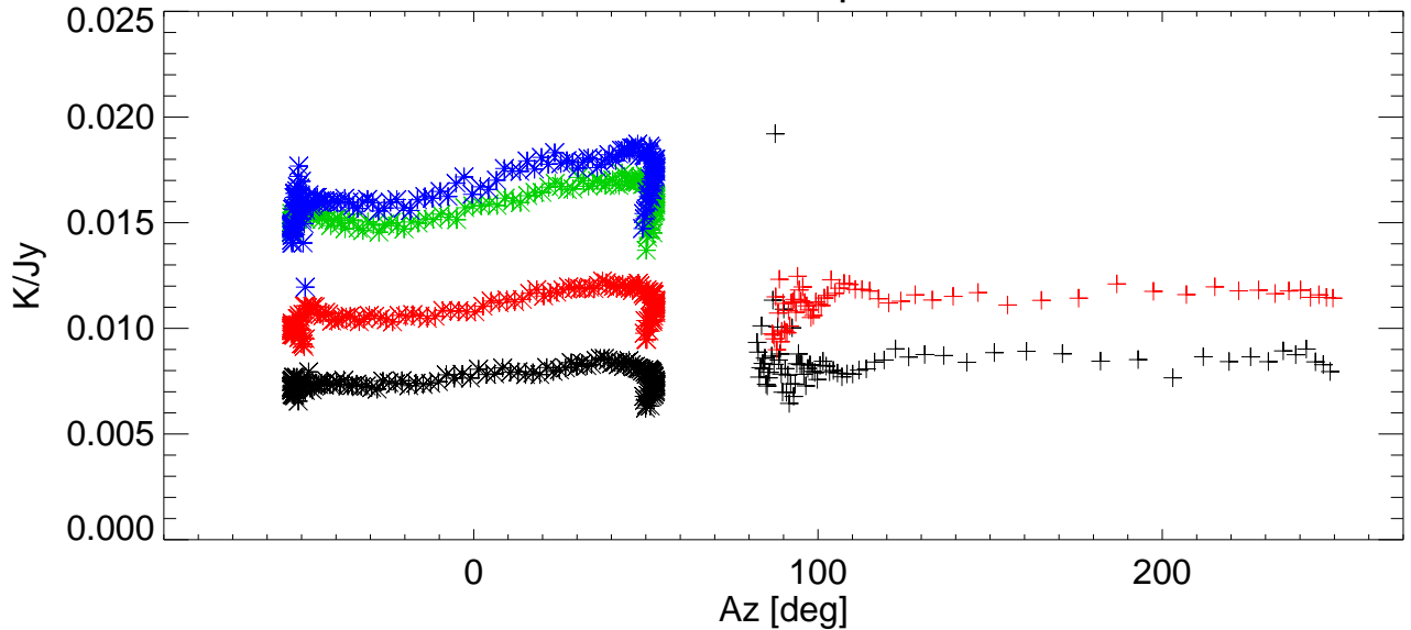
Gain vs Az for various shims. freq=9073 Pol:B RemoveBase.
