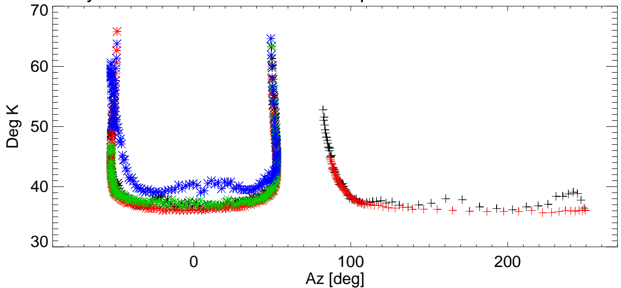
Tsys vs Az for various shims. freq=9073 Pol:B RemoveBase.
