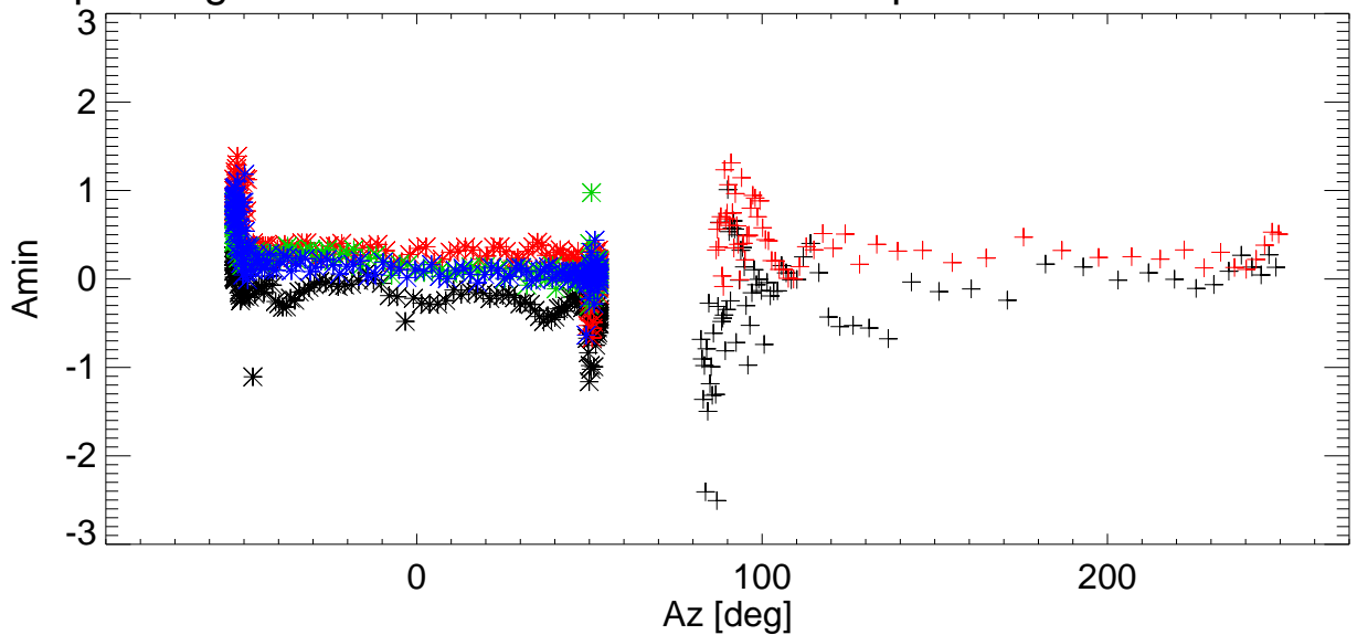
El pointing error vs Az for various shims. freq=9073 Pol:B RemoveBase.
