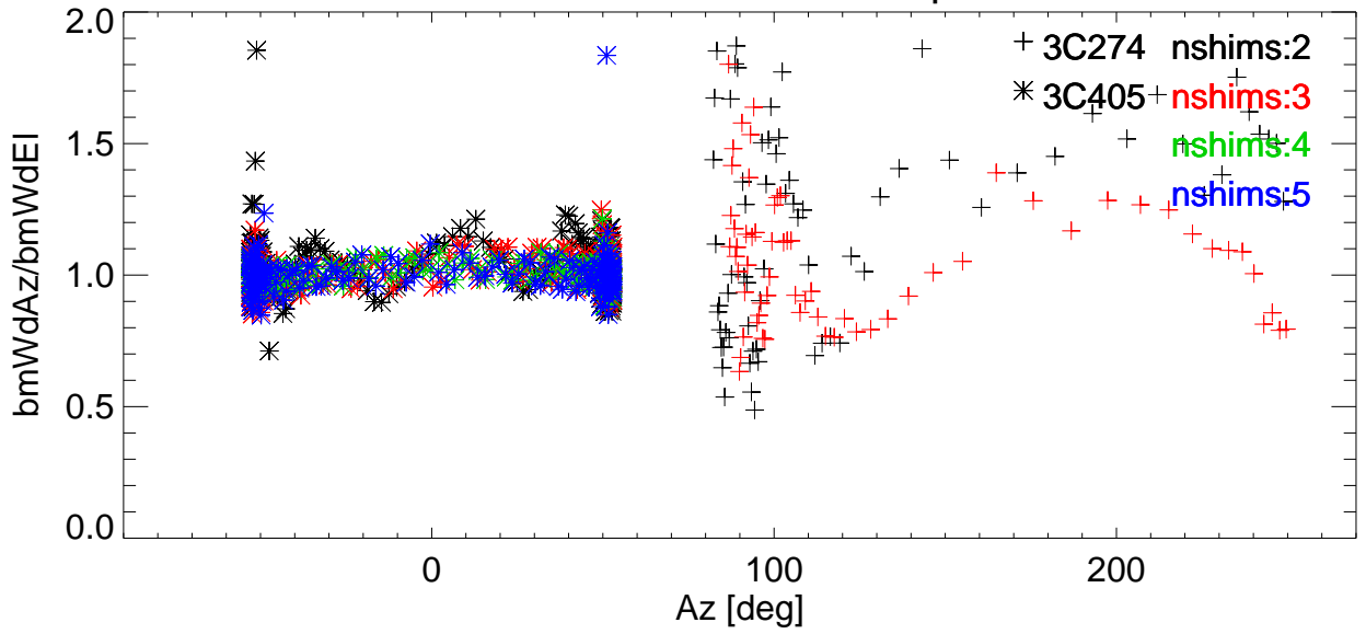
Az/EI BmWdRatio vs Az for various shims. freq=9073 Pol:A RemoveBase.
