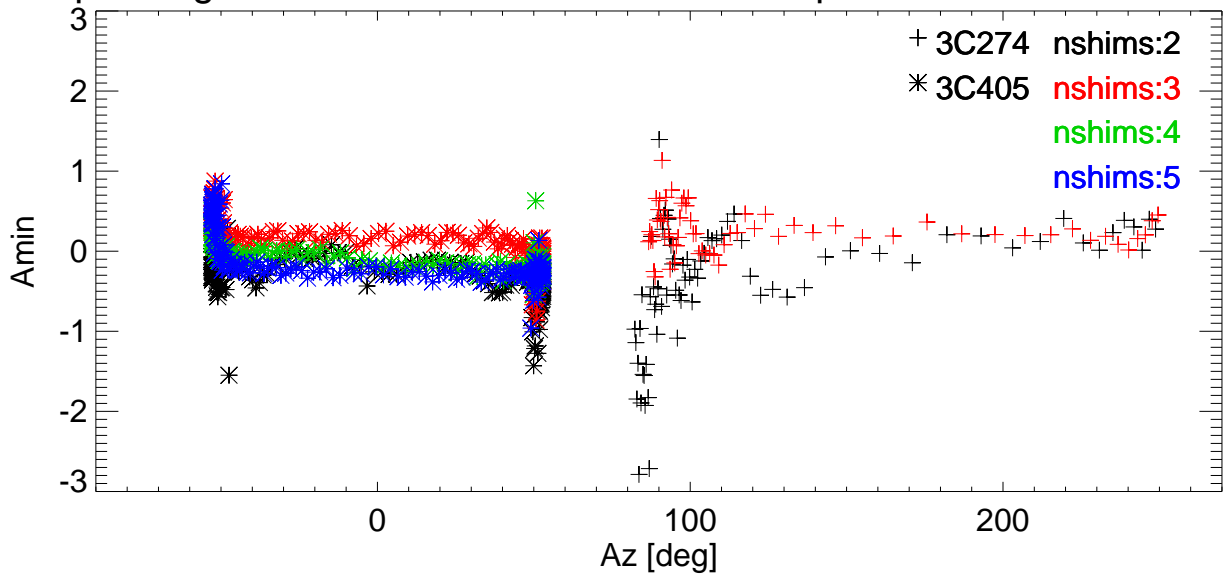
El pointing error vs Az for various shims. freq=9073 Pol:A RemoveBase.
