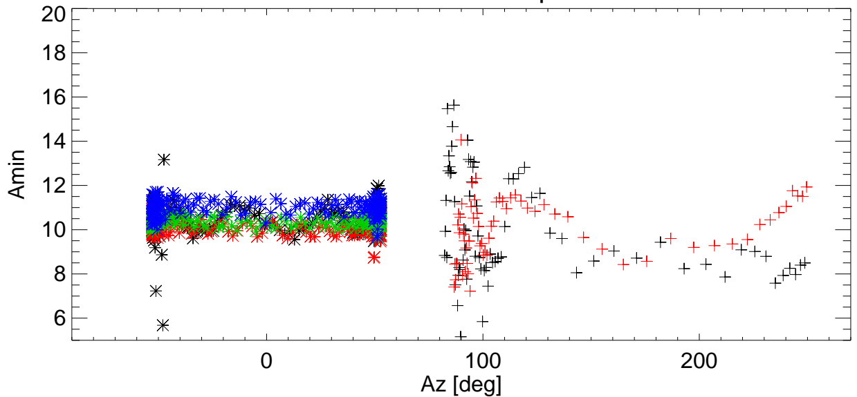
El BmWidth vs Az for various shims. freq=9073 Pol:B RemoveBase.
