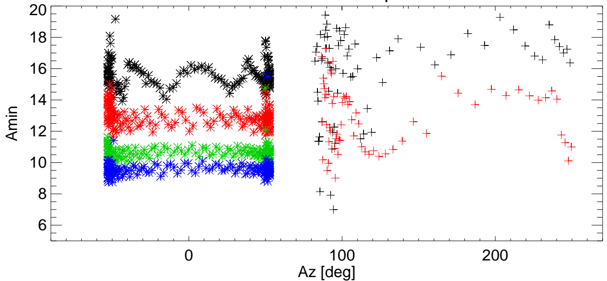
Az BmWidth vs Az for various shims. freq=9073 Pol:B RemoveBase.
