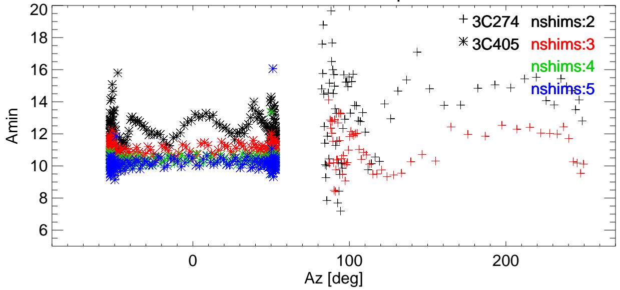
Az BmWidth vs Az for various shims. freq=9073 Pol:A RemoveBase.
