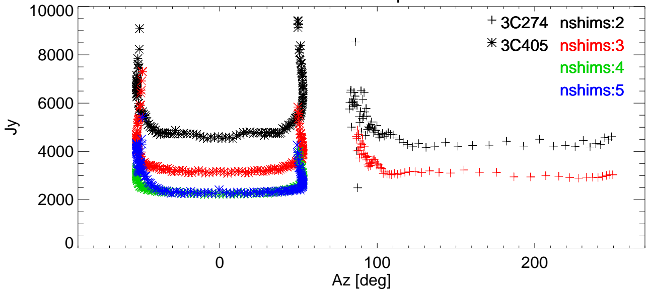
SEFD vs Az for various shims. freq=9073 Pol:A RemoveBase.
