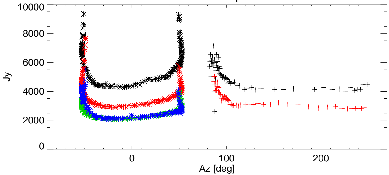
SEFD vs Az for various shims. freq=9073 Pol:B RemoveBase.
