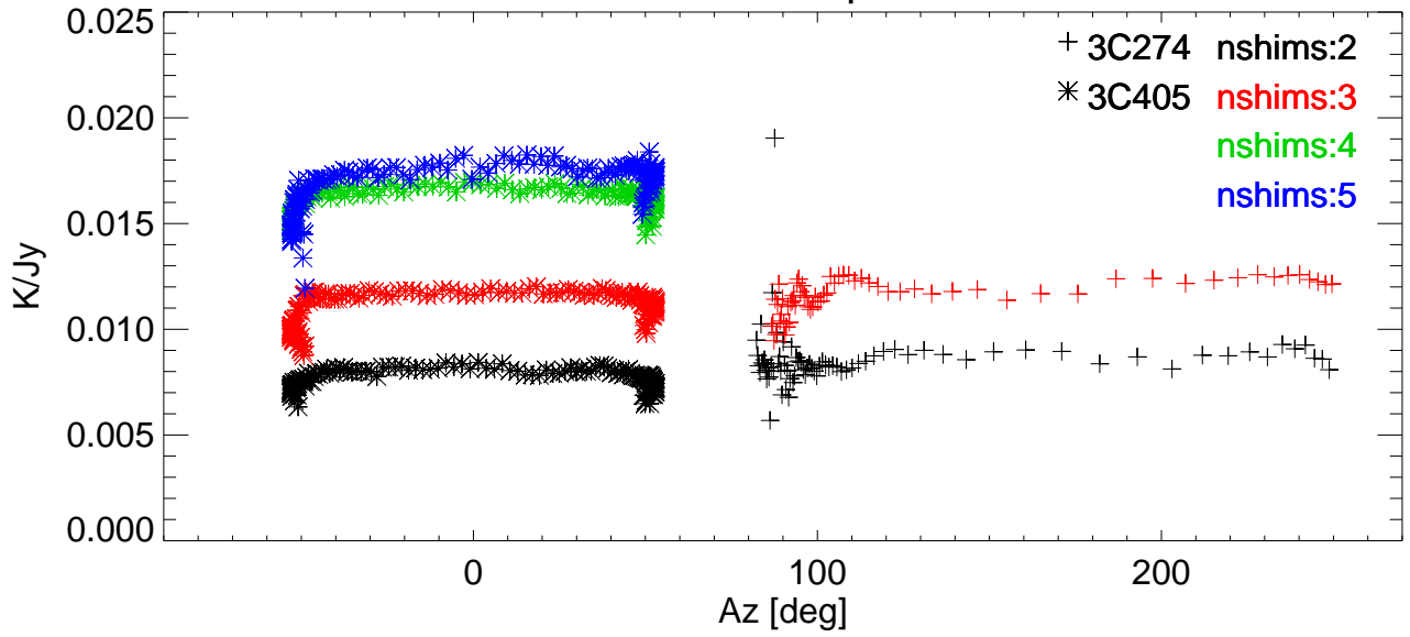
Gain vs Az for various shims. freq=9073 Pol:A RemoveBase.
