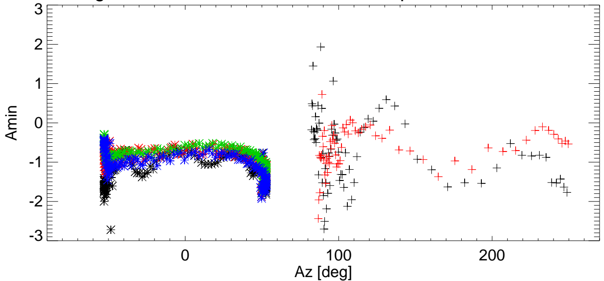
Az Pointing error vs Az for various shims. freq=9073 Pol:B RemoveBase.
