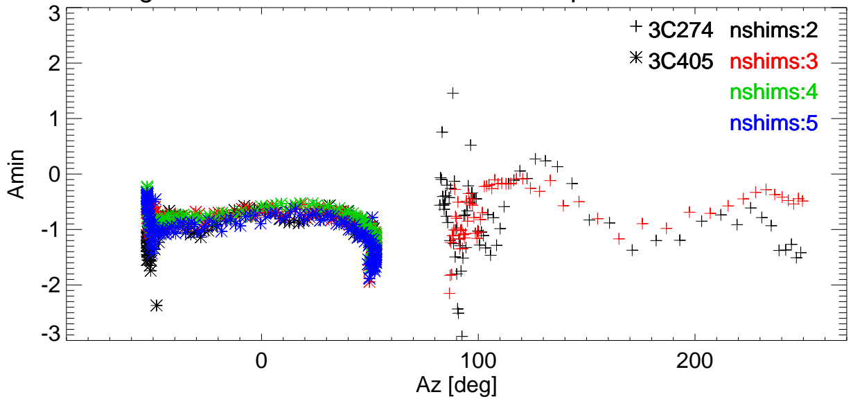
Az Pointing error vs Az for various shims. freq=9073 Pol:A RemoveBase.
