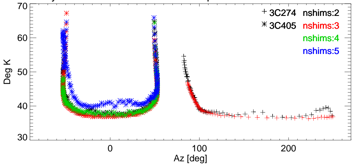
Tsys vs Az for various shims. freq=9073 Pol:A RemoveBase.
