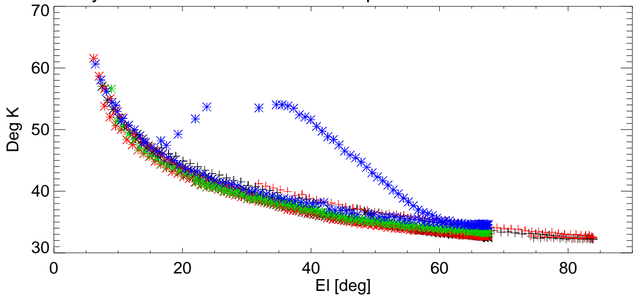
Tsys vs El for various shims. freq=8931 Pol:B RemoveBase.
