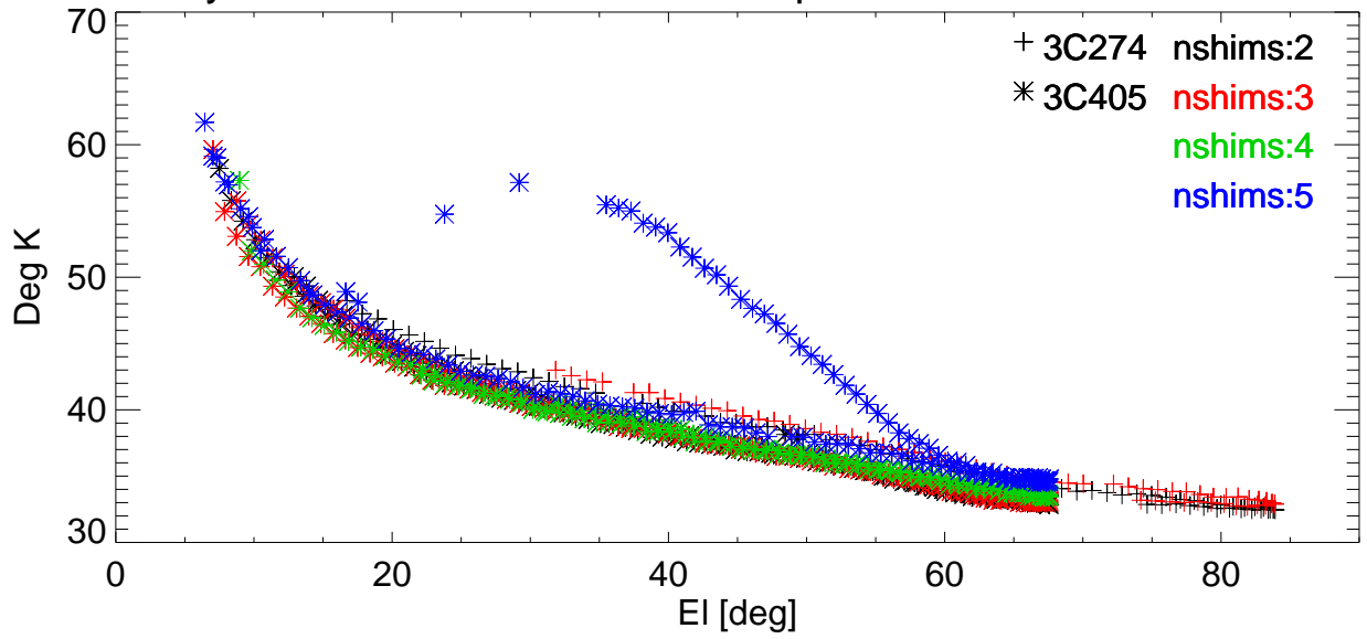
Tsys vs El for various shims. freq=8931 Pol:A RemoveBase.
