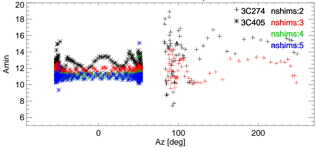
Az BmWidth vs Az for various shims. freq=8223 Pol:A RemoveBase.
