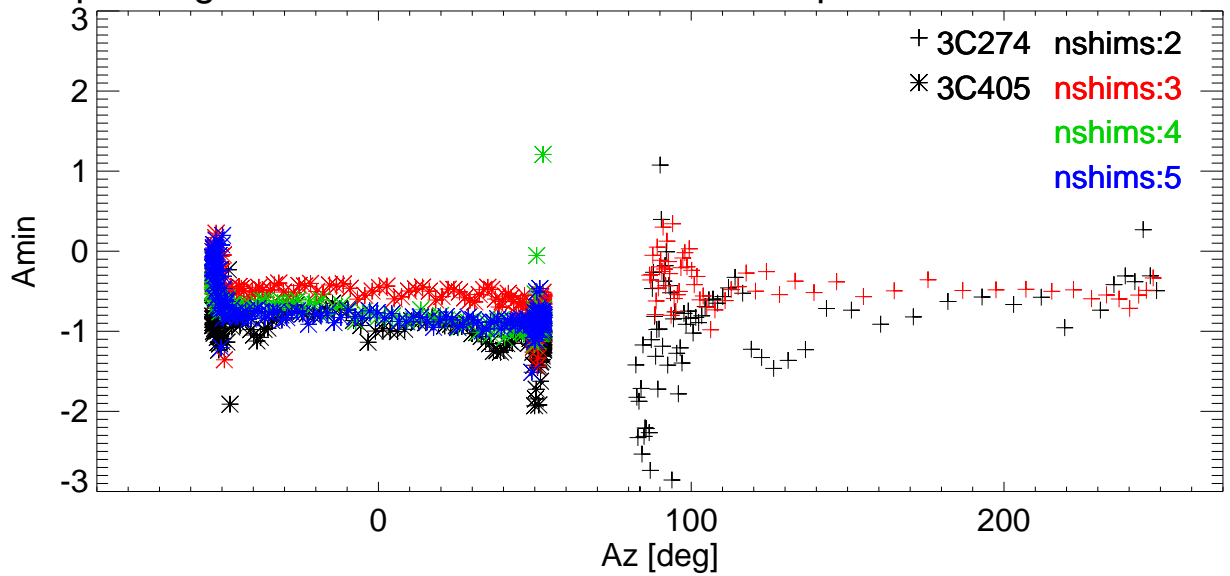
El pointing error vs Az for various shims. freq=8223 Pol:A RemoveBase.
