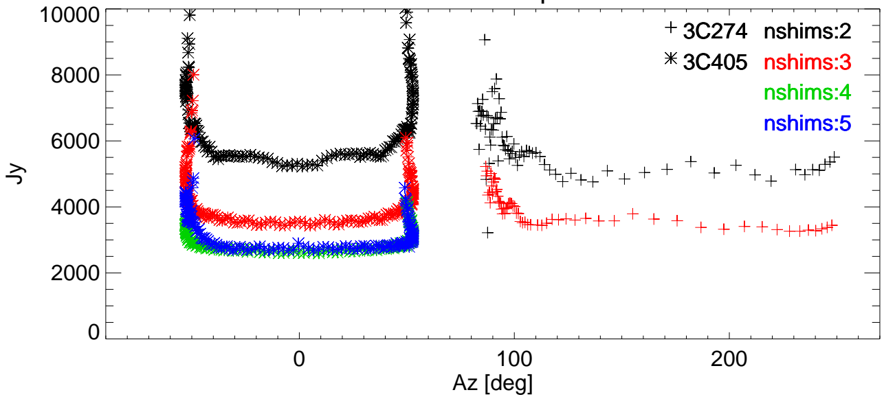
SEFD vs Az for various shims. freq=8223 Pol:A RemoveBase.
