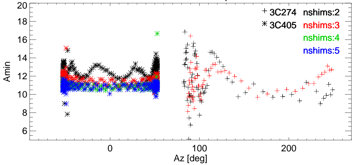
El BmWidth vs Az for various shims. freq=8223 Pol:A RemoveBase.
