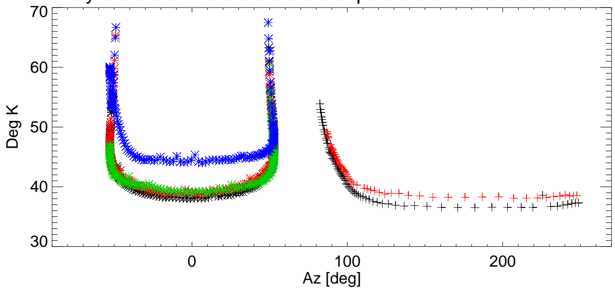
Tsys vs Az for various shims. freq=8223 Pol:B RemoveBase.
