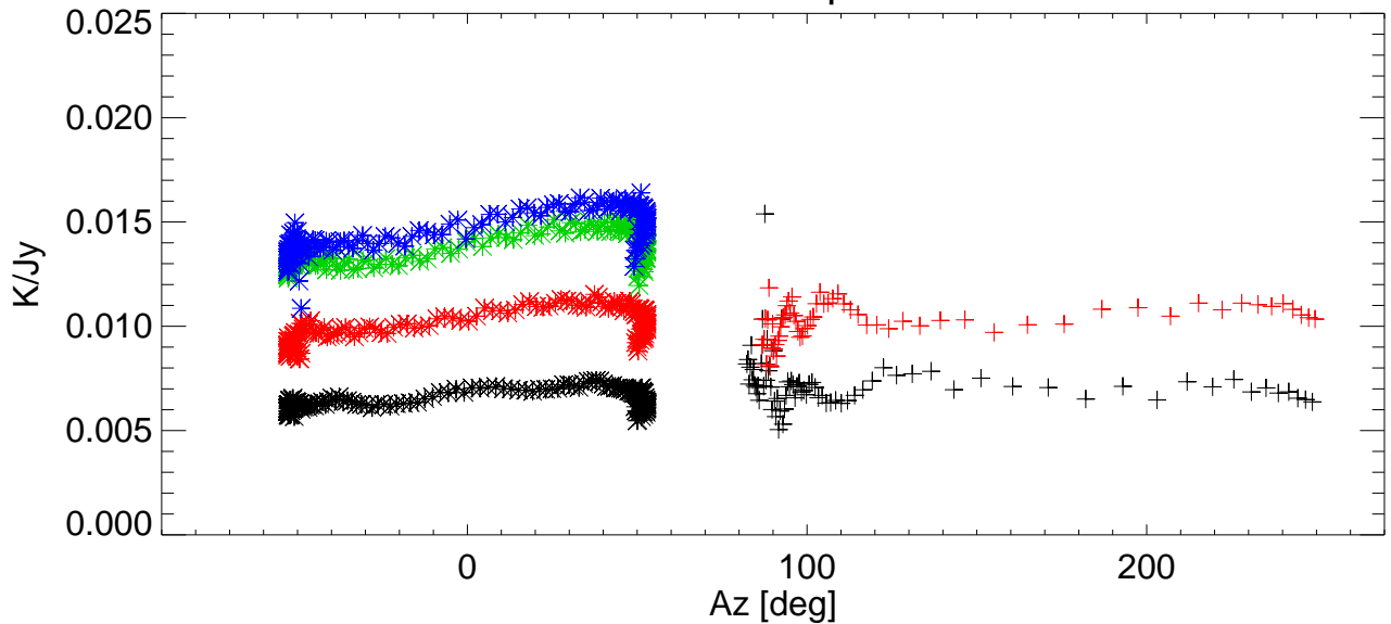
Gain vs Az for various shims. freq=8223 Pol:B RemoveBase.
