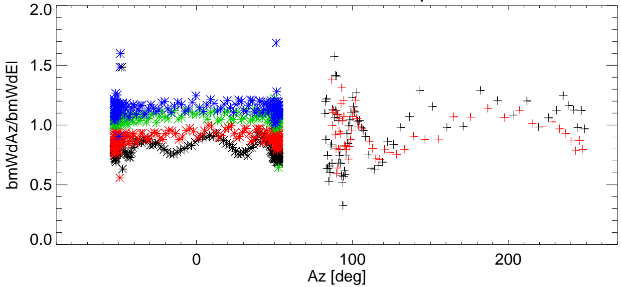
Az/EI BmWdRatio vs Az for various shims. freq=8223 Pol:B RemoveBase.
