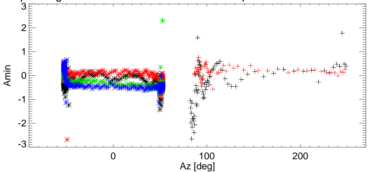
El pointing error vs Az for various shims. freq=8223 Pol:B RemoveBase.
