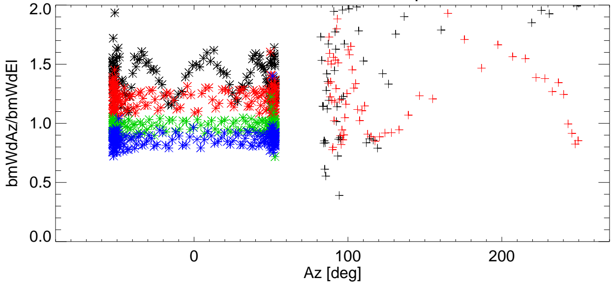
Az/EI BmWdRatio vs Az for various shims. freq=8223 Pol:B RemoveBase.
