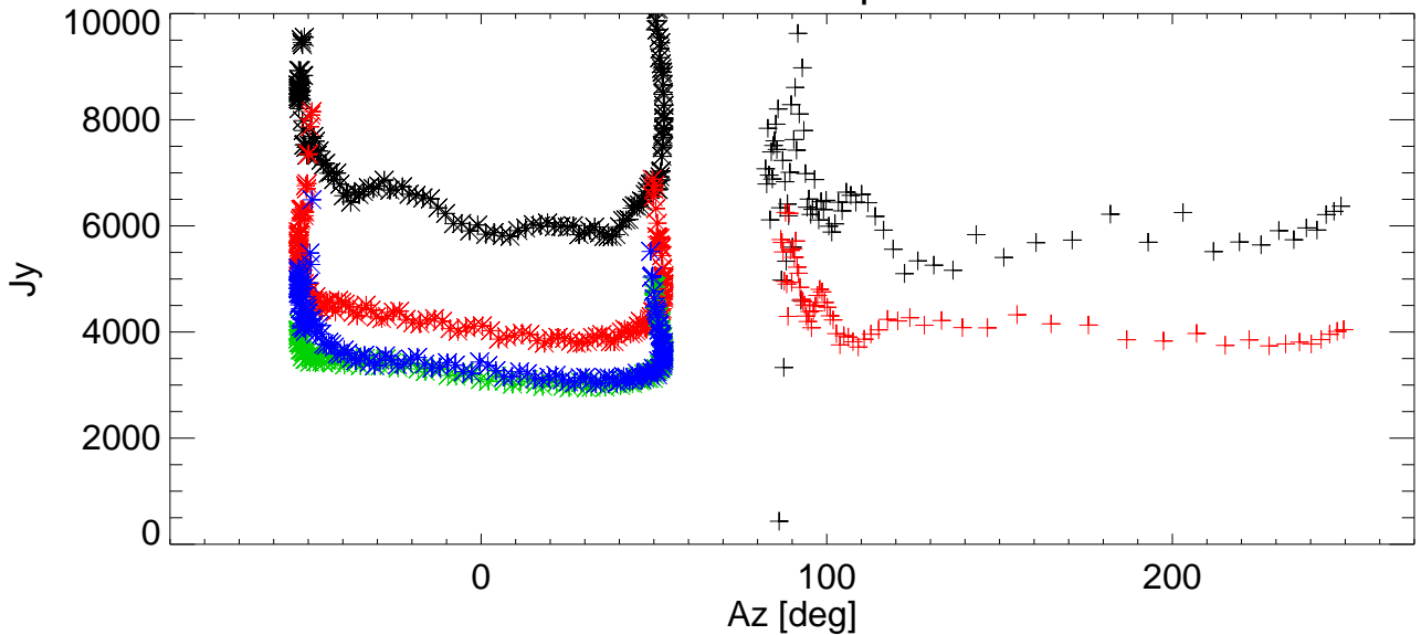
SEFD vs Az for various shims. freq=8223 Pol:B RemoveBase.
