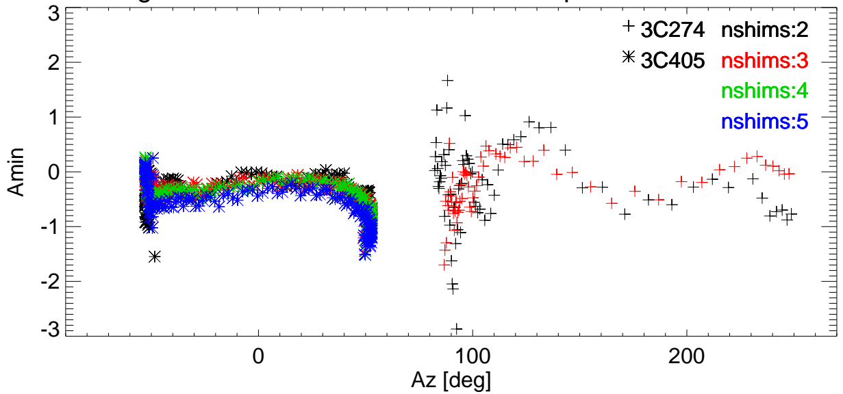
Az Pointing error vs Az for various shims. freq=8223 Pol:A RemoveBase.
