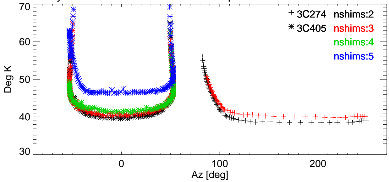
Tsys vs Az for various shims. freq=8223 Pol:A RemoveBase.
