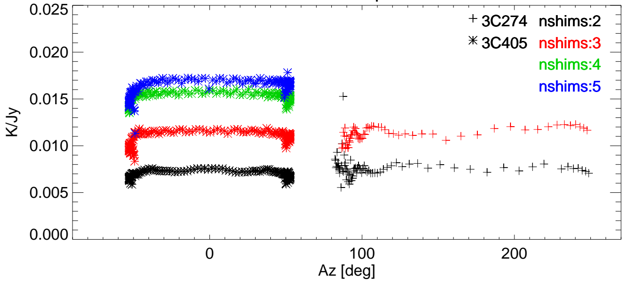
Gain vs Az for various shims. freq=8223 Pol:A RemoveBase.
