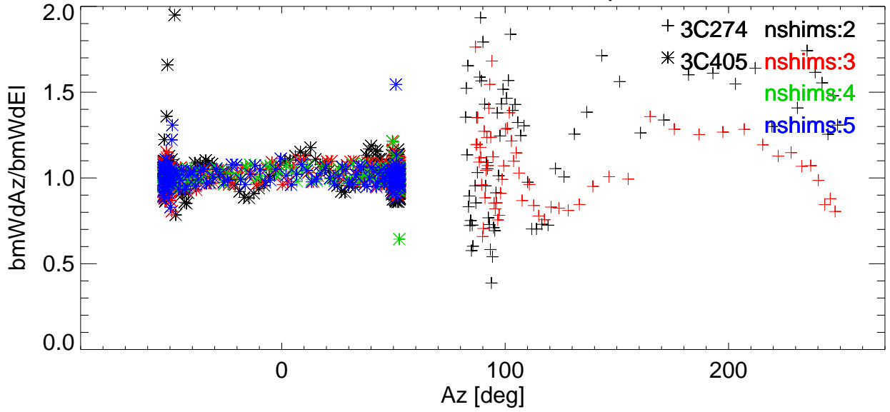
Az/EI BmWdRatio vs Az for various shims. freq=8223 Pol:A RemoveBase.
