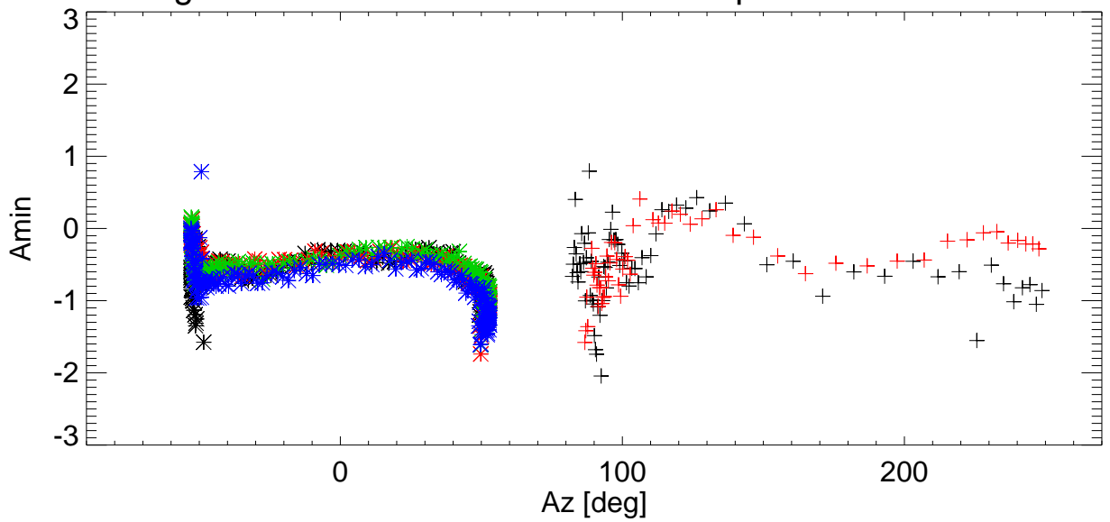
Az Pointing error vs Az for various shims. freq=8223 Pol:B RemoveBase.
