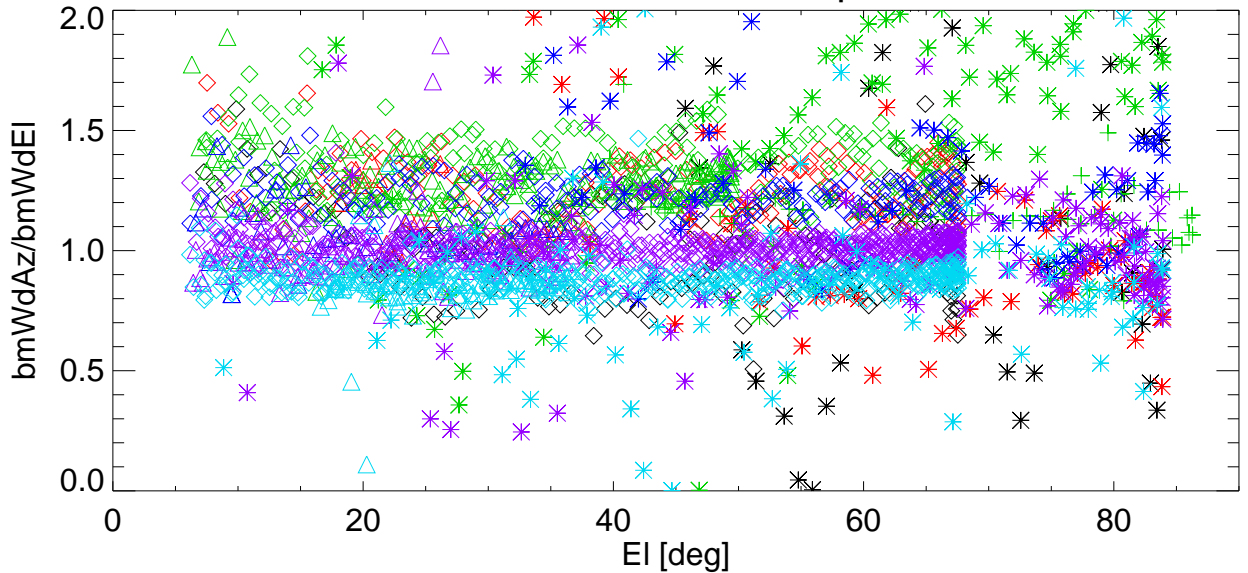
Az/EI BmWdRatio vs EI for various shims. freq=8931 Pol:B RemoveBase.
