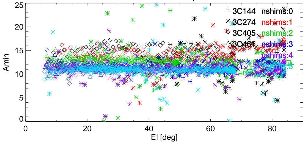
El BmWidth vs El for various shims. freq=8223 Pol:A RemoveBase.
