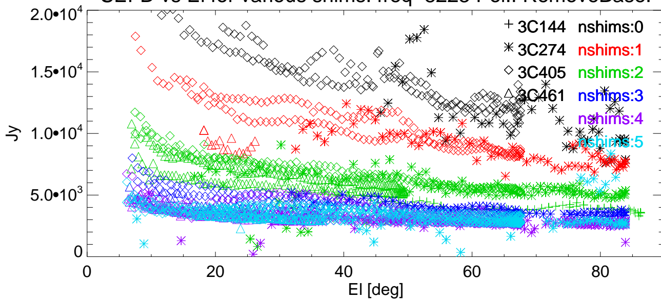
SEFD vs EI for various shims. freq=8223 Pol:A RemoveBase.
