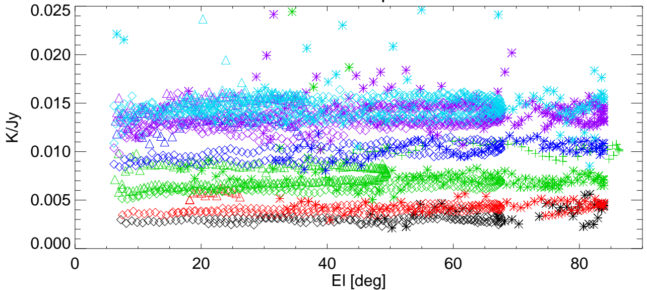
Gain vs EI for various shims. freq=8223 Pol:B RemoveBase.
