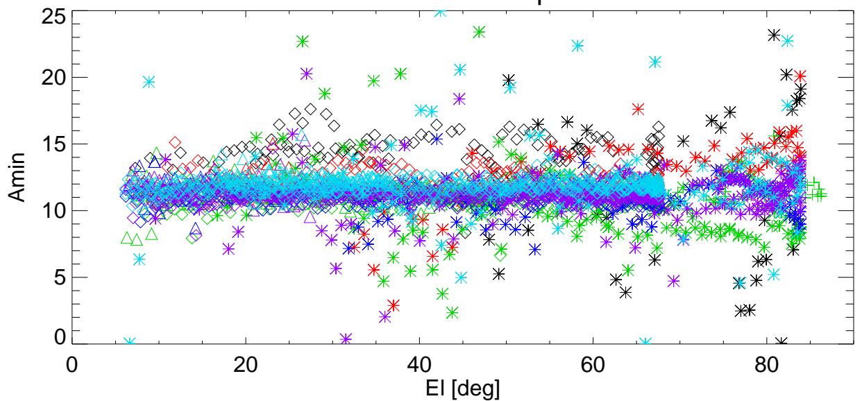
El BmWidth vs El for various shims. freq=8223 Pol:B RemoveBase.
