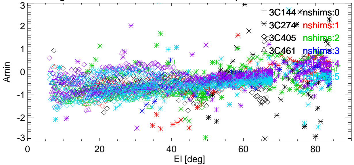
Az Pointing error vs EI for various shims. freq=8223 Pol:A RemoveBase.
