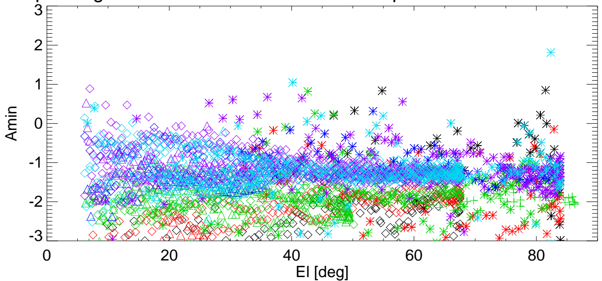
El pointing error vs El for various shims. freq=8223 Pol:B RemoveBase.
