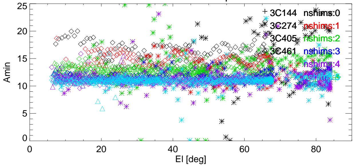
Az BmWidth vs EI for various shims. freq=8223 Pol:A RemoveBase.
