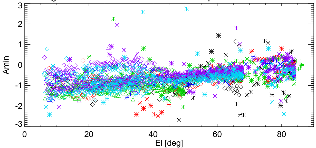
Az Pointing error vs EI for various shims. freq=8223 Pol:B RemoveBase.
