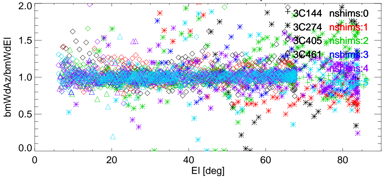
Az/EI BmWdRatio vs EI for various shims. freq=8223 Pol:A RemoveBase.
