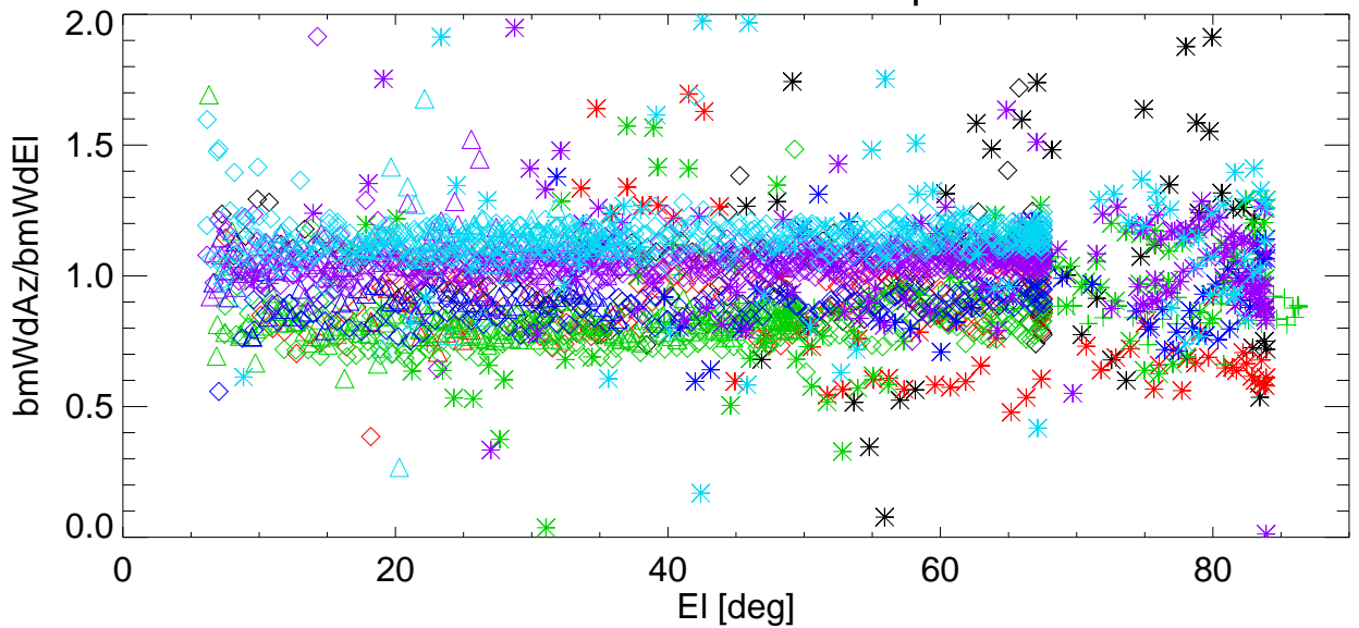
Az/EI BmWdRatio vs EI for various shims. freq=8223 Pol:B RemoveBase.
