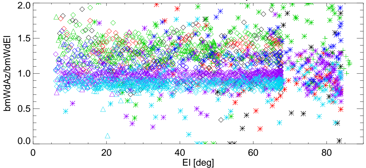
Az/EI BmWdRatio vs EI for various shims. freq=8223 Pol:B RemoveBase.
