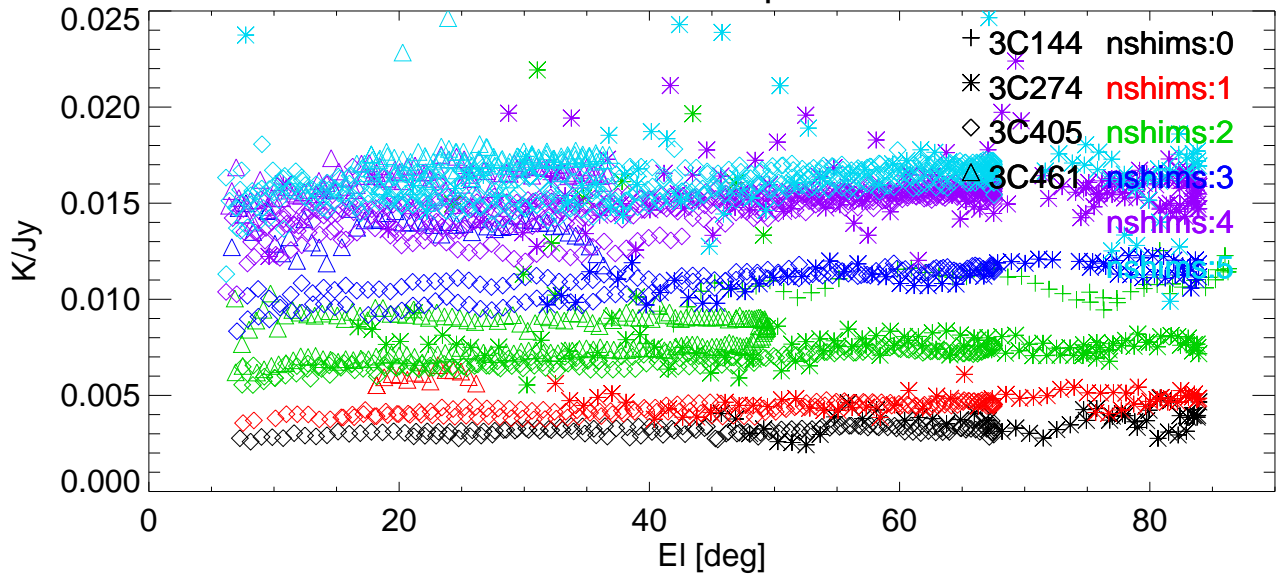
Gain vs EI for various shims. freq=8223 Pol:A RemoveBase.
