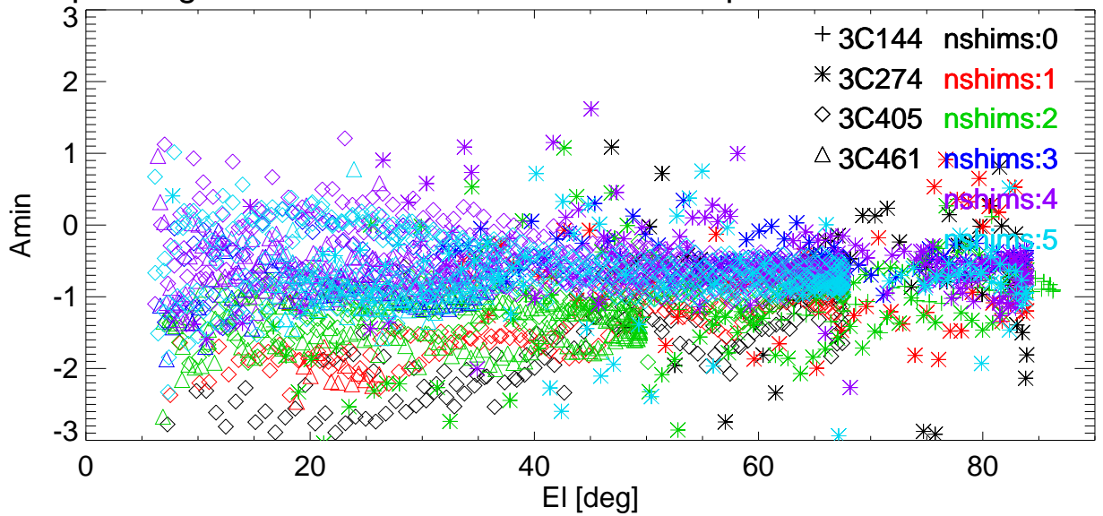
El pointing error vs El for various shims. freq=8223 Pol:A RemoveBase.
