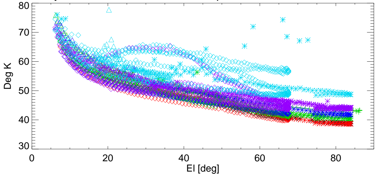
Tsys vs EI for various shims. freq=8223 Pol:B RemoveBase.
