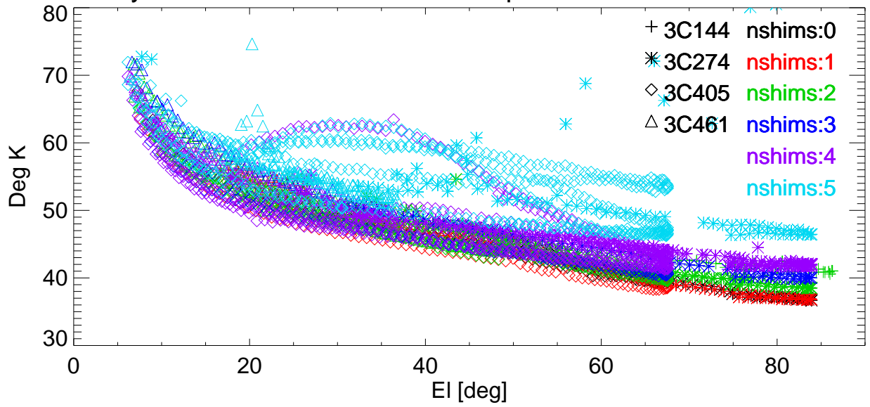
Tsys vs EI for various shims. freq=8223 Pol:A RemoveBase.
