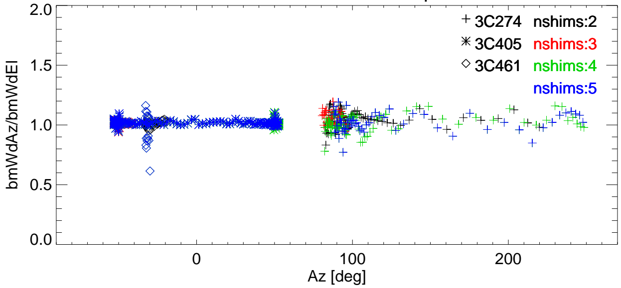
Az/EI BmWdRatio vs Az for various shims. freq=3272 Pol:A RemoveBase.
