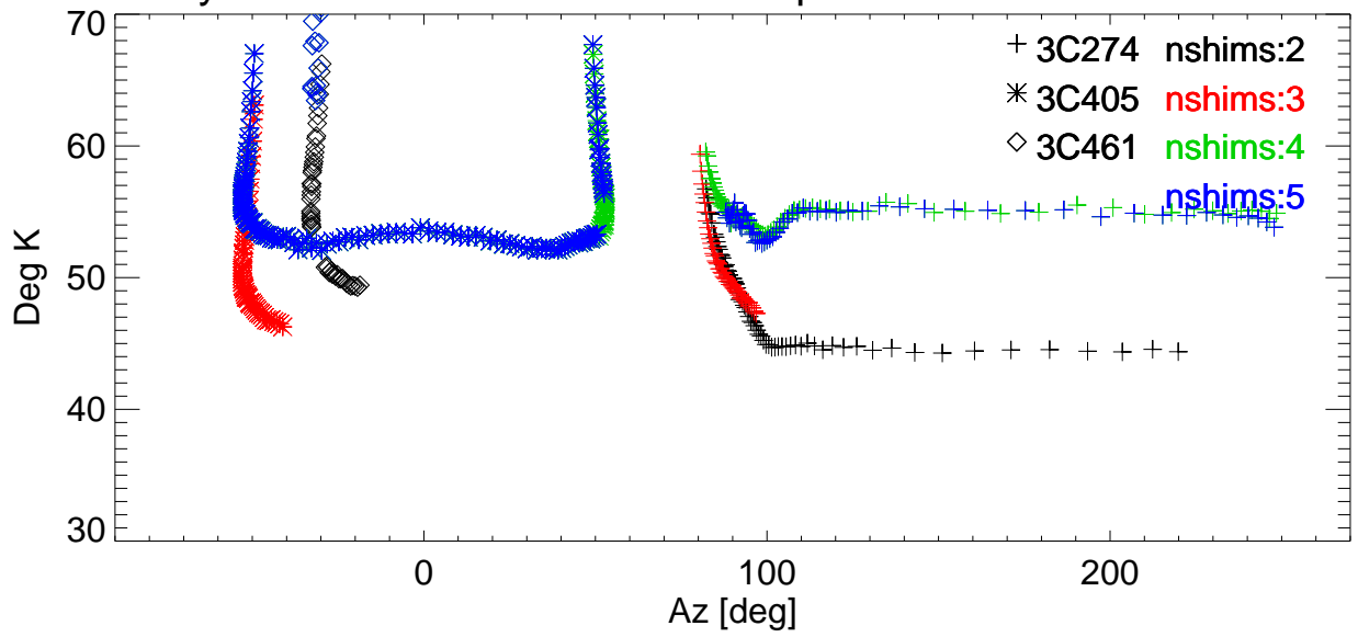
Tsys vs Az for various shims. freq=3272 Pol:A RemoveBase.
