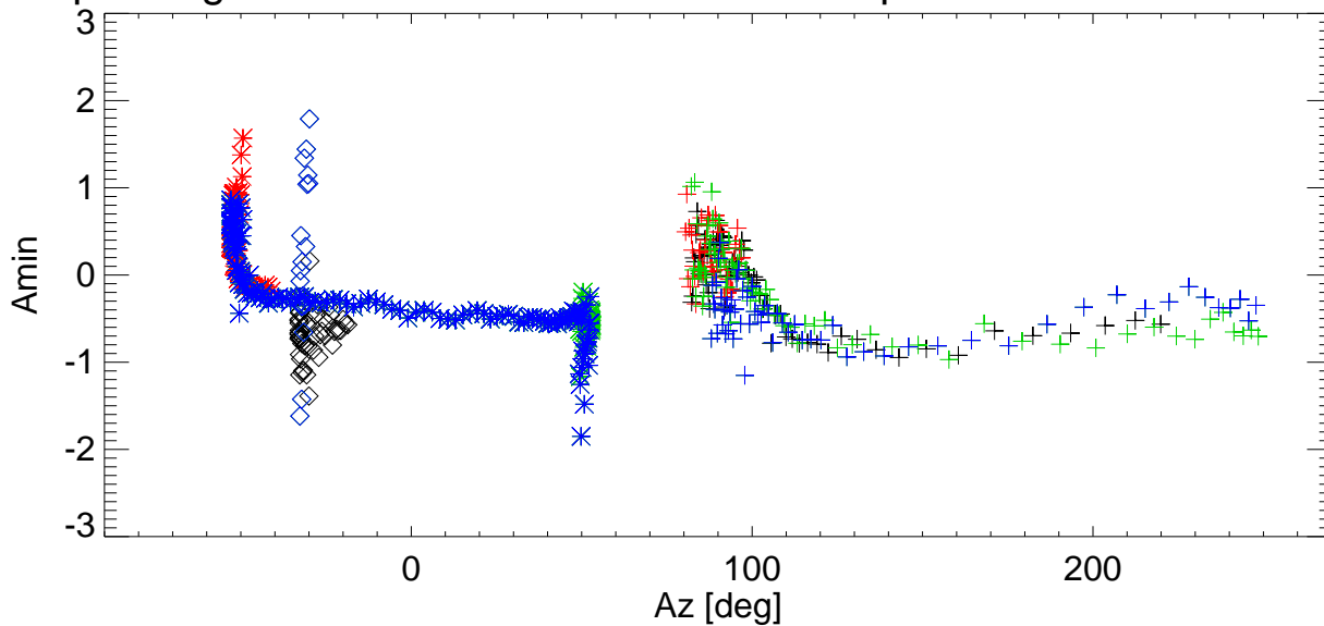
El pointing error vs Az for various shims. freq=3272 Pol:B RemoveBase.
