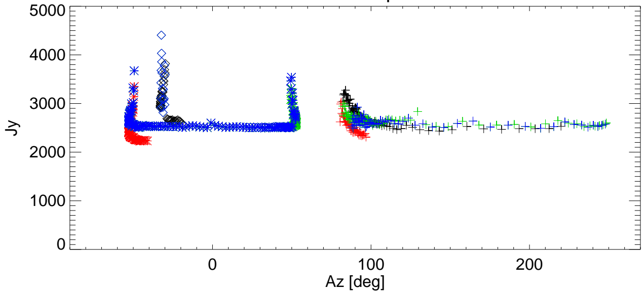
SEFD vs Az for various shims. freq=3272 Pol:B RemoveBase.
