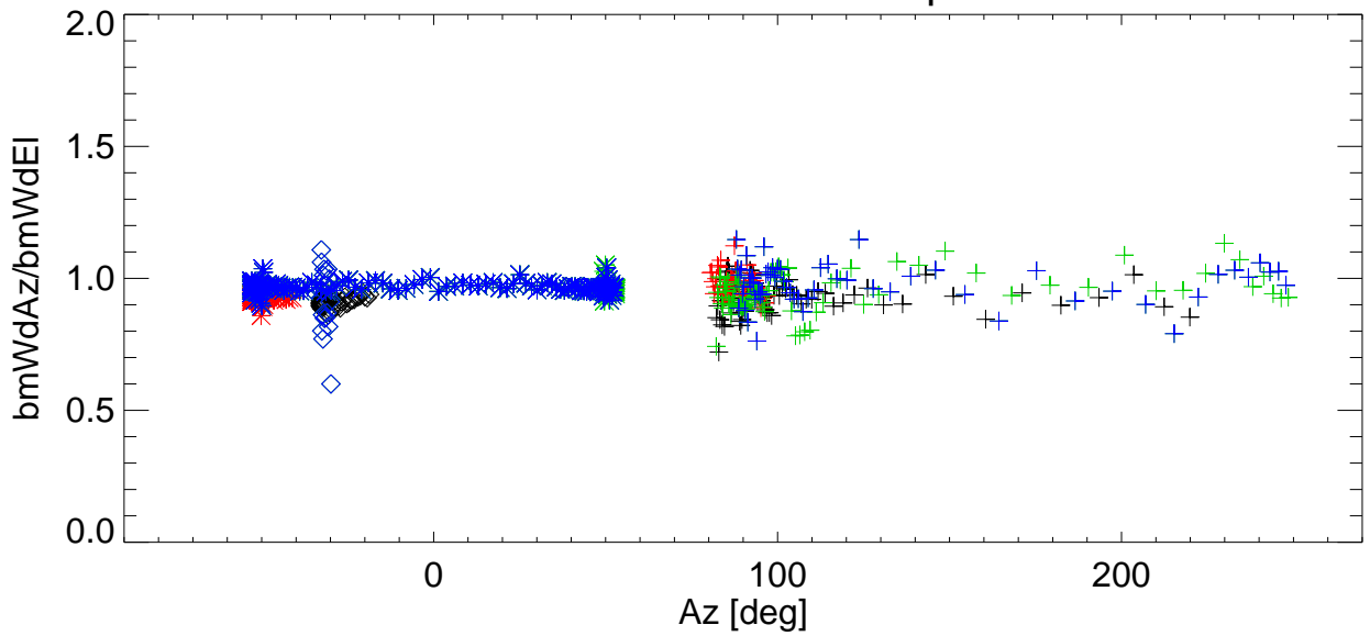
Az/EI BmWdRatio vs Az for various shims. freq=3272 Pol:B RemoveBase.
