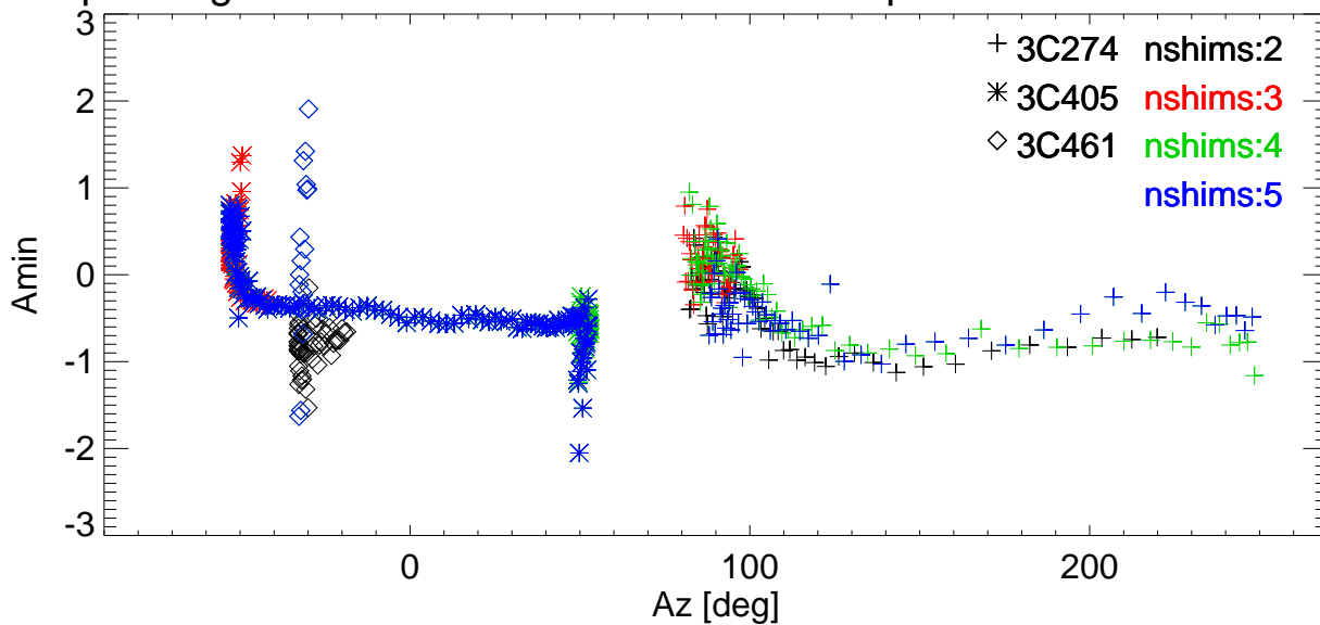
El pointing error vs Az for various shims. freq=3272 Pol:A RemoveBase.
