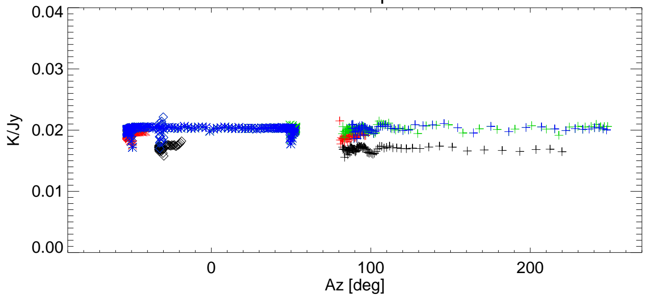
Gain vs Az for various shims. freq=3272 Pol:B RemoveBase.
