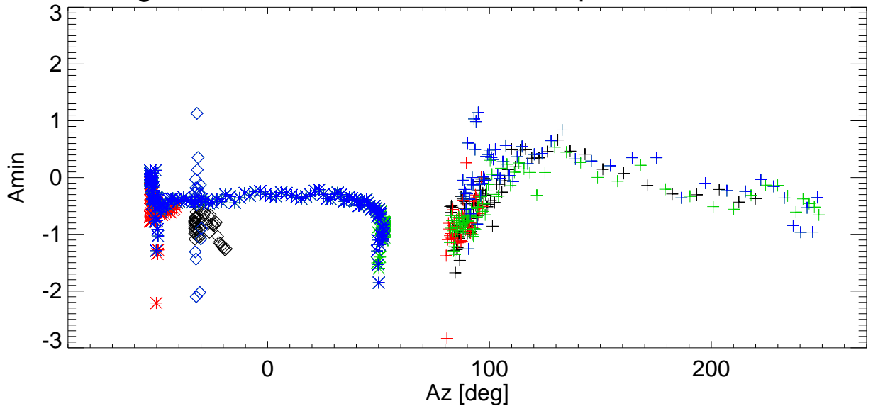
Az Pointing error vs Az for various shims. freq=3272 Pol:B RemoveBase.
