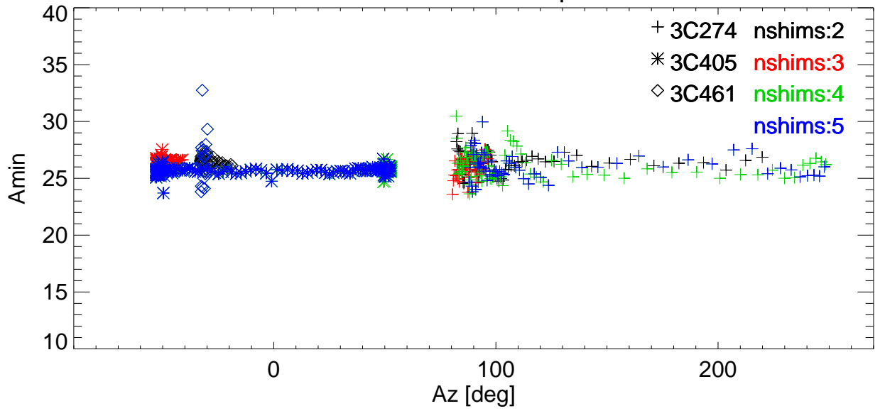
El BmWidth vs Az for various shims. freq=3272 Pol:A RemoveBase.
