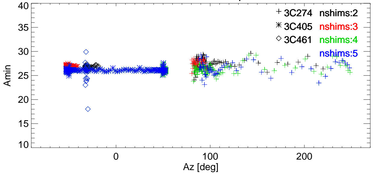
Az BmWidth vs Az for various shims. freq=3272 Pol:A RemoveBase.
