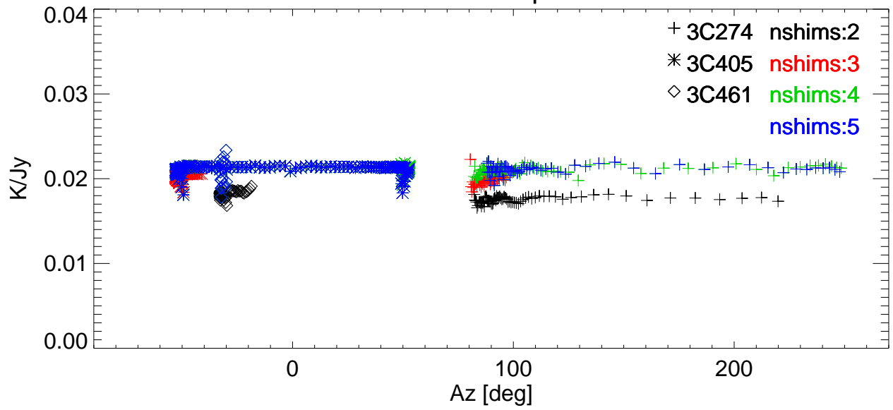
Gain vs Az for various shims. freq=3272 Pol:A RemoveBase.
