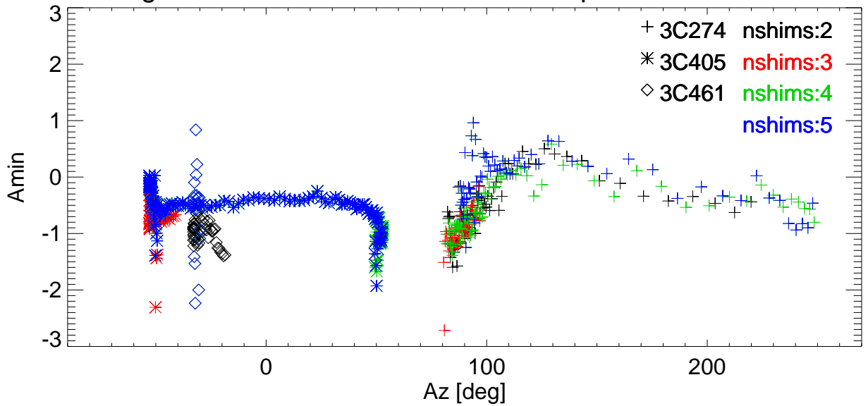
Az Pointing error vs Az for various shims. freq=3272 Pol:A RemoveBase.
