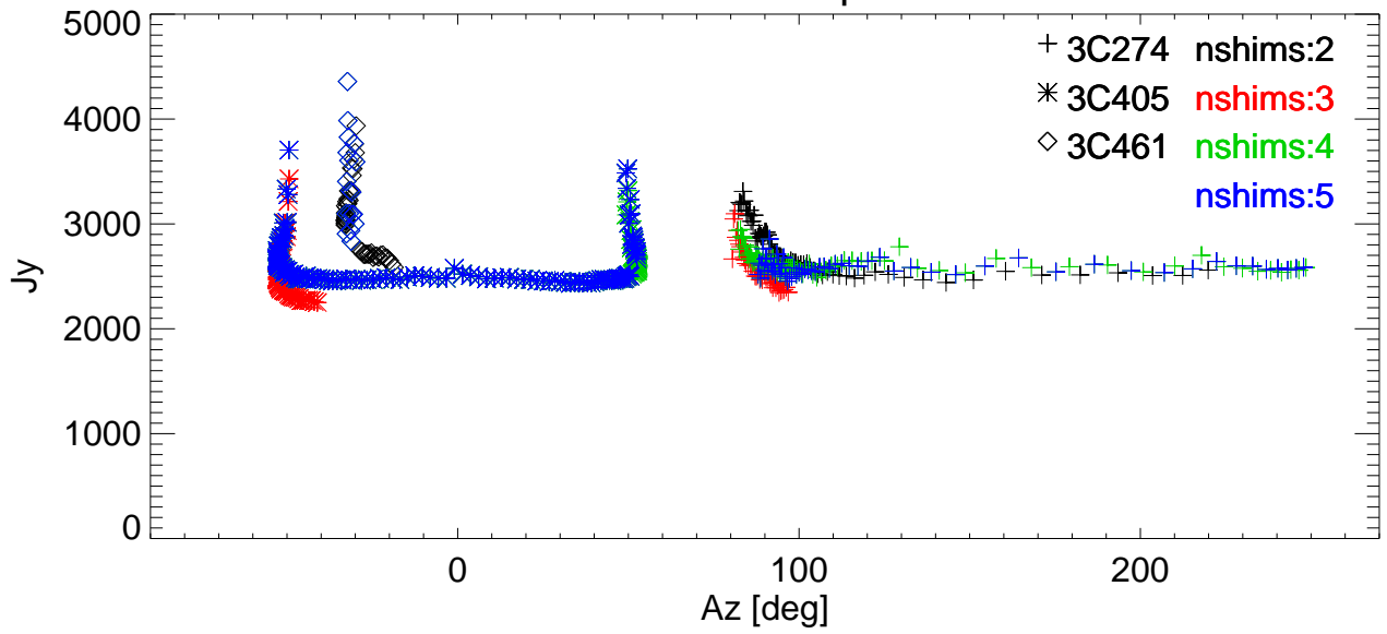
SEFD vs Az for various shims. freq=3272 Pol:A RemoveBase.
