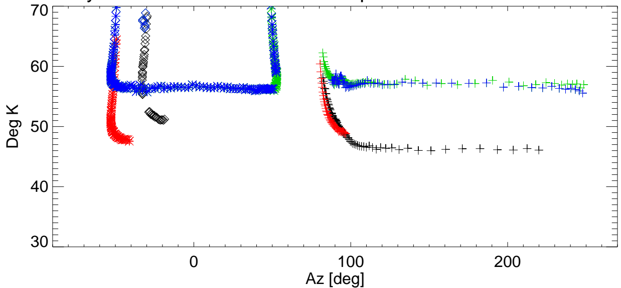
Tsys vs Az for various shims. freq=3272 Pol:B RemoveBase.
