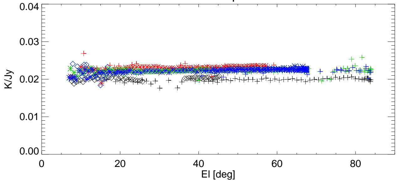
Gain vs EI for various shims. freq=2988 Pol:B RemoveBase.
