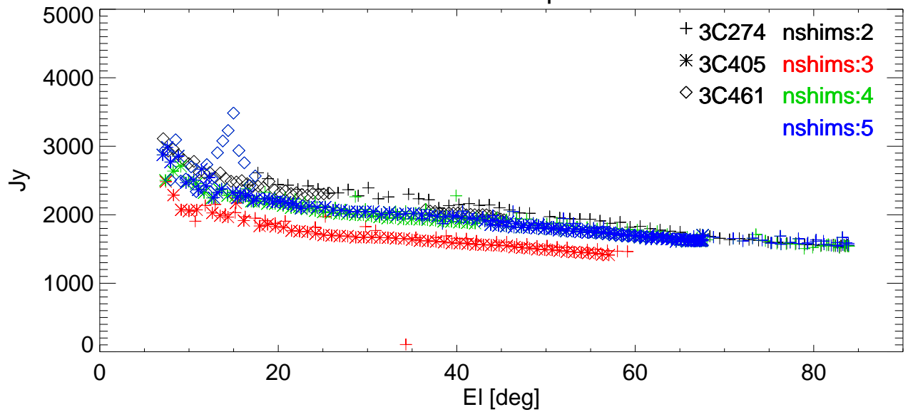
SEFD vs EI for various shims. freq=2988 Pol:A RemoveBase.
