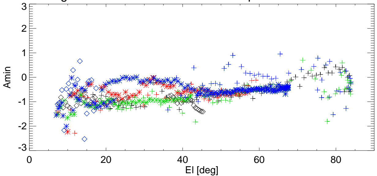
Az Pointing error vs EI for various shims. freq=2988 Pol:B RemoveBase.
