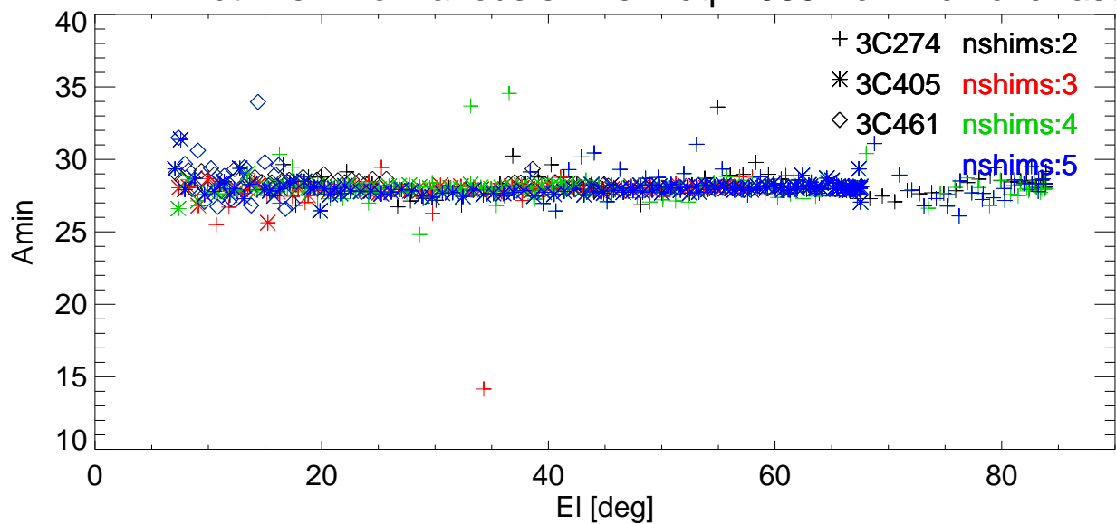
El BmWidth vs El for various shims. freq=2988 Pol:A RemoveBase.
