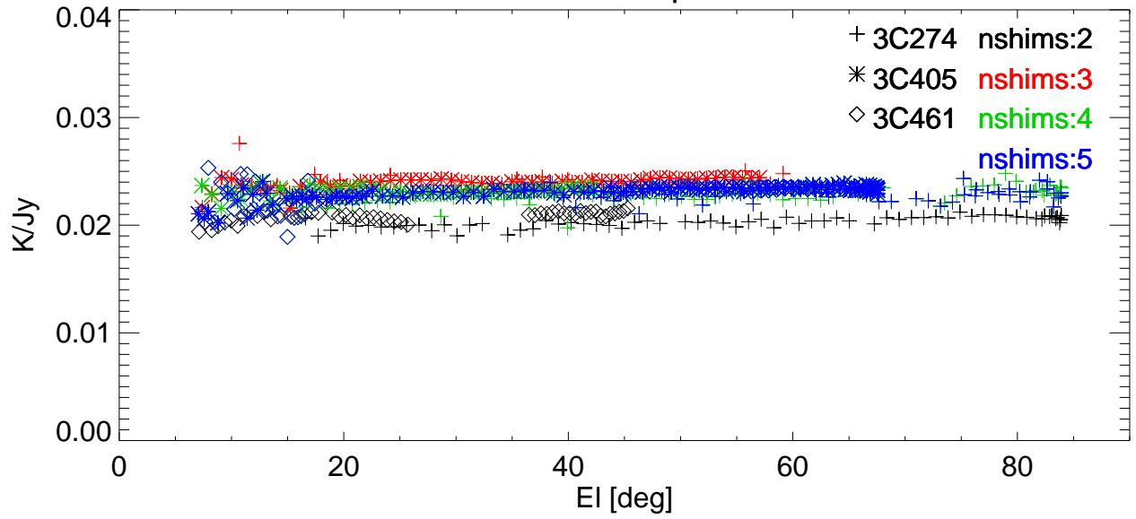
Gain vs EI for various shims. freq=2988 Pol:A RemoveBase.
