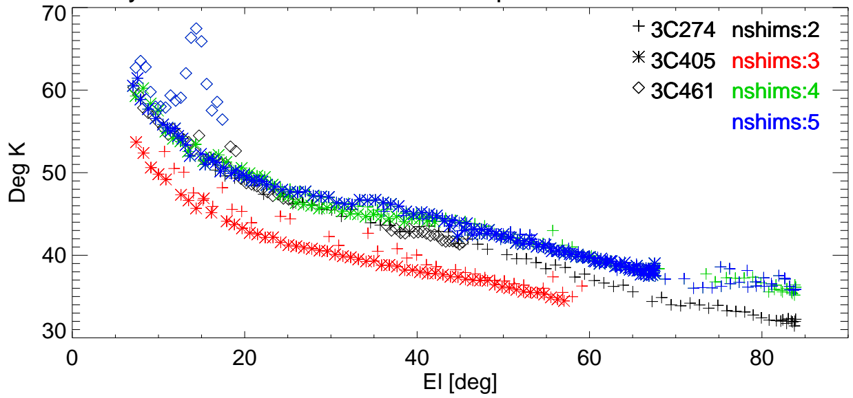
Tsys vs EI for various shims. freq=2988 Pol:A RemoveBase.
