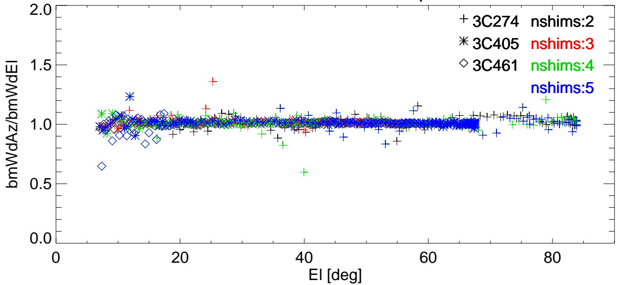
Az/EI BmWdRatio vs EI for various shims. freq=2988 Pol:A RemoveBase.
