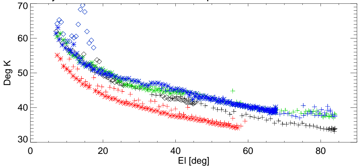
Tsys vs EI for various shims. freq=2988 Pol:B RemoveBase.
