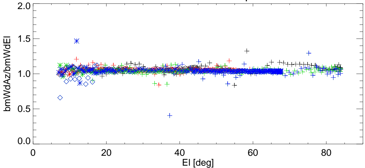
Az/EI BmWdRatio vs EI for various shims. freq=2988 Pol:B RemoveBase.
