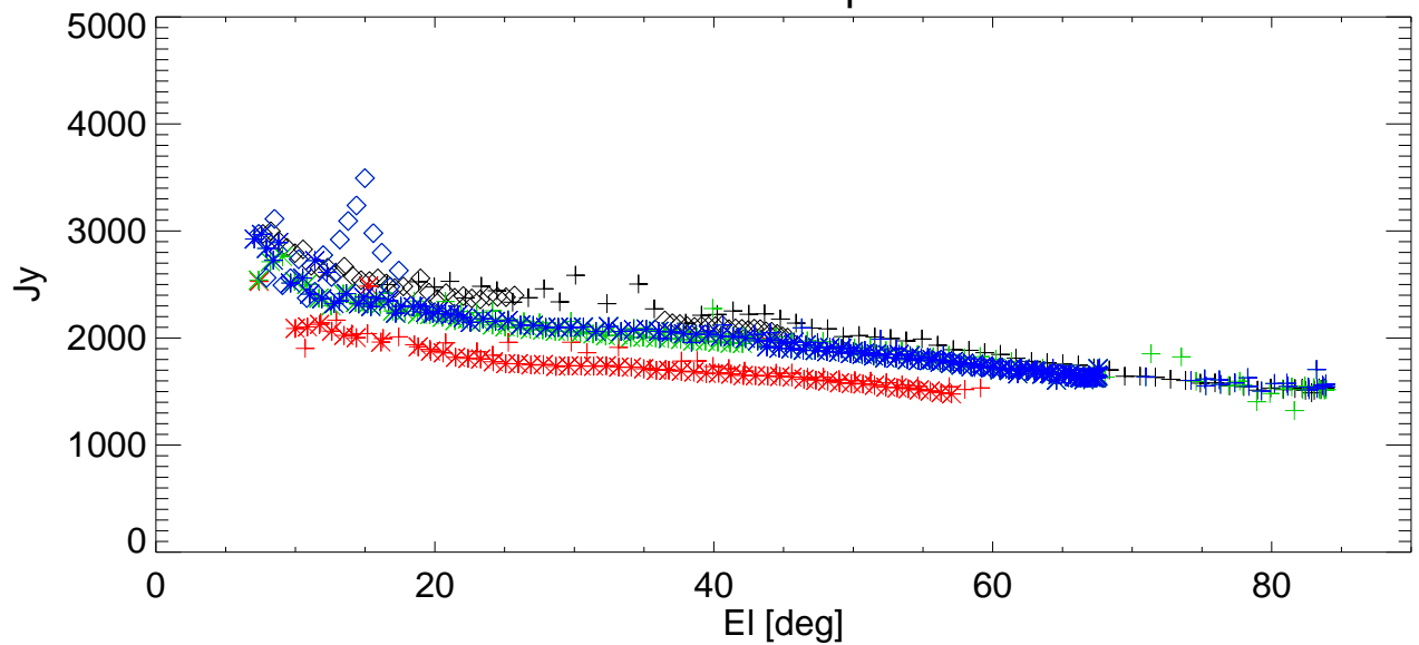
SEFD vs EI for various shims. freq=2988 Pol:B RemoveBase.
