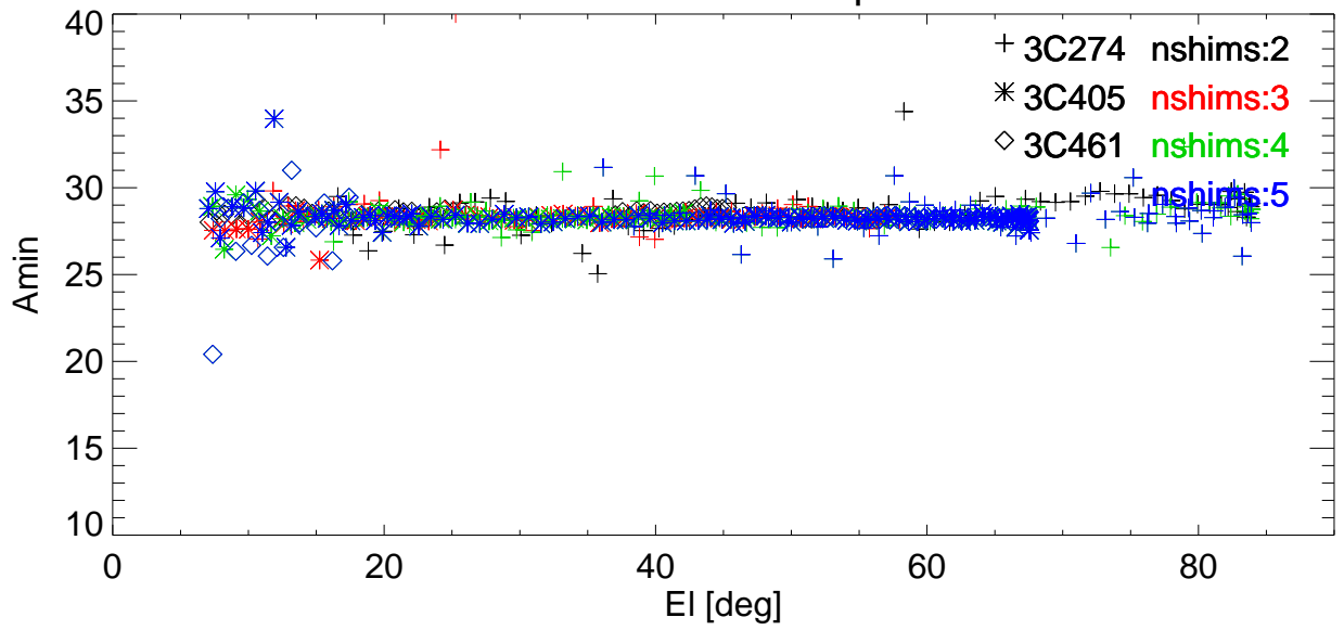
Az BmWidth vs EI for various shims. freq=2988 Pol:A RemoveBase.
