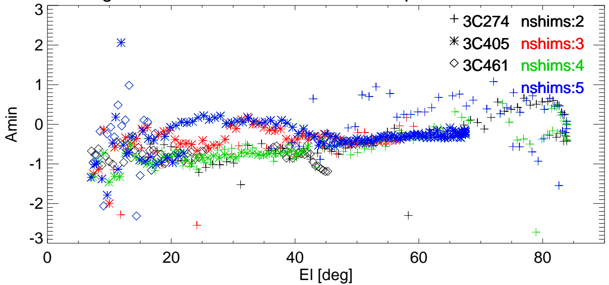
Az Pointing error vs EI for various shims. freq=2988 Pol:A RemoveBase.
