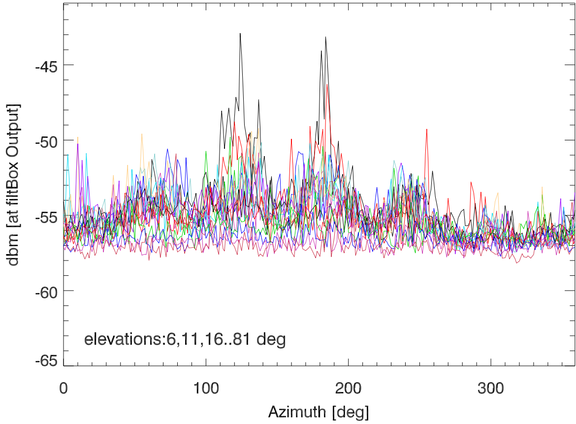
17may23 azswings. TotPwr 5075- 5600 MHz
