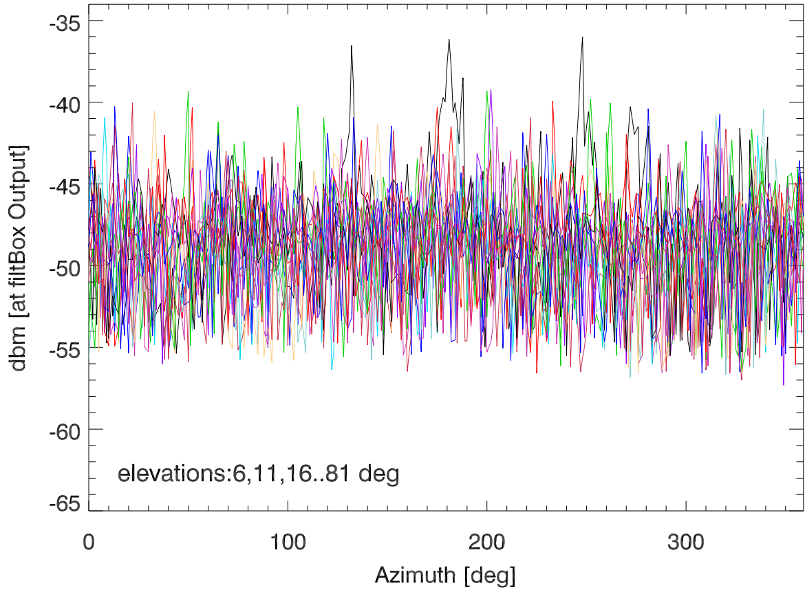
17may23 azswings. TotPwr 3550- 3700 MHz
