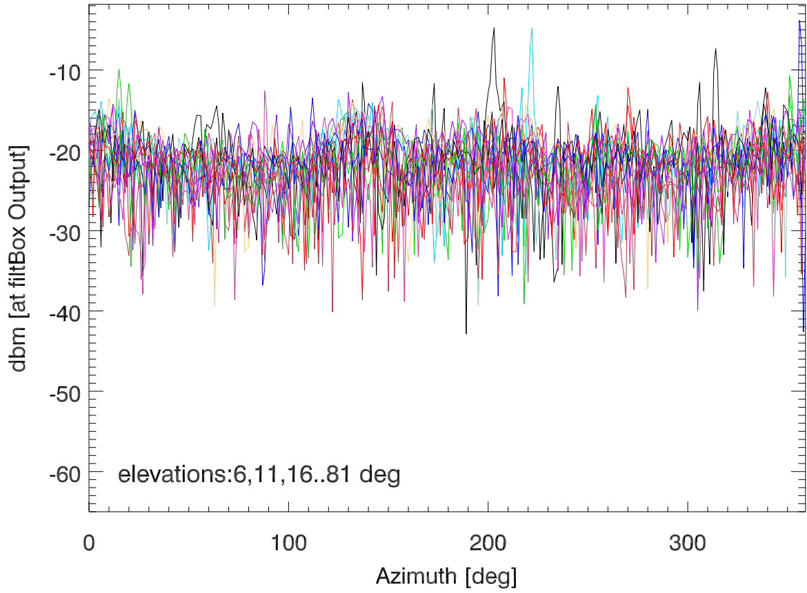
17may23 azswings. TotPwr 2500- 2700 MHz
