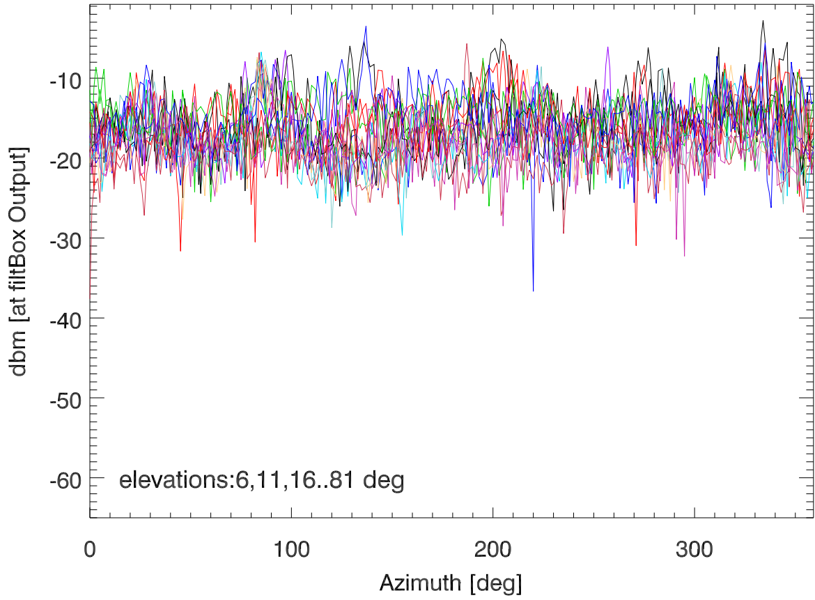
17may23 azswings. TotPwr 2340- 2355 MHz
