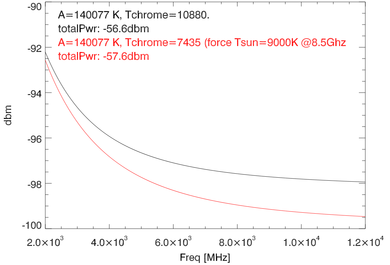
computed power (1MHz rbw) from the sun vs freq
