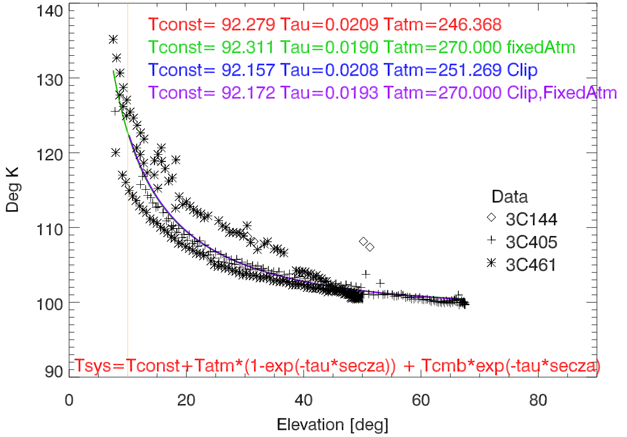
Tsys vs El. bandcfr:9073 MHz
