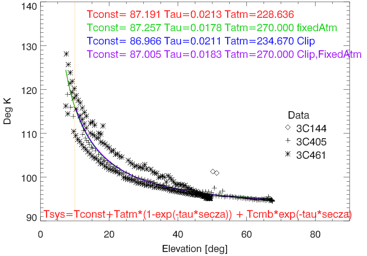
Tsys vs El. bandcfr:8505 MHz
