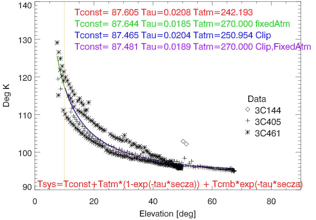
Tsys vs El. bandcfr:8789 MHz
