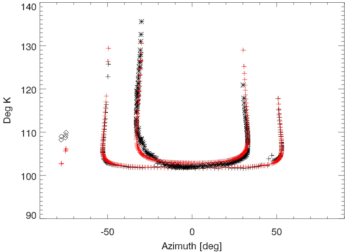
Tsys vs Az. bandcfr:8931 MHz
