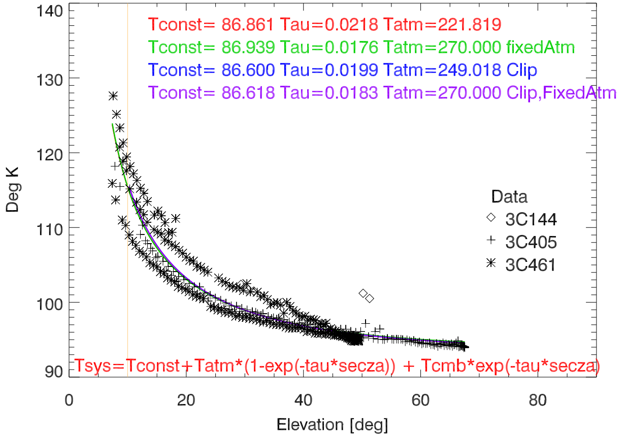
Tsys vs El. bandcfr:8647 MHz
