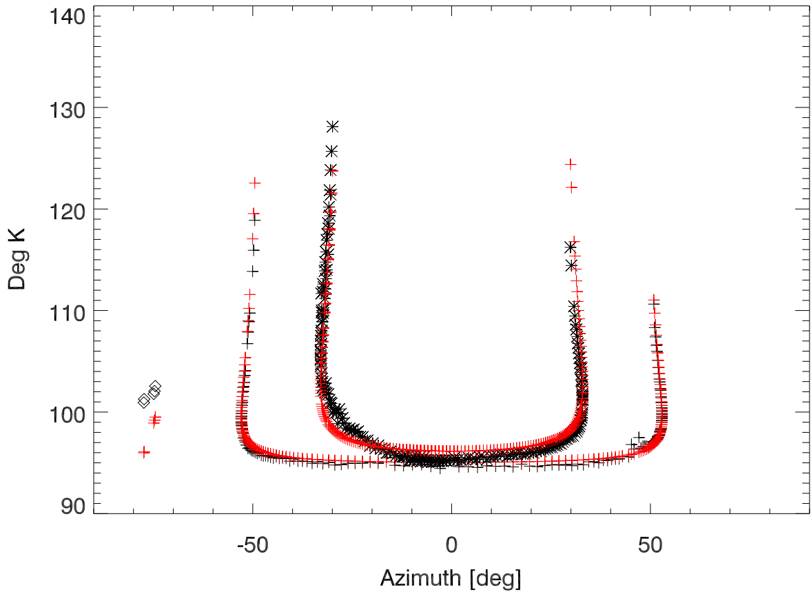
Tsys vs Az. bandcfr:8505 MHz
