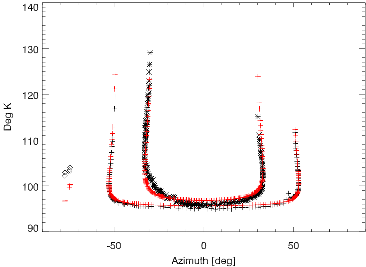
Tsys vs Az. bandcfr:8789 MHz
