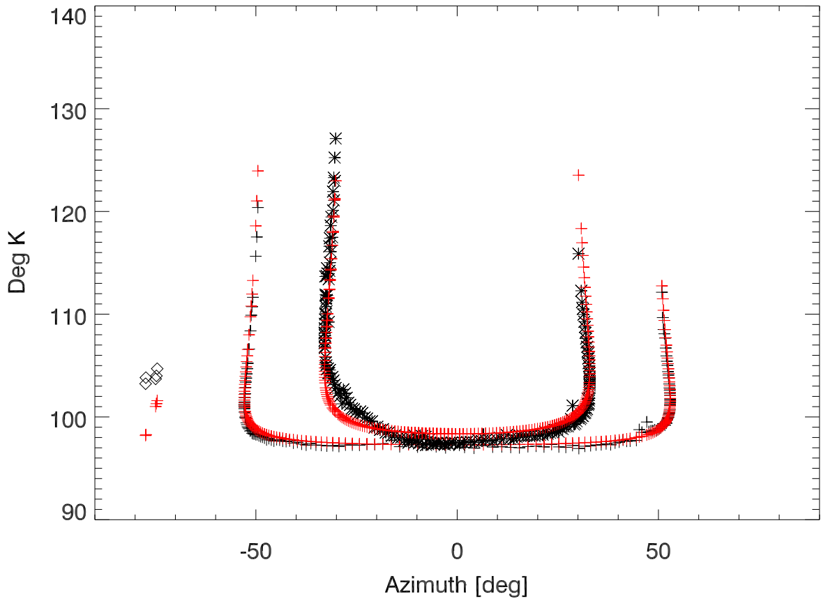
Tsys vs Az. bandcfr:8223 MHz
