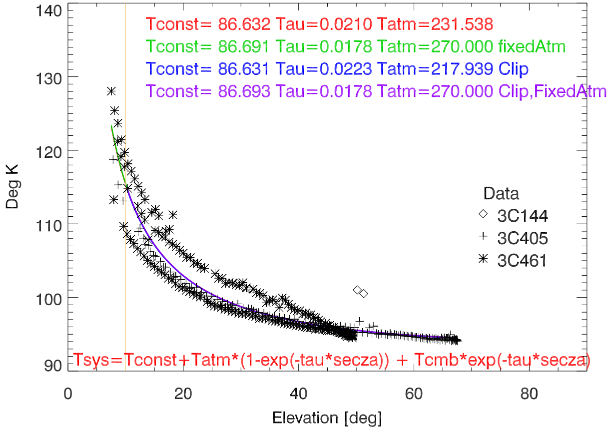
Tsys vs El. bandcfr:8363 MHz
