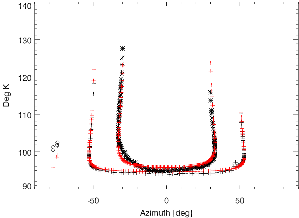
Tsys vs Az. bandcfr:8647 MHz
