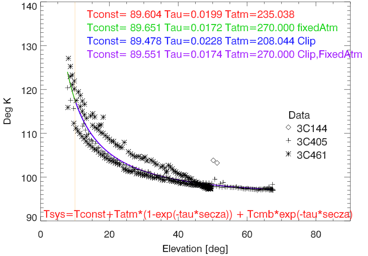
Tsys vs El. bandcfr:8223 MHz
