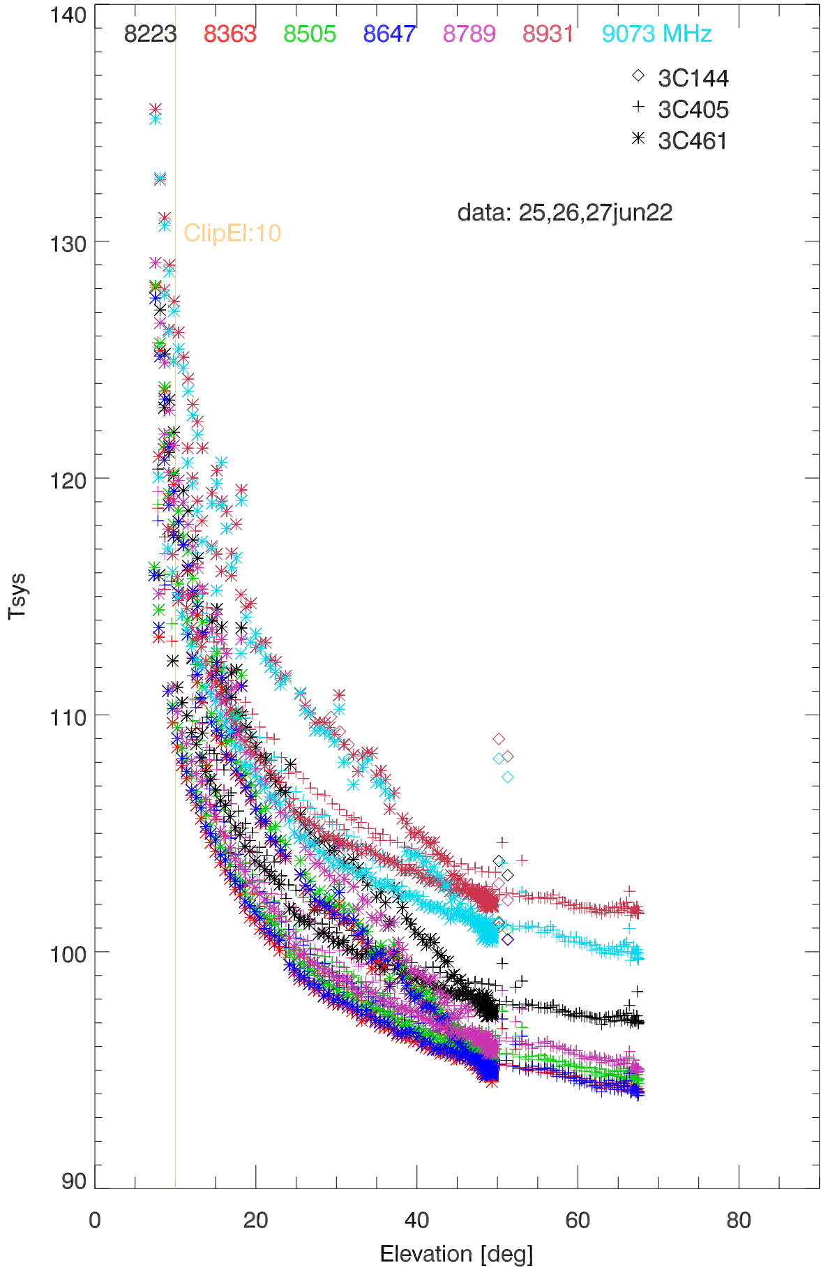
jun22 xband crosses. Tsys vs el by frequency band (after clipping)
