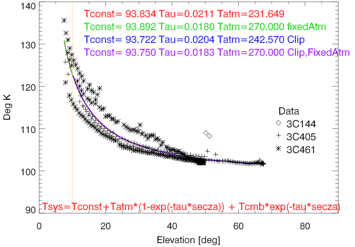
Tsys vs El. bandcfr:8931 MHz
