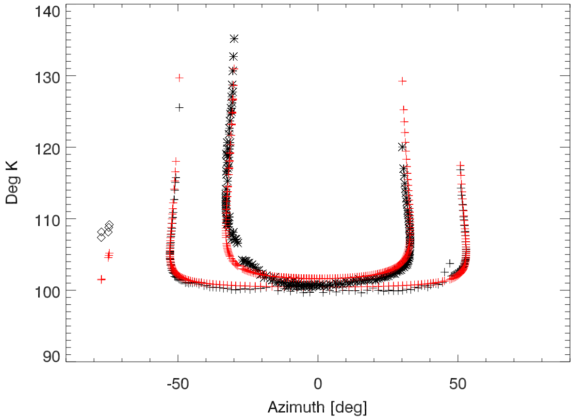
Tsys vs Az. bandcfr:9073 MHz
