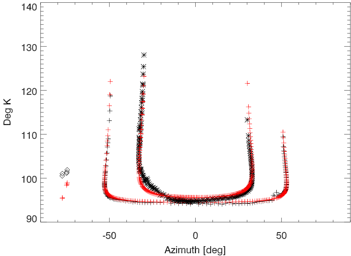
Tsys vs Az. bandcfr:8363 MHz
