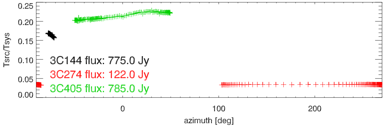
04-06apr22 sband crosses. Tsrc/Tsys vs az CFR:2270.0MHz
