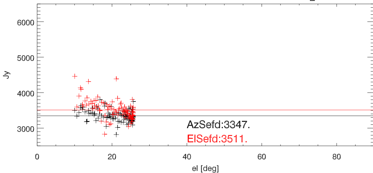
12m sband model3A 1d fits. SEFD from src: Pictor_A
