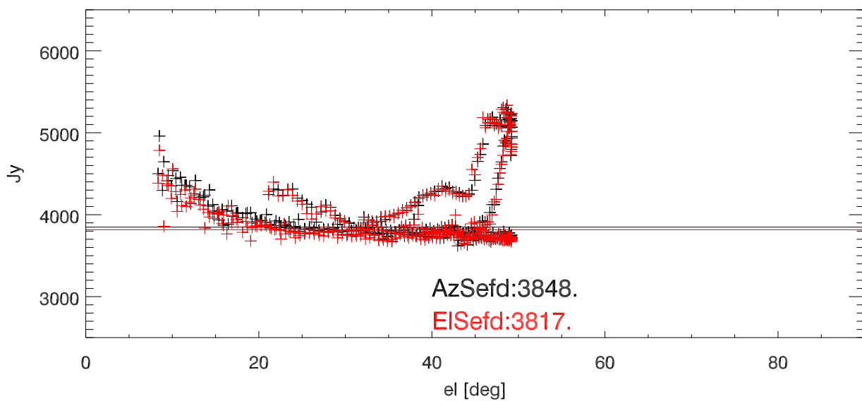
12m sband model3A 1d fits. SEFD from src: 3C461
