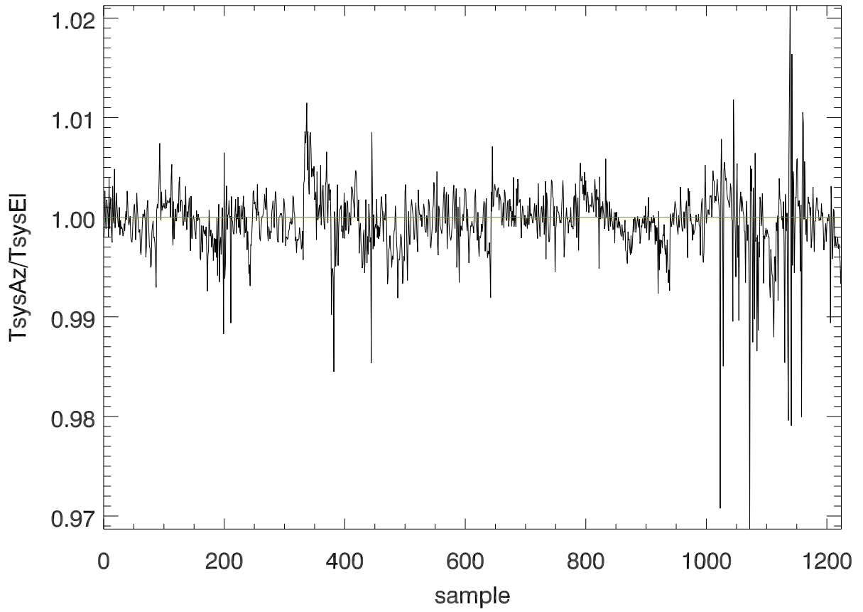
Ratio TsysAz/TsysEI strips
