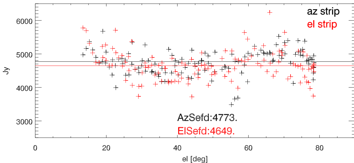
12m sband model3A 1d fits. SEFD from src: 3C123
