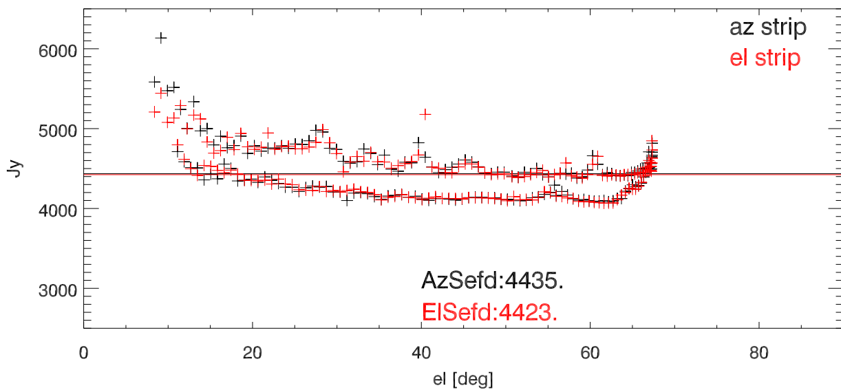
12m sband model3A 1d fits. SEFD from src: 3C405
