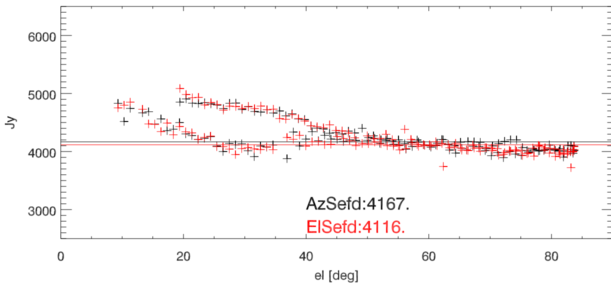
12m sband model3A 1d fits. SEFD from src: 3C274
