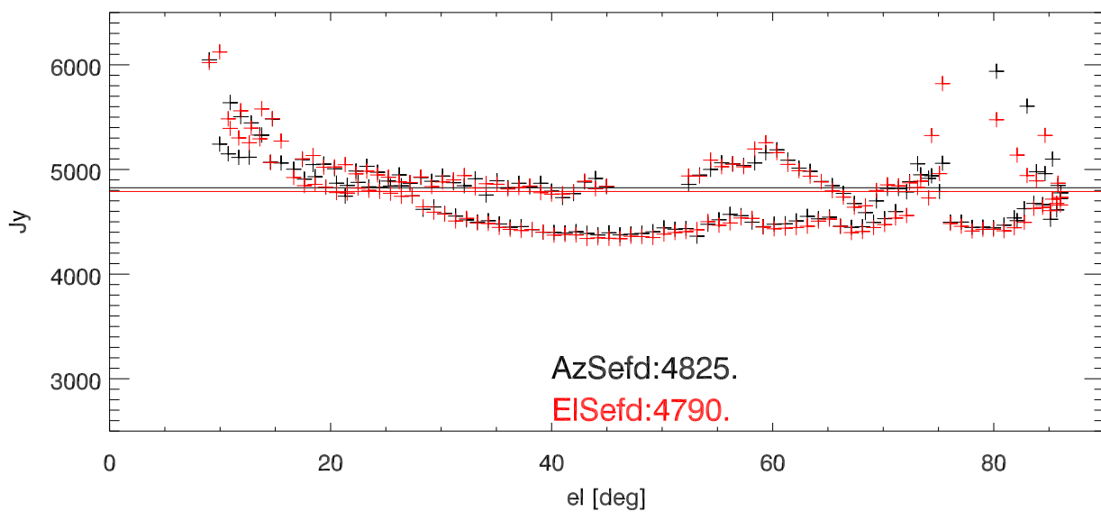
12m sband model3A 1d fits. SEFD from src: 3C144
