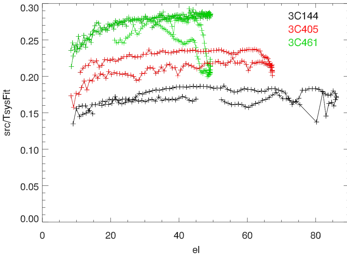
Tsource/ Tsys fit by src
