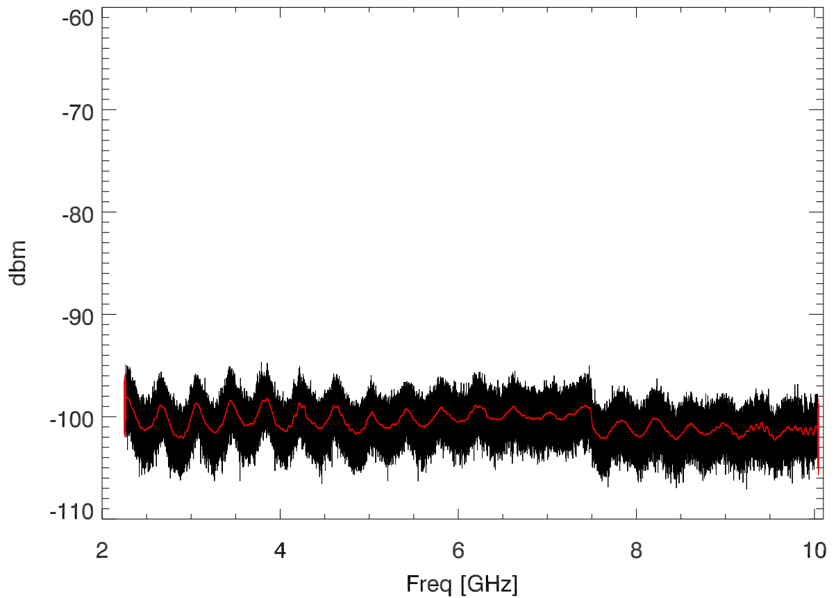
28mar23 dwMon spectra at fieldFox input. Box closed
