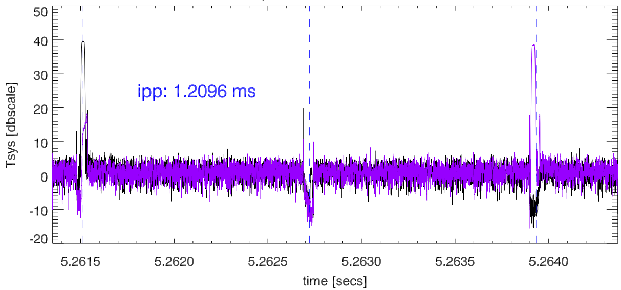
Blowup in time. 1usec resolution
