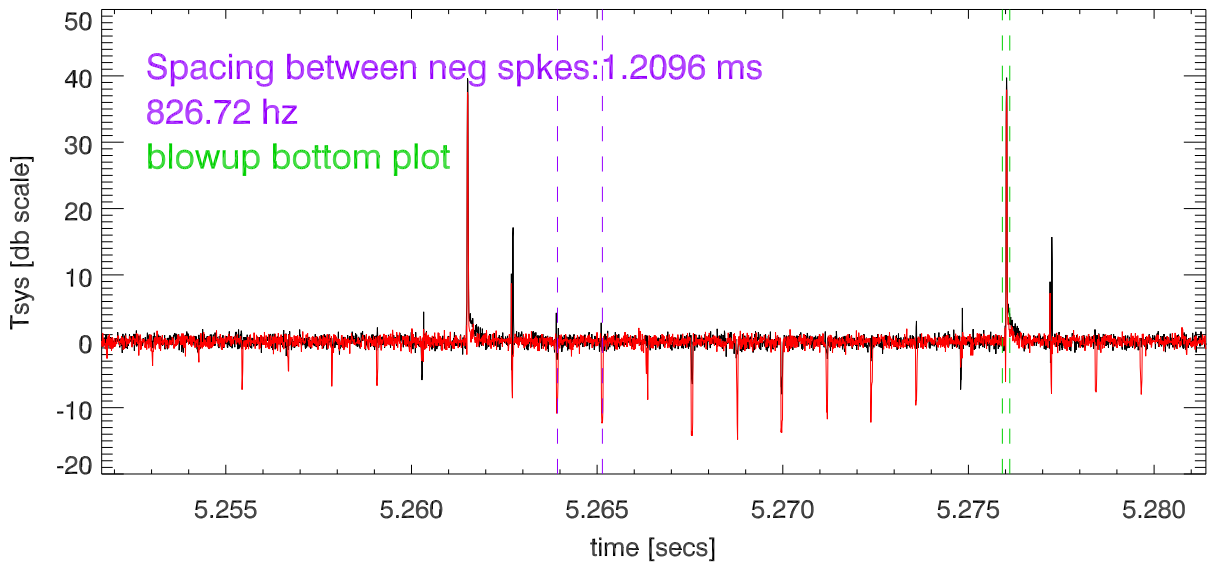
22feb23 totPwr vs time. 5.4 Mhz about 8762Mhz. 10Usec tmRes
