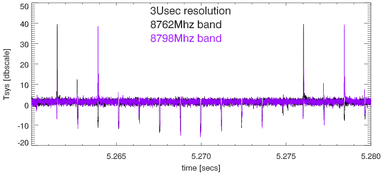
22feb23 totPwr vs time 8762 and 8798 Mhz Bands. PoIB
