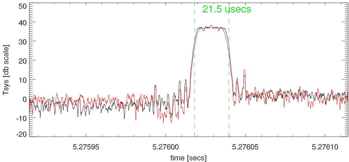
Blowup around peak. 1usec resolution
