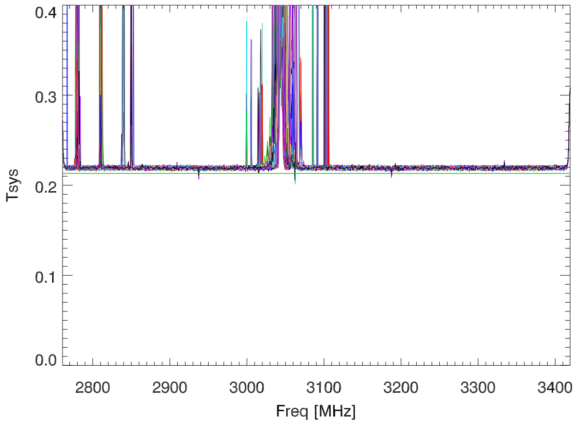
21jun23 rms/mean by freqChan for J0437-4715 (blowup) PoIB
