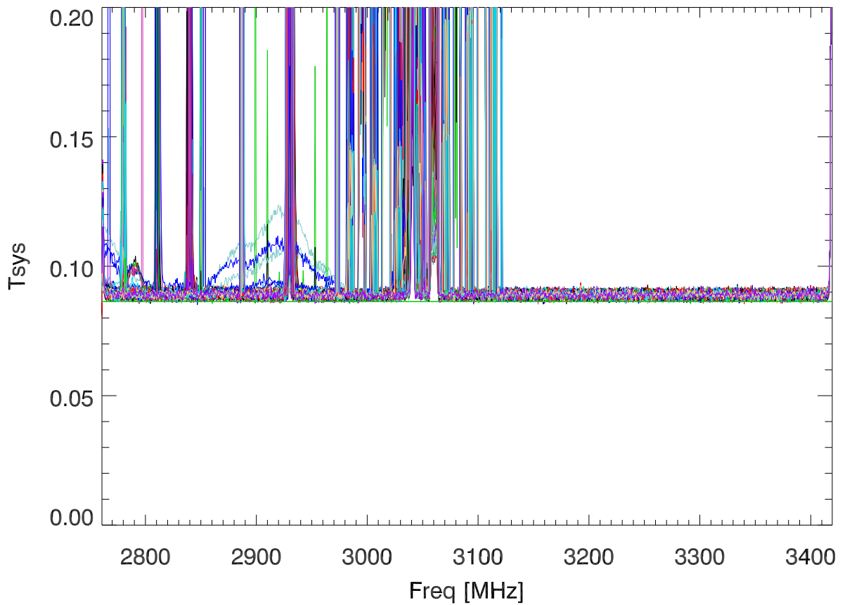
230615 rms/mean by freqChan for B0329+58 (blowup) PoIB
