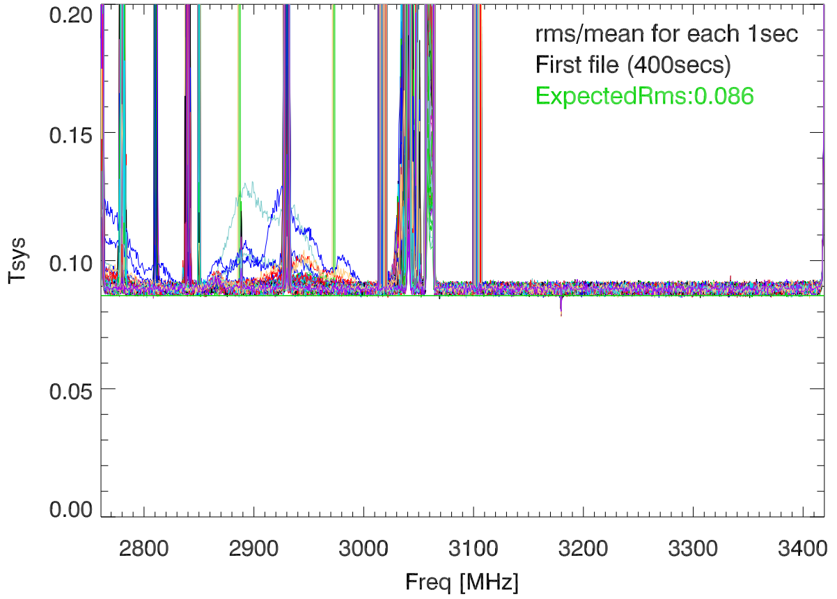
230615 rms/mean by freqChan for B0329+58 (blowup) PoIA
