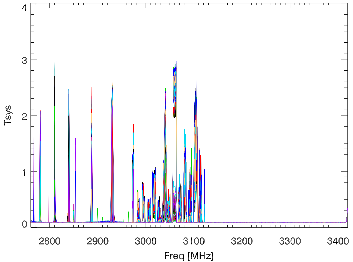
230615 rms/mean by freqChan for B0329+58PoIB
