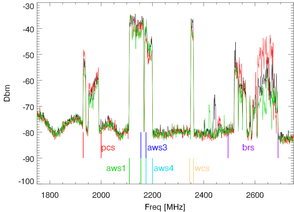
PoIB: Peak hold (30secs)
