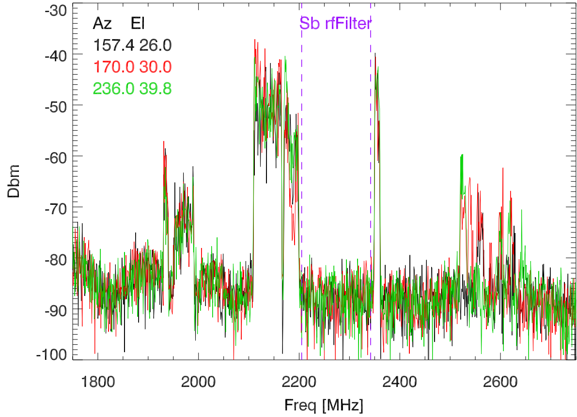
221021: p12m sband spectra before postamps. PoIB: Sample
