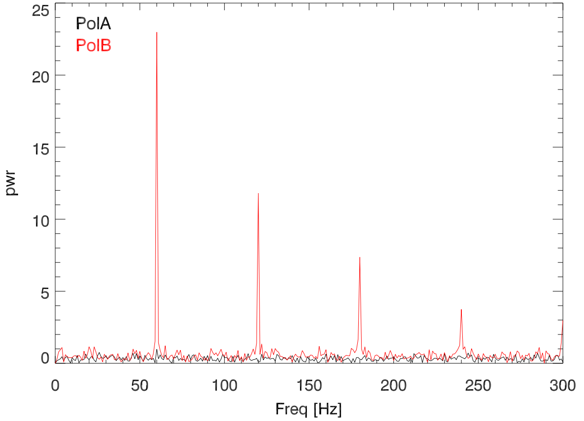
magnitude spectra of total power: 2292.8-2296.3 MHz
