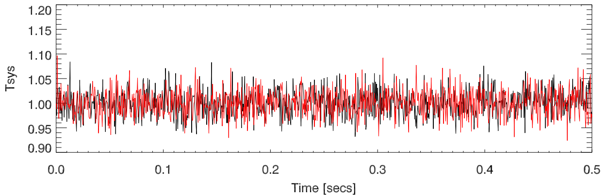
total pwr vs time. 2220.-2223.4 MHz
