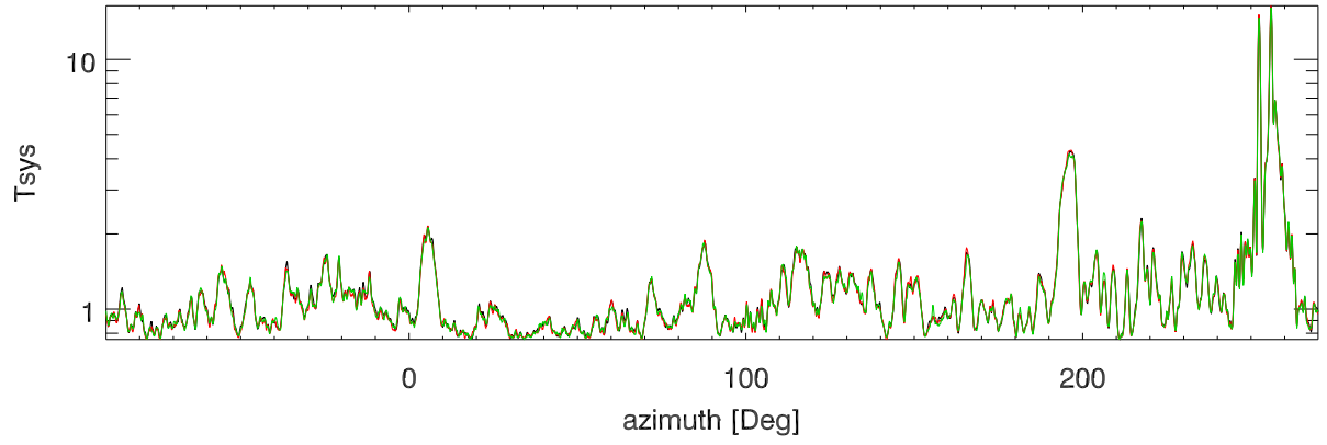
22mar22 totPwr vs az for various birdies: freq:2342.95 to 2344.82
