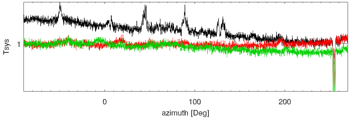
22mar22 totPwr vs az for various birdies: freq:2267.18 to 2268.90
