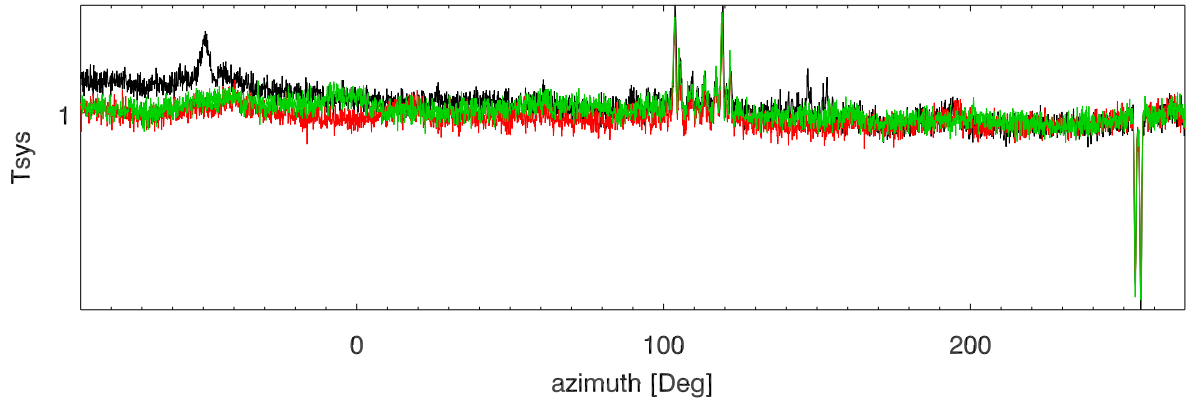
22mar22 totPwr vs az for various birdies: freq:2240.15 to 2241.24
