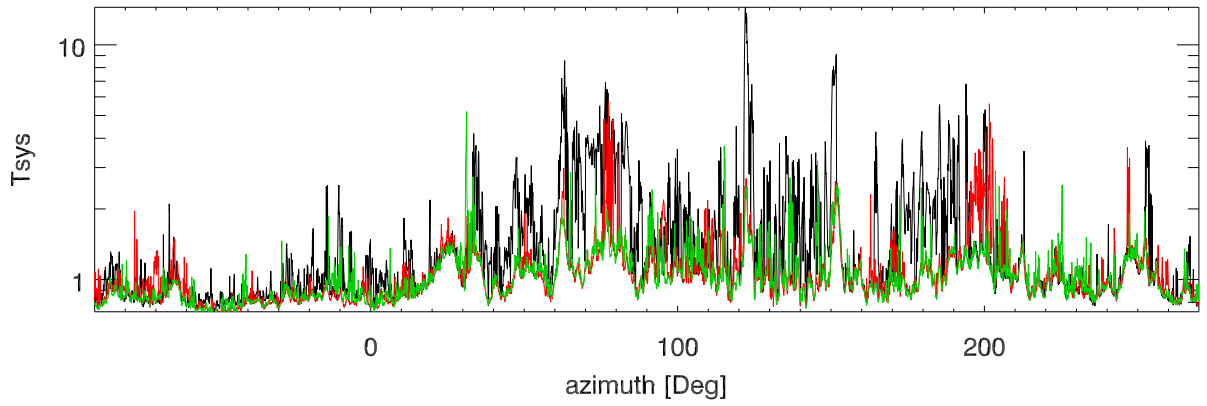
22mar22 totPwr vs az for various birdies: freq:2192.97 to 2199.06
