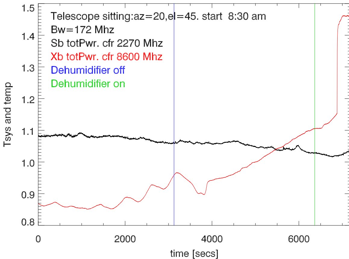
05mar16 12meter sb,xb total pwr vs time. Dehumidifier on,off
