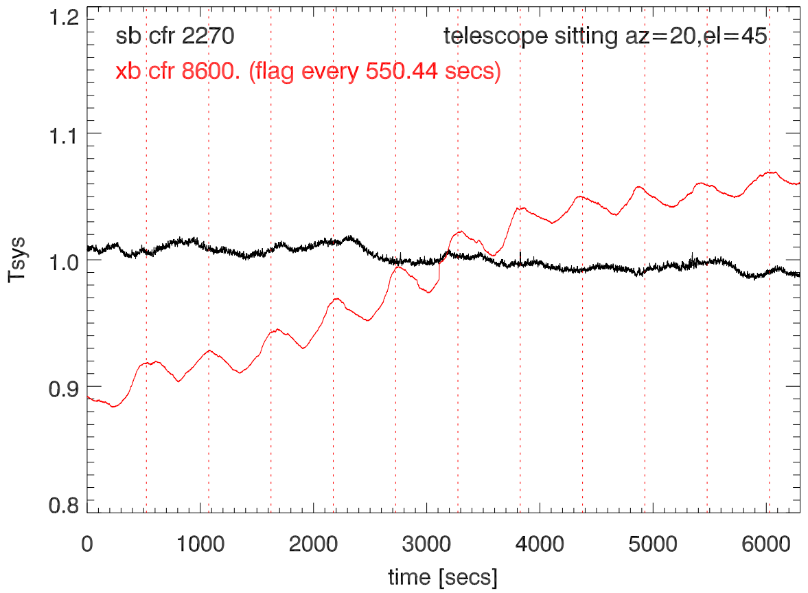
01mar16 12Meter: total power vs time sb,xb (bw=172Mhz)
